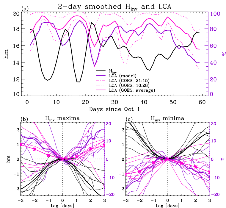
Fig. 10. (a): UKMO model-simulated inversion height (full black line) and low-cloud cover averaged over the region 90^{\circ} W– 80^{\circ} W, 15^{\circ} S– 25^{\circ} S. Both model-derived and satellite-derived (GOES-10) low-cloud cover are shown, in violet and magenta colours, respectively. The thin broken lines show the satellite-derived daily minima and maxima. (b) and (c): composites of inversion height and cloud cover in the region 90^{\circ} W– 80^{\circ} W, 15^{\circ} S– 25^{\circ} S based on the extrema of the daily-average MBL depth averaged over 90^{\circ} W– 80^{\circ} W, 19.5^{\circ} S– 20.5^{\circ} S.
