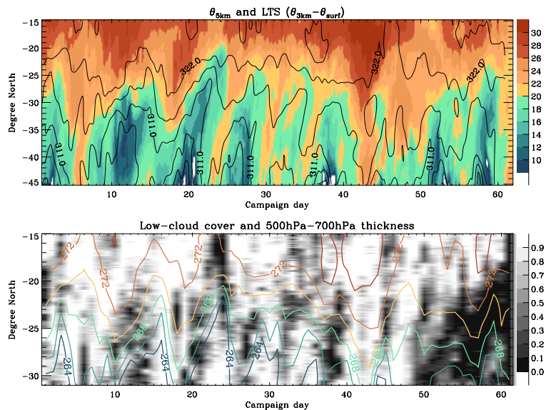
Fig. 8. (a) Lower tropospheric stability ( \theta_{700} - \theta_{\text{surf}} ) averaged over 80\text{--}85^\circ\text{W} , as a function of time and latitude; (b) as (a) but for cloud fraction from GOES at 19:30 UTC (late afternoon), and 500–700 hPa thickness contours. Thickness and temperature data from UKMO global operational analysis and 3 h–21 h forecasts.
