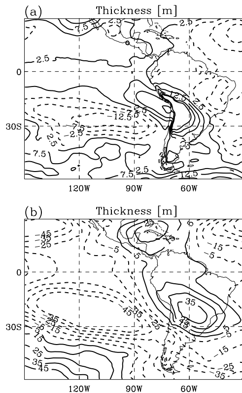
Fig. 2. Zonally asymmetric components of the 500 hPa–700 hPa and 200 hPa–500 hPa geopotential thickness fields (panels (a) and (b), respectively) in the eastern-Pacific/south-American sector. Shown are the time-means for the period between 1 October 2008 and 30 November 2008. Positive values are shown by the solid contours, negative values by broken contours. In panel (a), the contour interval is 5 m; in panel (b), it is 10 m. Data from UKMO operational analysis.
