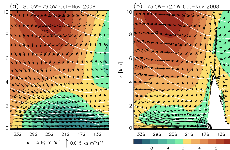
Fig. 3. Meridional transects of mean winds and isoentropes during October–November 2008. Winds are multiplied by density to give mass fluxes. Colour-coding shows zonal wind-speed, with contour interval of 2 \text{ kg m}^{-2} \text{ s}^{-2} ; white lines are contours for the dry potential temperature, with a spacing of 5 K. Vector scales for the meridional and the vertical winds are given on the bottom-right. Left: section along 80 W. Right: section along 73 W. Means from 3-hourly UKMO operational analysis and 3 h–21 h forecasts are used.
