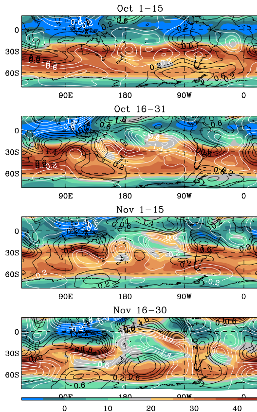
Fig. 16. Zonal wind at 200 hPa, in units of m/s, for four fortnight periods in October and November 2008 (colour coding, scale at the bottom). Contour lines show the zonally asymmetric component of the 200 hPa streamfunction. Contour interval is 4 \times 10^6 \text{ m}^2/\text{s} ; white contours indicate negative values (clockwise, or cyclonic, circulation in the Southern Hemisphere), and black positive values (anticlockwise, or anticyclonic, circulation). Data from UKMO operational analyses.
