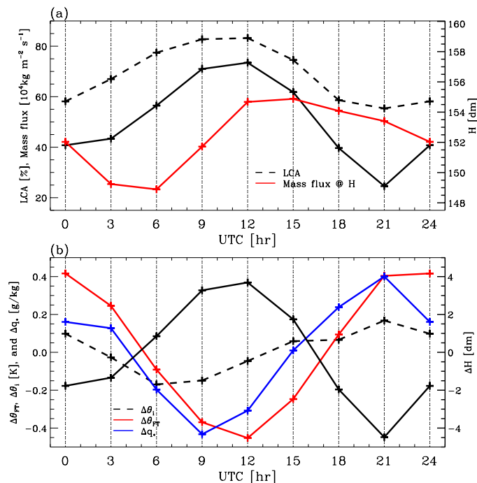
Fig. 20. Mean diurnal evolution of thermodynamic quantities near the inversion in the area 15^\circ \text{S} – 25^\circ \text{S} , 90^\circ \text{W} – 80^\circ \text{W} . (a) Inversion height (solid black line), cloud amount (broken line), and diagnosed mass entrainment across the inversion (red line) as a function of time of the day. (b) Inversion height anomalies (solid line) together with the lower-tropospheric ( z = 2200 \text{ m} ) potential temperature (red line), the MBL-top potential temperature (broken line), and the MBL-top saturation mixing ratio (blue line) as a function of the time of the day. Data from the UKMO operational analyses and 3 h–21 h forecasts.
