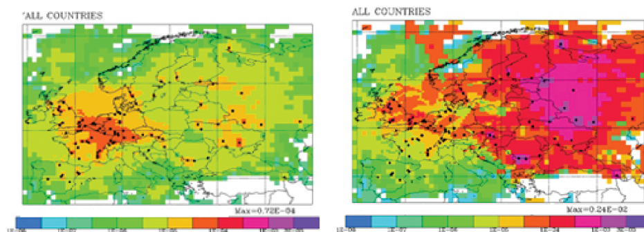
Nuclear risk maps from the Riskmap website; left with the IAEA scenario and right with the RT scenario.
