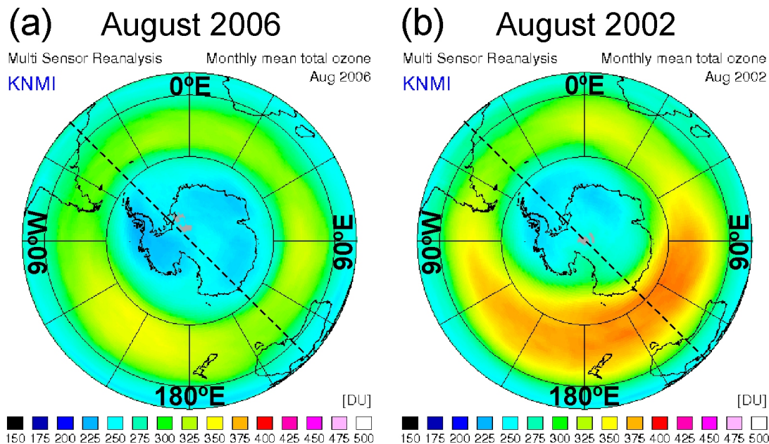
Fig. 1. A1. Total ozone fields from Multi Sensor Reanalysis data for (a) strong and zonally symmetric vortex in August 2006 and (b) weak and zonally asymmetric vortex in August 2002.
