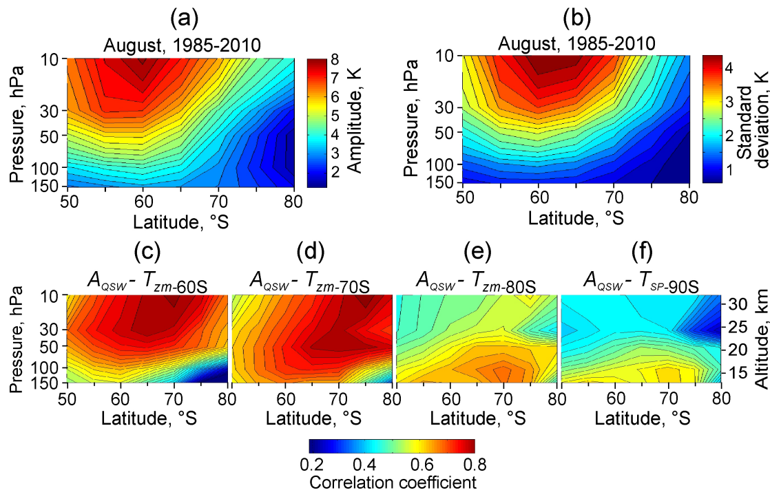
Fig. 2. Climatology of (a) August QSW amplitudes and (b) amplitude SD in stratosphere temperature. (c–f) Correlation QSW amplitude and zonal mean stratospheric temperature (vertically averaged) in August.
