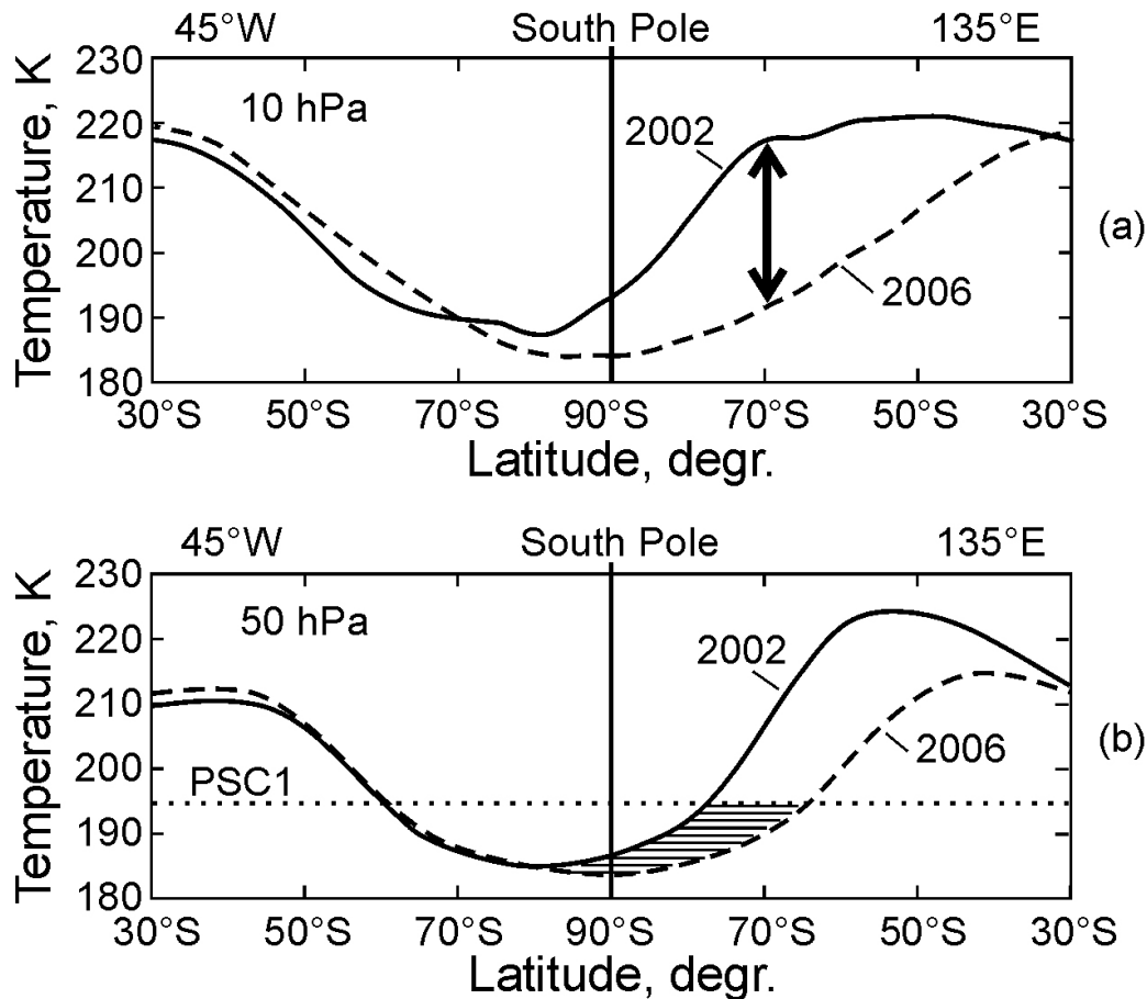
Fig. 3. A2. Stratospheric temperature profiles in the meridional plane 45° W–135° E at the pressure levels of (a) 10 hPa and (b) 50 hPa for August 2002 and August 2006 (solid and dashed curves, respectively).
