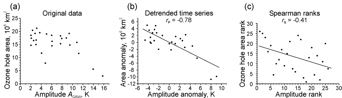
Fig. 1. A1. Variations of the ozone hole area in October and the QSW amplitude in August at 70^\circ \text{ S} , 10 hPa, during 1985–2010: (a) original data, (b) detrended anomalies and (c) Spearman ranks.
