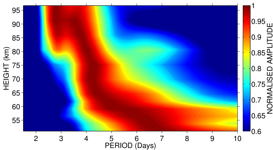
Fig. 2. Period vs Height of annually-averaged E1 wave amplitudes obtained by least squares fits on the satellite temperatures. Each amplitude within a height gate is normalised to that height's maximum.
