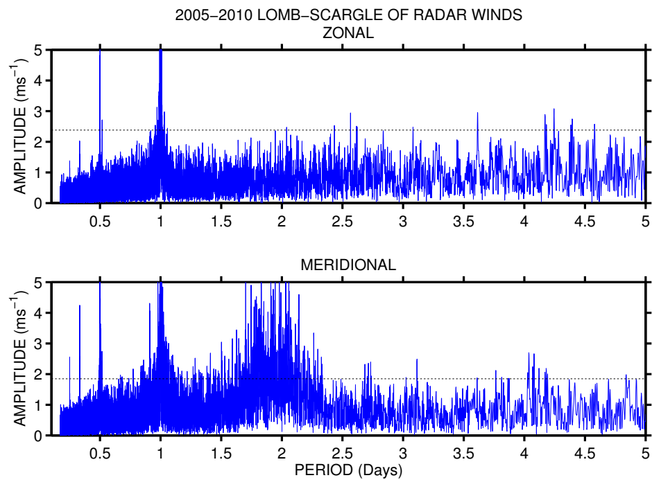
Fig. 4. Lomb-Scargle periodogram of all six years (2005 - 2010) of zonal and meridional radar winds. The horizontal dashed lines represent the 95% confidence limit.
