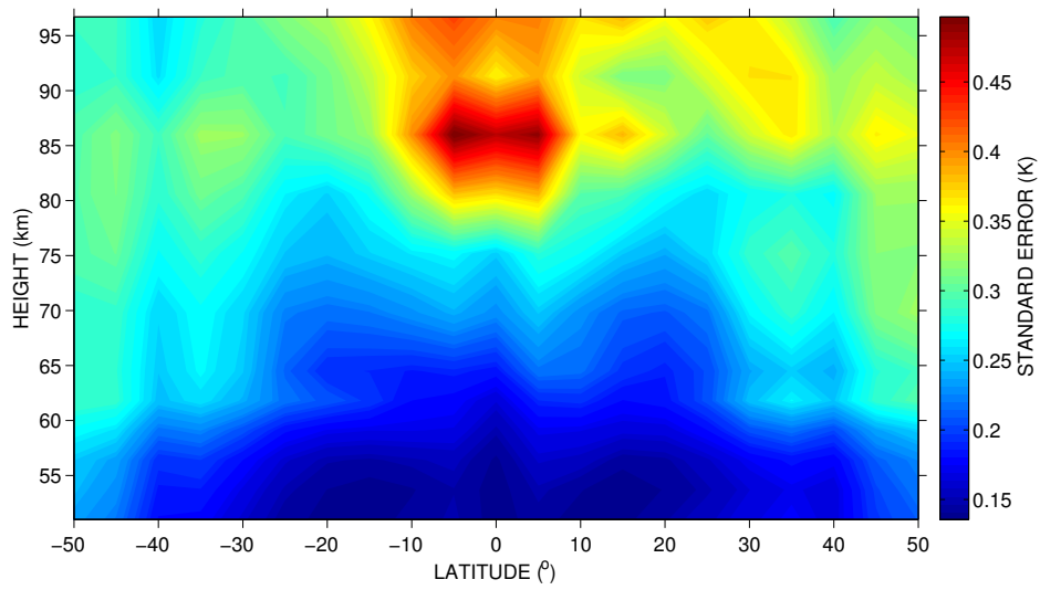
Fig. 3. Standard error on E1 wave amplitudes least squares fitted to Aura MLS temperatures, averaged over six years of data (2005-2010).
