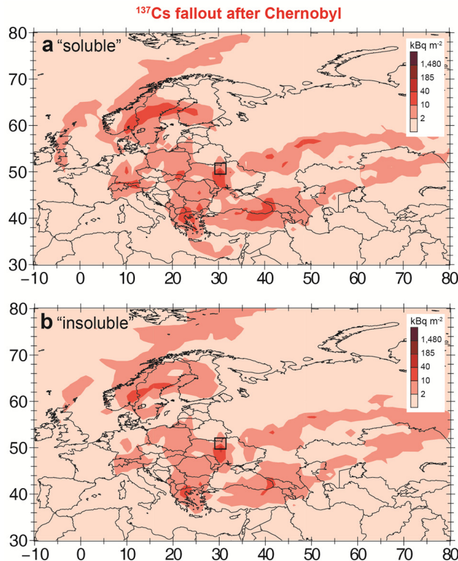
Fig. 1. Model calculated fallout of 137 Cs after the Chernobyl accident, assuming a soluble particle tracer (a) and an insoluble one (b) . The location of Chernobyl is indicated by the black square. The colour scale is the same as in Peplow (2006).
