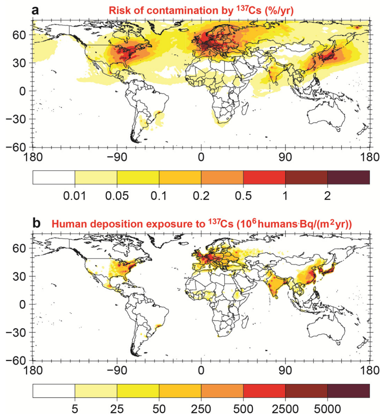
Fig. 2. Global risk of radioactive contamination by ^{137}\text{Cs} . (a) Modelled deposition of \geq 40 \text{ kBq } ^{137}\text{Cs/m}^2 \text{ yr}^{-1} . The risk is the expected value normalized by 40 \text{ kBq m}^{-2} . (b) Modelled risk of human exposure to ^{137}\text{Cs} deposition.
