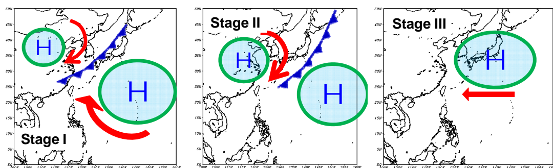
Figure A1: Schematic of the relationship between the movement of continental highs and associated wind direction around Taiwan. Stage I: Taiwan is covered in a warm air while a front is approaching. Stage II: continental cold air outflow after frontal passage. Stage III: the outflow rebound by the high pressure
