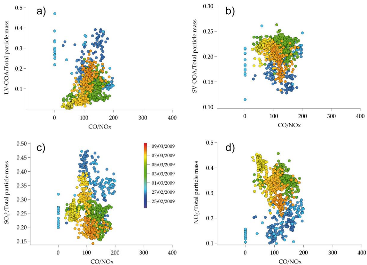
Figure S9 The fraction of a) LV-OOA, b)SV-OOA, c)\chem{SO_4}, and d)\chem{NO_3} to the total aerosol mass against the measured CO/\chem{NO_X} for cloud-free periods during the winter campaign coloured by date.
