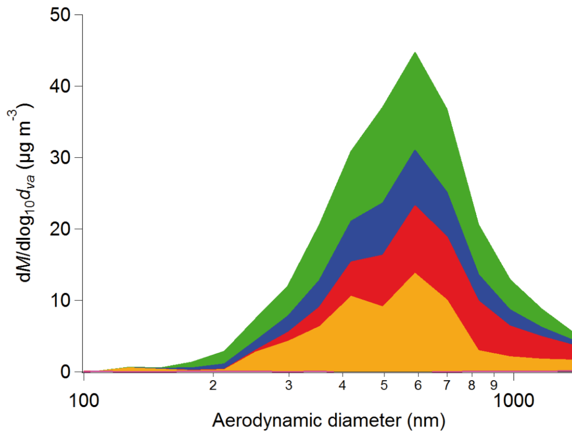
Figures S10. Typical size distribution of the aerosol particle species measured by the AMS at the pdD site.
