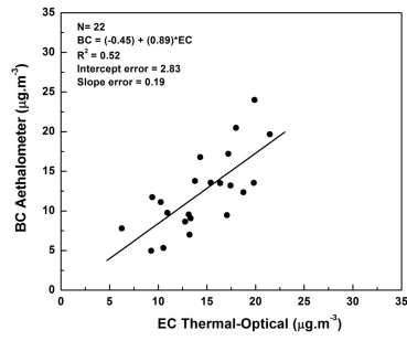
Figure 4: Comparison of BC measurements (from Aethalometer) and EC measurements (from thermal-optical analyzer) at village center (VC) located in Surya Village (SV1_1).
