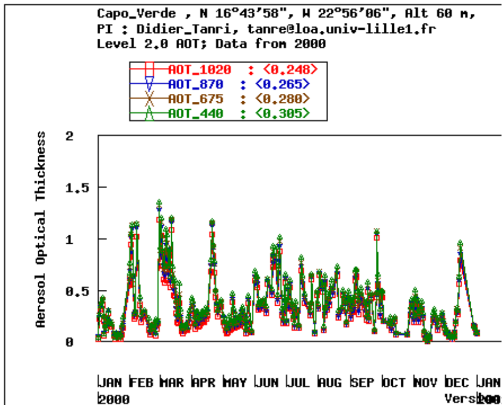
Fig. 1. Daily AOD at several wavelengths for year 2000 in Cape Verde.
