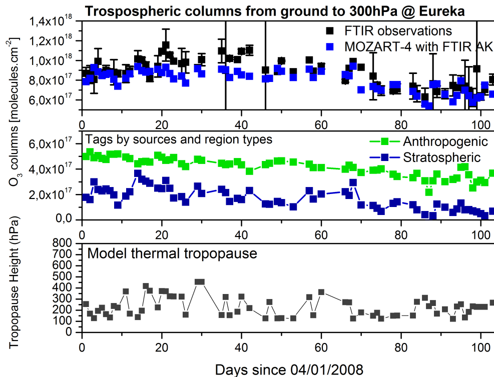
Fig. 1. Top: Daily mean O 3 tropospheric columns at Eureka. Middle: Anthropogenic and stratospheric contributions to O 3 tropospheric columns. Bottom: Model thermal tropopause height variation (hPa).
