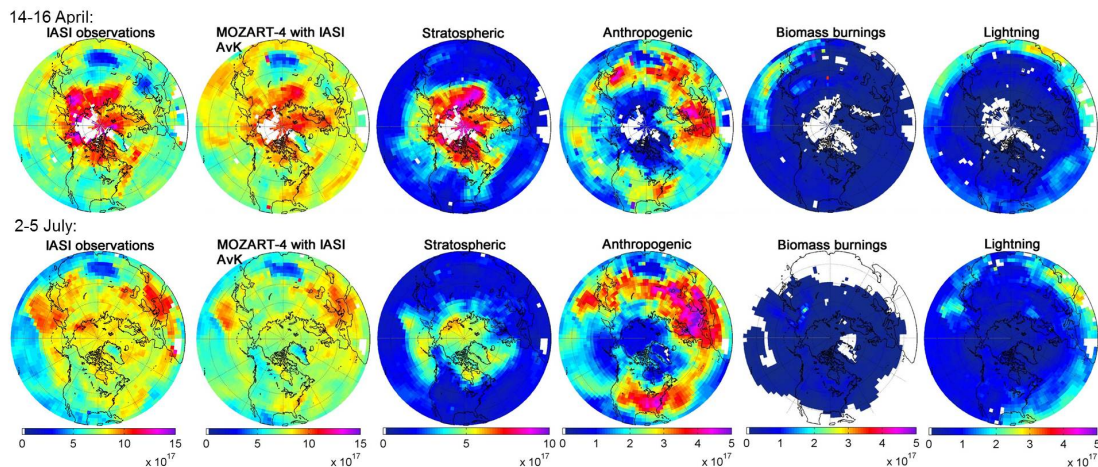
Fig. 2. Mean O 3 columns (molecules/cm 2 ) from ground-300hPa over 14-16 April and 2-5 July, observed by the IASI satellite and simulated by MOZART-4 smoothed with the averaging kernels of IASI observations.
