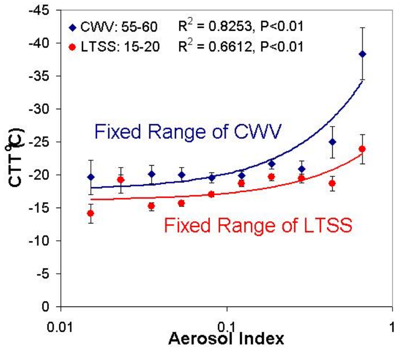
Fig. 2. Tests on the relation between cloud top temperature and AI using fixed range of CWV(55-60mm) and LTSS (15-20 degree Celsius)
