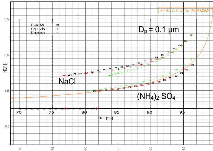
Figure 1: Copy of figure 3 from the paper under review (upper right panel), with an additional result (orange line) from the “kappa” parametrisation (PK2007), for \kappa=0.53 , (\text{NH}_4)_2\text{SO}_4 .
