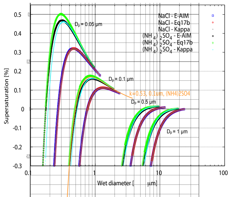
Figure 2: Copy of figure 5 from the paper under review (upper right panel), with an additional result (orange line) from the “kappa” parametrisation (PK2007), for \kappa=0.53 , (\text{NH}_4)_2\text{SO}_4 .
