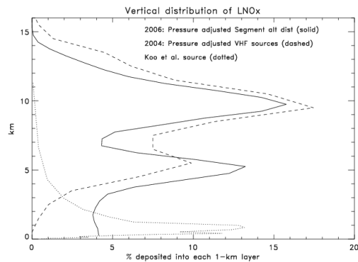
Figure 2. Vertical distribution of lightning-NO production assumed for CMAQ simulations by Allen et al. (2011) and Koo et al. (2010). The solid (dashed) black line shows the Allen et al. distribution for 2006 (2004). The dotted line shows the Koo et al. distribution.
