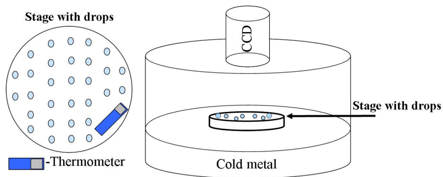
Fig. 2. Schematic diagram of the immersion freezing method.
