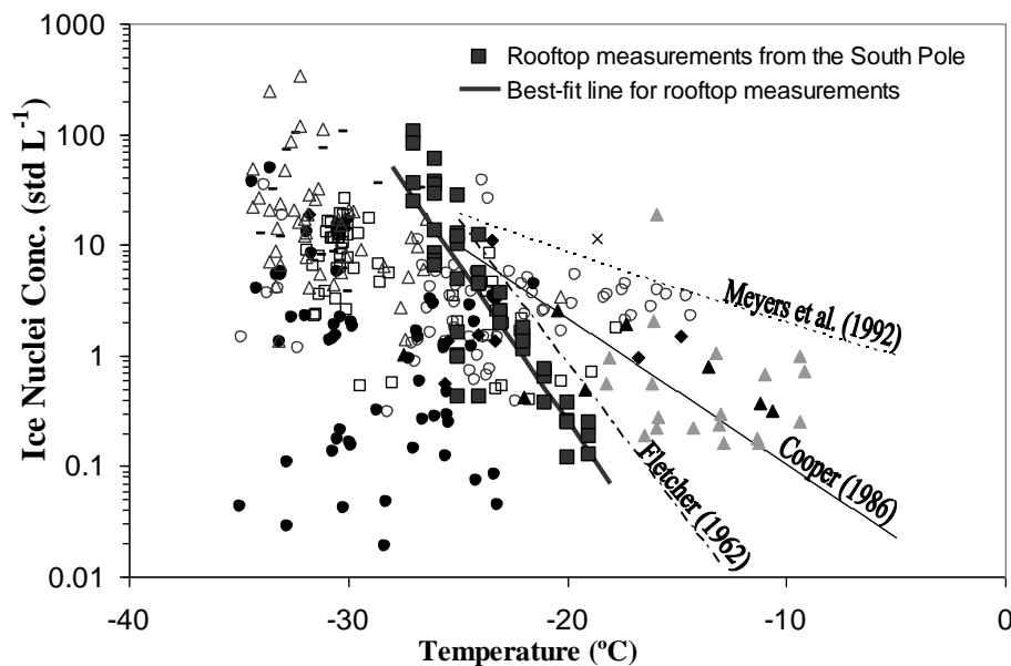
Fig. 11. Ice nuclei concentrations as a function of temperature from DeMott et al. (2010) with the present measurements shown in black squares.
