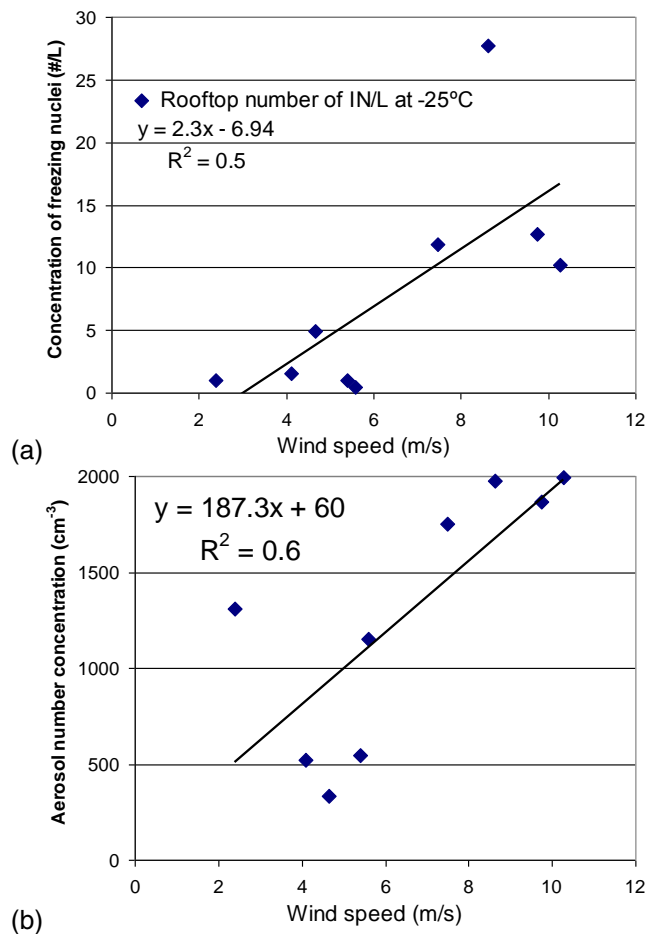
Fig. 7. (a) Concentration of freezing nuclei at -25^{\circ}\text{C} as a function of wind speed. (b) Concentration of aerosols >0.01\ \mu\text{m} as a function of wind speed.
