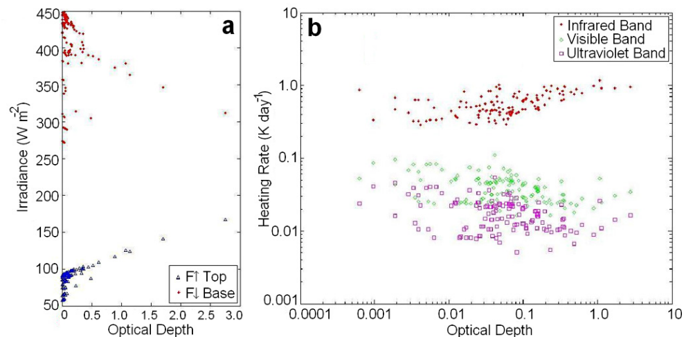
Fig. 4. (a) Broadband fluxes versus optical depths. Upward Flux at the cloud top ( F \uparrow Top) and downward Flux at the cloud base ( F \downarrow Base), for all studied clouds. (b) Daily Mean Heating rates for all studied cirrus clouds at each spectral solar band versus their optical depth.
