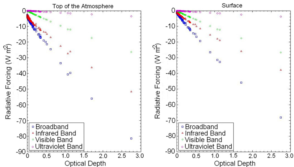
Fig. 5. Relation between daily mean value of SCRF, both for the broadband and the spectral bands of solar radiation, and the cirrus optical depths, for all dataset.
