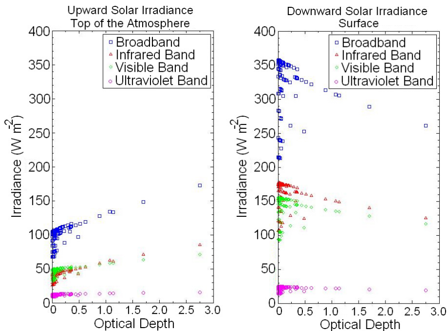
Fig. 3. Daily mean solar radiation flux in presence of cirrus clouds. Upward flux at TOA and downward flux at SFC, for the solar radiation broadband and spectral bands, versus cirrus optical depth for all cirrus measured with lidar in Camagüey.
