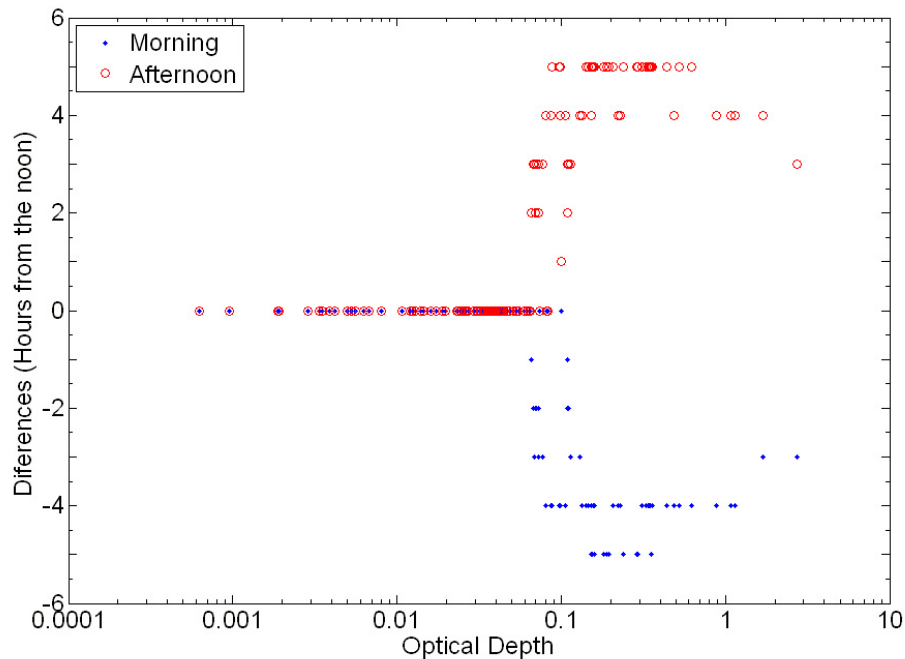
Fig. 2. Plot of the differences between hour of maximum SCRF and noontime (12:00 LT) versus optical depth, for the clouds measured with lidar in Camagüey. Threshold value is 0.083 for the occurrence of the maximum out of the noon.
