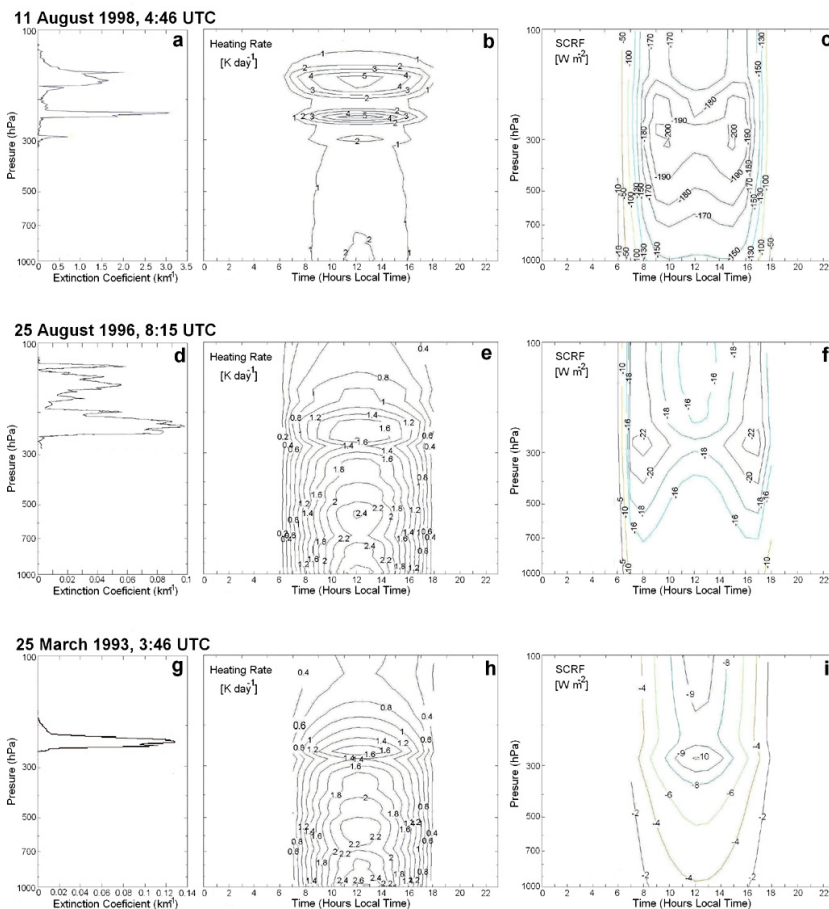
Fig. 1. Examples of cirrus clouds cases: extinction coefficient profiles, diurnal cycle of heating rate and SCRF. Top panel: opaque cirrus cloud; medium panel: thin cirrus cloud, bottom panel: subvisible cirrus cloud.
