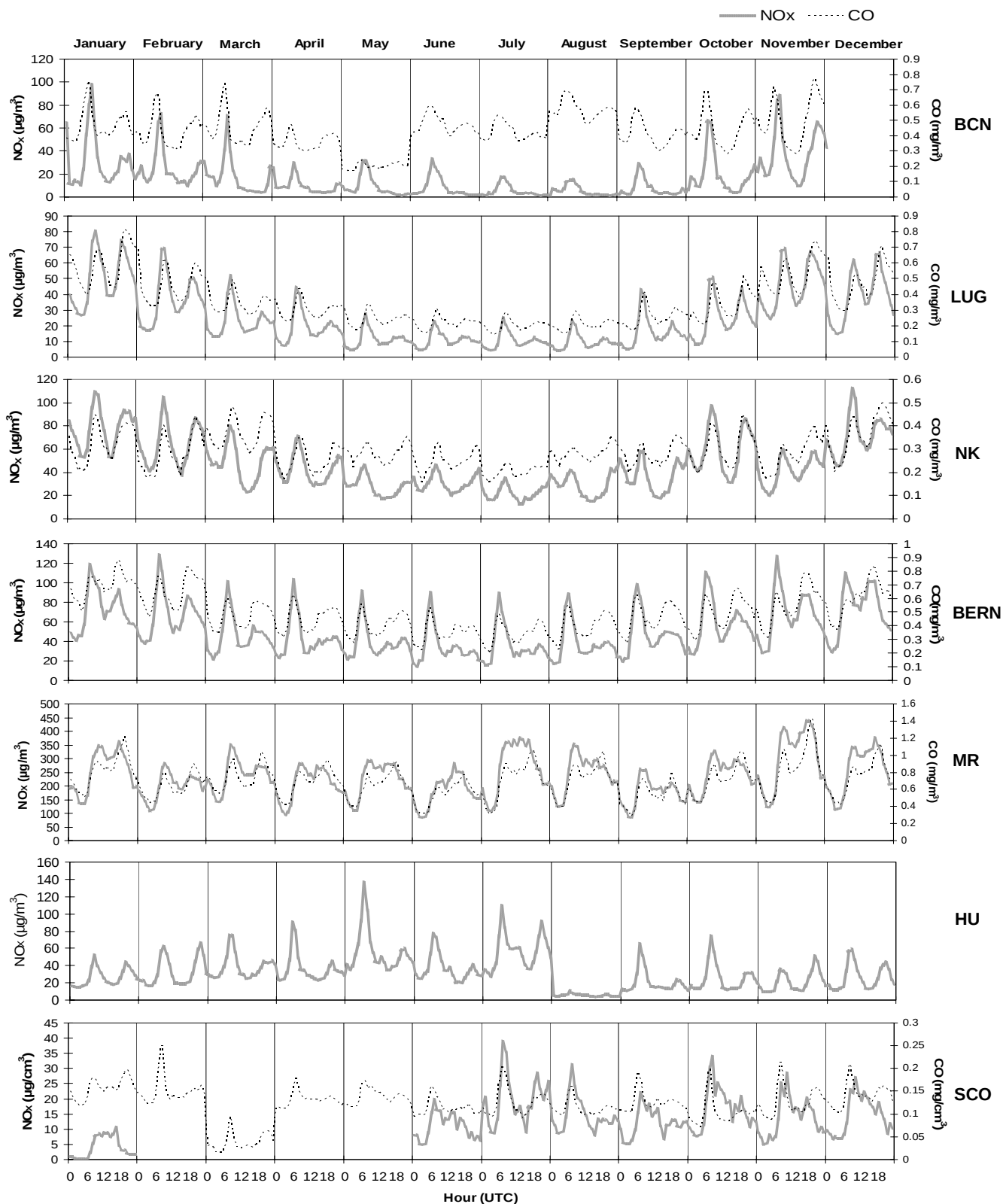
Figure S2. Daily cycle of NO x and CO for each month.
