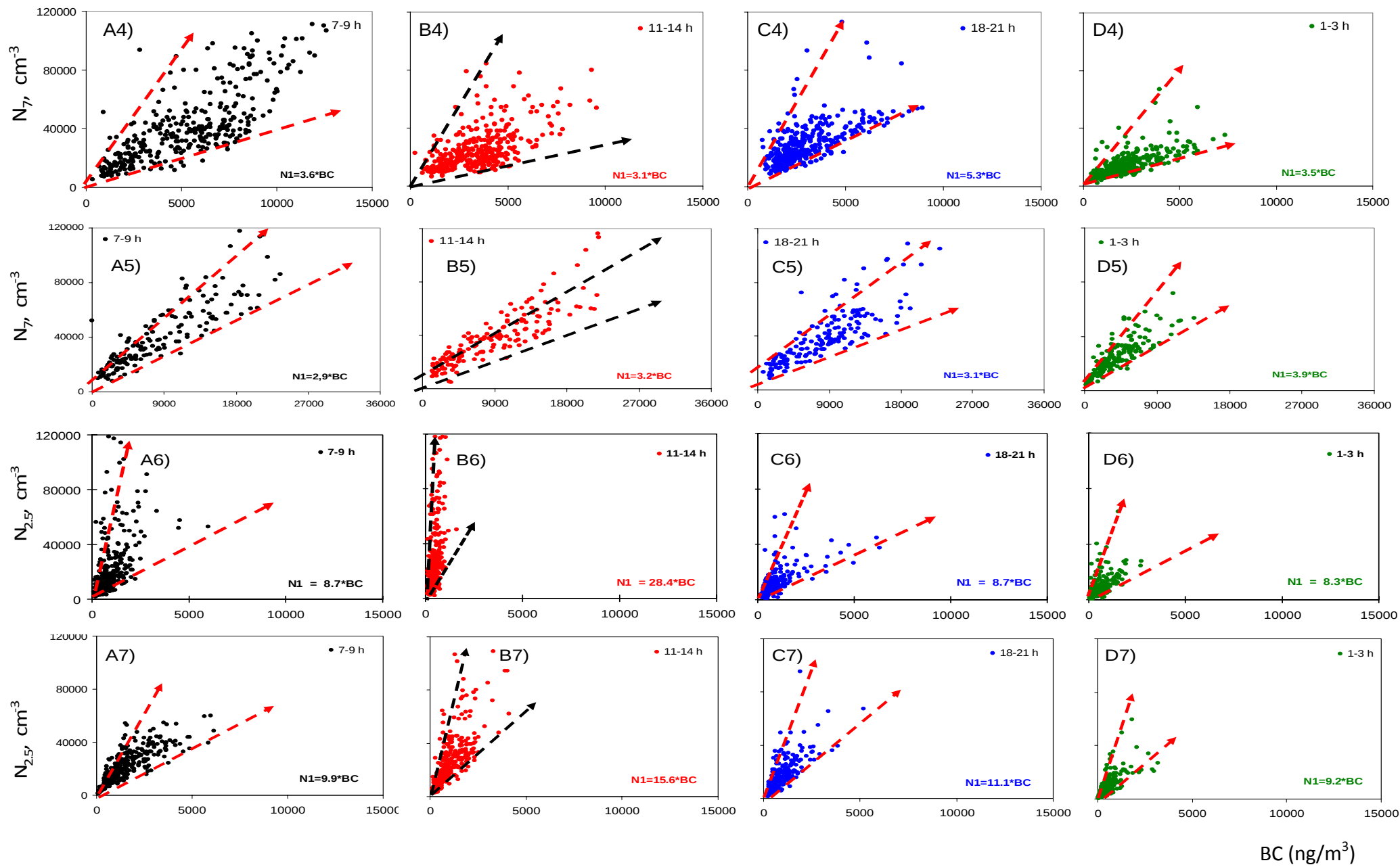
Figure S3. BC vs. N scatter plots for the different stations under study. 1:BCN; 2: LUG; 3: NK; 4: Bern; 5: MR; 6: HU; and 7: SCO.
