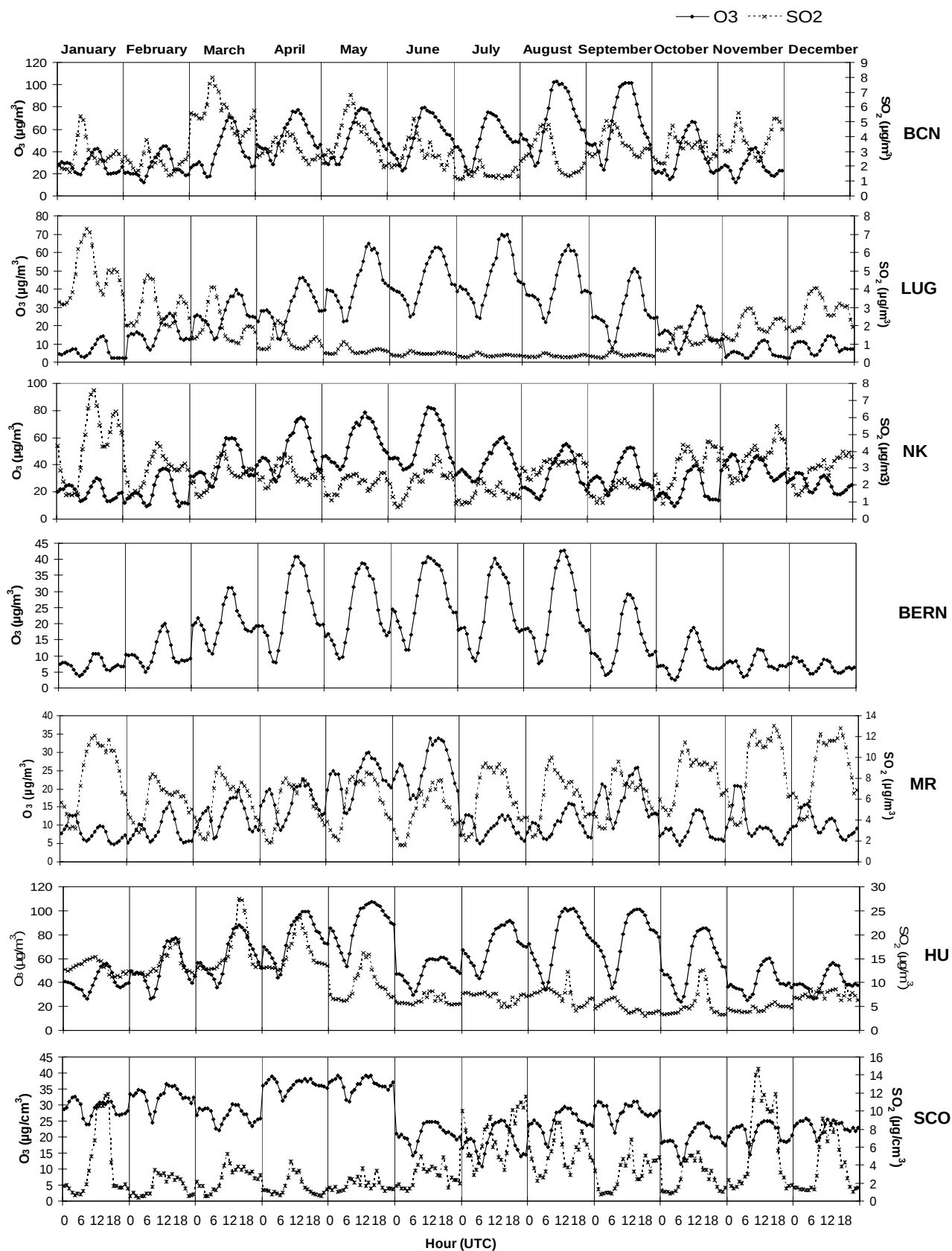
Figure S1. Daily cycle of SO 2 and O 3 for each month.
