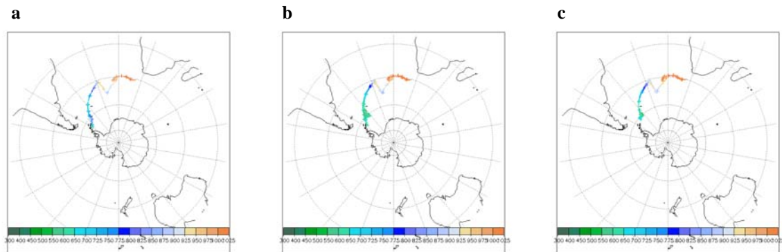
Figure S.8 Calculated back trajectories for March 16 th for the period of study. Plots a, b and c correspond to 6:00, 9:00 and 12:00 GMT respectively. The colour bar below each plot is an indication of the pressure level (300 to 1025hPa).
