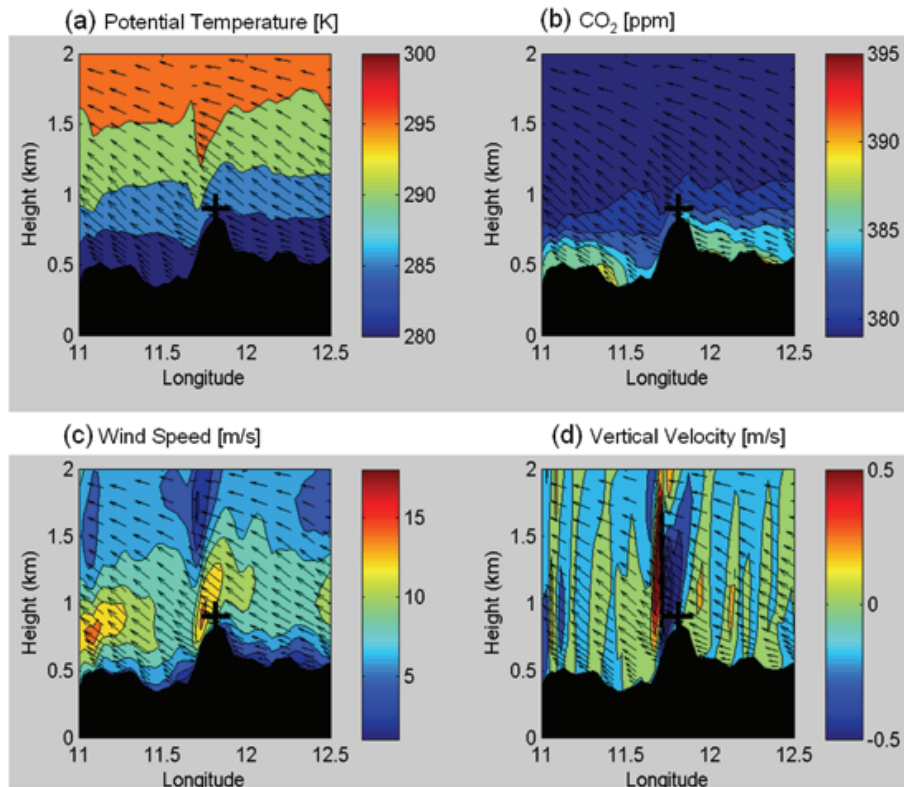
Fig. 12. Vertical cross section along OXK latitude ( 50^{\circ}01' \text{ N} ) on 17 October 2006 at 02:00 UTC, showing WRF-VPRM simulated (a) potential temperature in Kelvin, (b) \text{CO}_2 concentration in ppm, (c) wind speed in \text{m s}^{-1} , and (d) vertical velocity in \text{m s}^{-1} . The overlaid arrows indicate wind direction.
