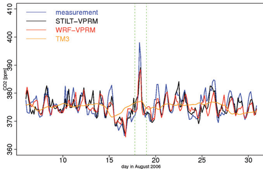
Fig. 6. Comparison of measured and modeled \text{CO}_2 concentrations for August 2006 at 90 m on the OXK. A period between dashed green vertical bars denotes a synoptic event during 00:00 to 15:00 UTC on 18 August 2006 (see also Sect. 4.1).
