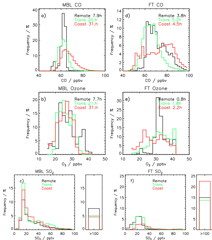
Fig. 5. All-aircraft carbon monoxide (top panels), ozone (centre panels) and sulphur dioxide (lower panels) concentration probability density functions gridded to longitudinal zones (colour-coded as indicated) along 20° S, in the MBL (left panels) and the FT (right panels). Total sampling time in hours is plotted in each panel for each zone. See text for further details.
