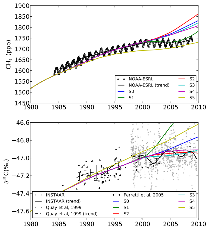
Fig. 3. Comparison between model results for the scenarios S0 to S5 and measurements at the station of Cape-Grim, Australia, for methane (top) and \delta^{13}\text{C}\text{-CH}_4 (bottom). Model results are shown as deseasonalized trends (2-yr smoothing). Error bars represent the uncertainty of the calculated trend (yearly RMSE divided by the number of measurements).
