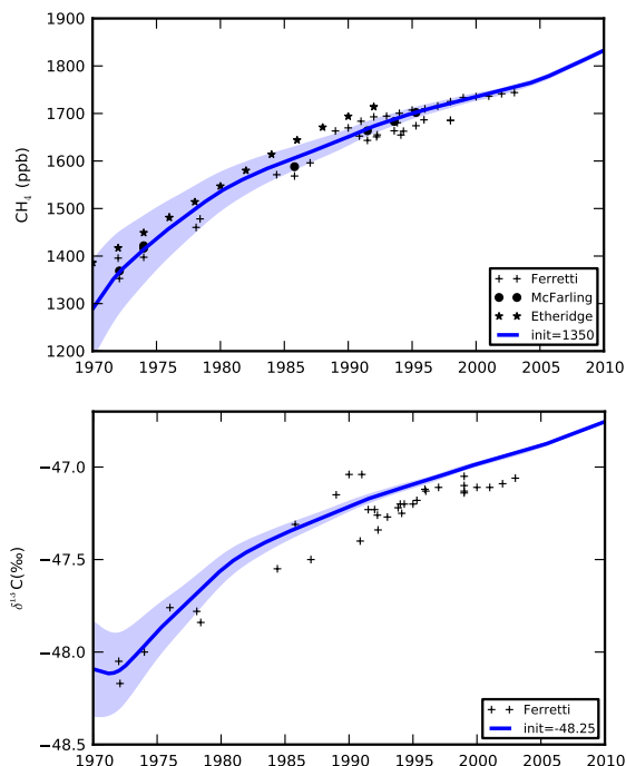
Fig. 1. Comparison between model base scenario and measurements from ice-cores and firn by Etheridge et al. (1998), Ferretti et al. (2005) and MacFarling Meure et al. (2006) for CH 4 and \delta^{13}\text{C}-\text{CH}_4 . Solid blue line corresponds to simulations using mean initial values of 1350 ppb for CH 4 and -48.25\% for \delta^{13}\text{C}-\text{CH}_4 . Shaded areas represent uncertainty ranges of \pm 100 ppb for methane and \pm 0.5\% for \delta^{13}\text{C}-\text{CH}_4 .
