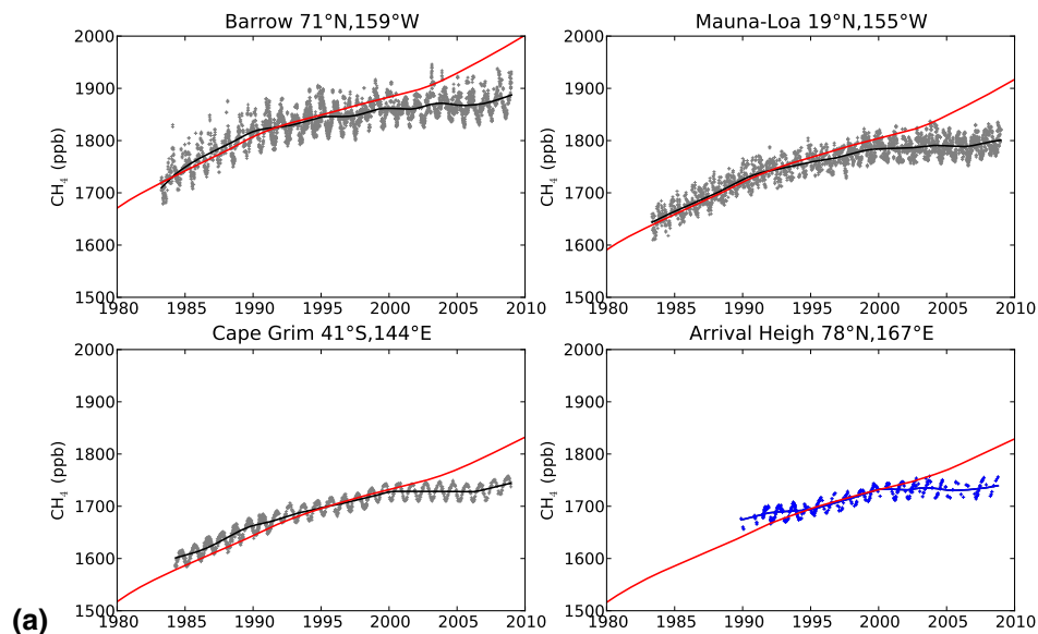
Fig. 2. Comparison between model scenario S0 and measurements for four representative stations, for \text{CH}_4 (a) and \delta^{13}\text{C}-\text{CH}_4 (b). Model results, shown as solid red lines, are deseasonalized. Measurements, shown as dots (real measurements) and as solid lines (deseasonalized trends), are from: grey: Dlugokencky et al. (2010) (NOAA); light blue: Francey et al. (1999); green: Quay et al. (1999); blue: Allan et al. (2005) (NIWA). Error bars in the trends lines for isotopes represents the yearly uncertainty of the trend.
