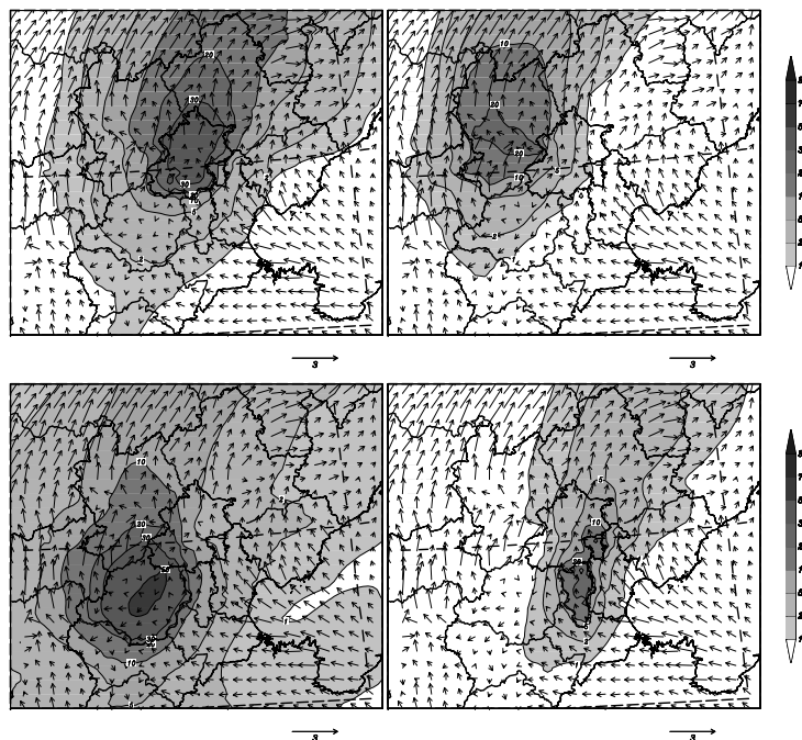
Fig. 13. Horizontal distribution of the percentage of Beijing local production and potential surrounding areas contributions to ozone monthly mean concentration over Beijing: up left: from BJ; up right: from ZJK; down left: BD; down right: LF. The unit of the wind vector is m/s.
