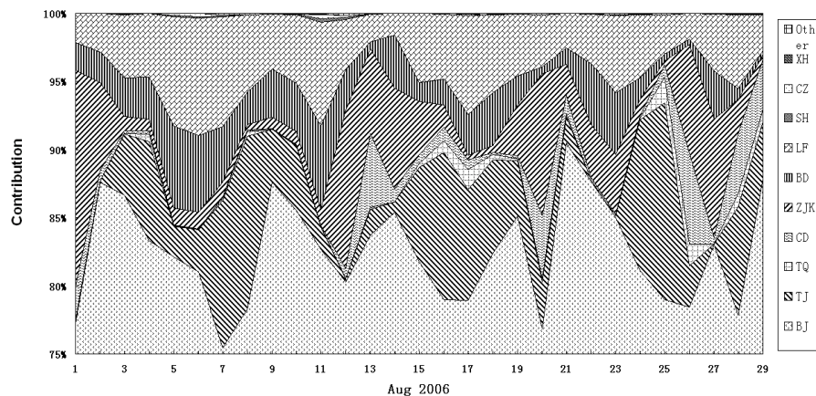
Fig. 9. Percentage of the contributions to the daily mean PM_{10} concentration in Beijing at the surface layer.
