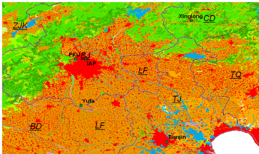
Fig. 2. The location of the observation stations (IAP, Yufa and Xinglong), red shaded is stand for urban area.
