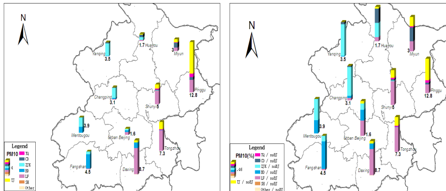
Fig. 10. Surrounding areas contribution to PM 10 monthly mean concentration ( \mu\text{g m}^{-3} ) over Beijing counties without Beijing local contribution (left) with its percentage (right).
