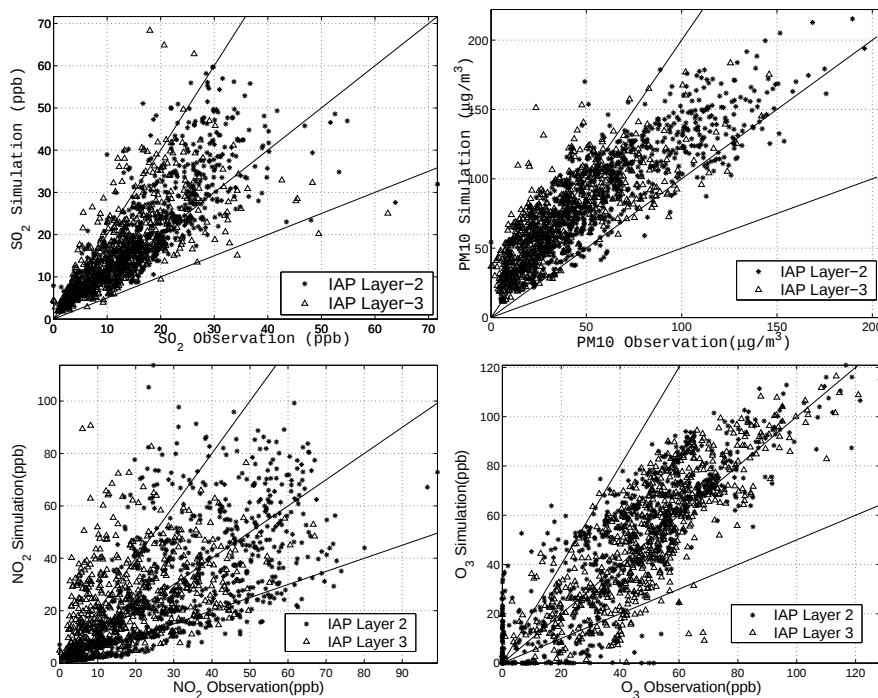
Fig. 3. The scatter plots of \text{SO}_2 , \text{PM}_{10} , \text{NO}_2 and \text{O}_3 at IAP tower station: three lines indicate y = 0.5x , y = x and y = 2x .
