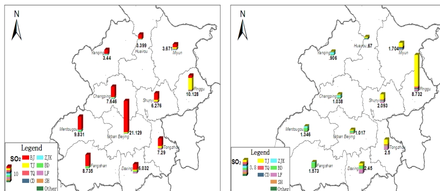
Fig. 7. The contribution to the SO 2 monthly mean concentration (ppbv) over Beijing counties, including Beijing local contribution (left) and without Beijing contribution (right).
