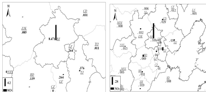
Fig. 11. The contribution to the \text{NO}_2 monthly mean concentration (ppbv) at surface layer (left), and at the upper layer (right), the grey bars indicate the contribution over Beijing.
