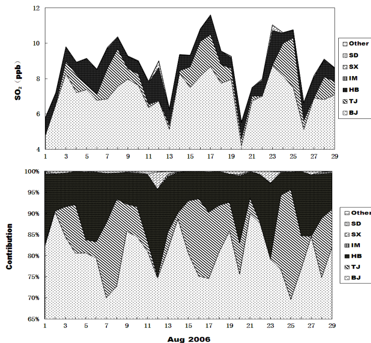
Fig. 5. Time series of the contributions to the daily mean \text{SO}_2 concentration (up) over Beijing at the surface layer and its percentage (down). Beijing (BJ); Tianjin (TJ); Hebei (HB); Inner Mongolia (IM); Shanxi (SX); Shandong (SD).
