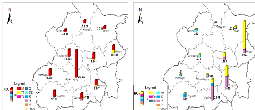
Fig. 12. Same as Fig. 7 but for \text{NO}_2 , concentration unit: ppbv.
