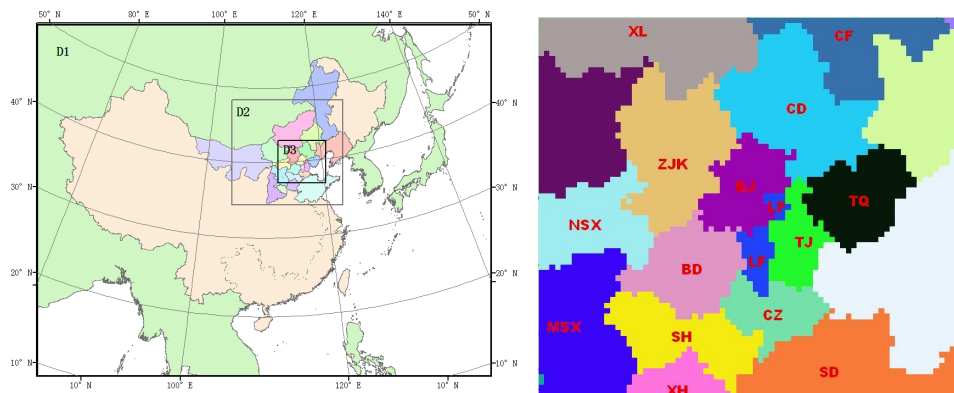
Fig. 1. The three nested domain used for simulation. Left: D1 covers East Asia with 83x65 grids; D2 with 61 \times 58 grids includes North China; D3 with 79x70 grids consists of Beijing and its surrounding cities. Right: source tagged regions: Beijing (BJ); Tianjin (TJ); Tangshan and Qinhuangdao (TQ); Chengde (CD); Zhangjiakou (ZJK); Baoding (BD); Langfang (LF); Shijiazhuang and Hengshui (SH); Cangzhou (CZ); Xingtai and Handan (XH); Xilinguole (XL); Chifeng (CF); Shandong (SD); Middle Shanxi (MSX); Northern Shanxi (NSX).
