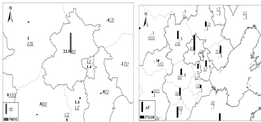
Fig. 8. The contribution to \text{PM}_{10} monthly mean concentration ( \mu\text{g m}^{-3} ) at the surface layer (left), and at the upper layer (right), the grey bars indicate the contribution over Beijing.
