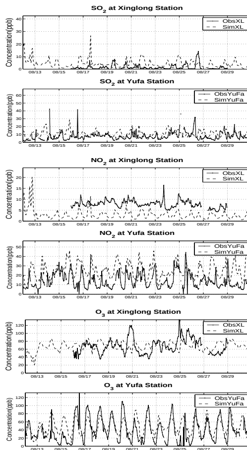
Fig. 4. Temporal variations of observed and simulated \text{SO}_2 , \text{NO}_2 and Ozone ( \text{O}_3 ) concentration at Xinglong and Yufa station in August 2006.
