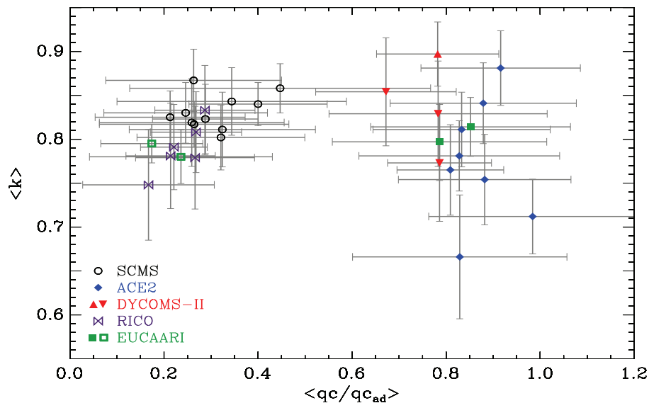
Fig. 4. Scatterplot of \langle k \rangle values as function of the LWC dilution ratio. For the LWC dilution ratio, the difference between the 80th and the 20th percentile of the frequency distribution is used as the error bar instead of the standard deviation to represent the variability.
