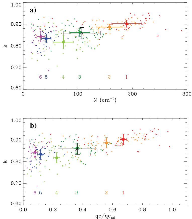
Fig. 3. Scatterplot of the 10Hz sample k factor values derived from Fast-FSSP data collected in a Cu during SCMS (points) as function of (a) the total droplet number concentration and (b) the LWC dilution ratio. Mean value is indicated for each of the six cloud traverses performed in this turret (colour dot) and for the whole data set (black triangle). Error bars correspond to one standard deviation.
