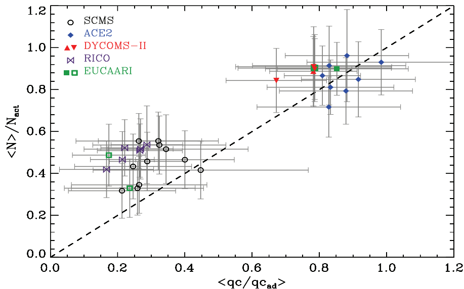
Fig. 8. Scatterplot of the CDNC dilution ratio as function of the LWC dilution ratio.
