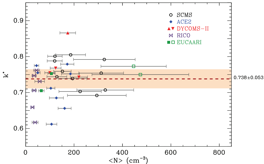
Fig. 7. Same as Fig. 6 for k^* values.
