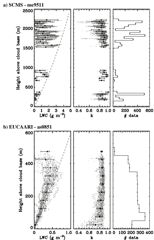
Fig. 5. Vertical profiles of LWC, the k factor and the number of data points in each 50 m altitude interval above cloud base. For LWC and the k factor, the mean value (black dot) and standard deviation (error bar) are superimposed to the data (grey points). The dashed line on the left panel corresponds to the adiabatic LWC profile.
