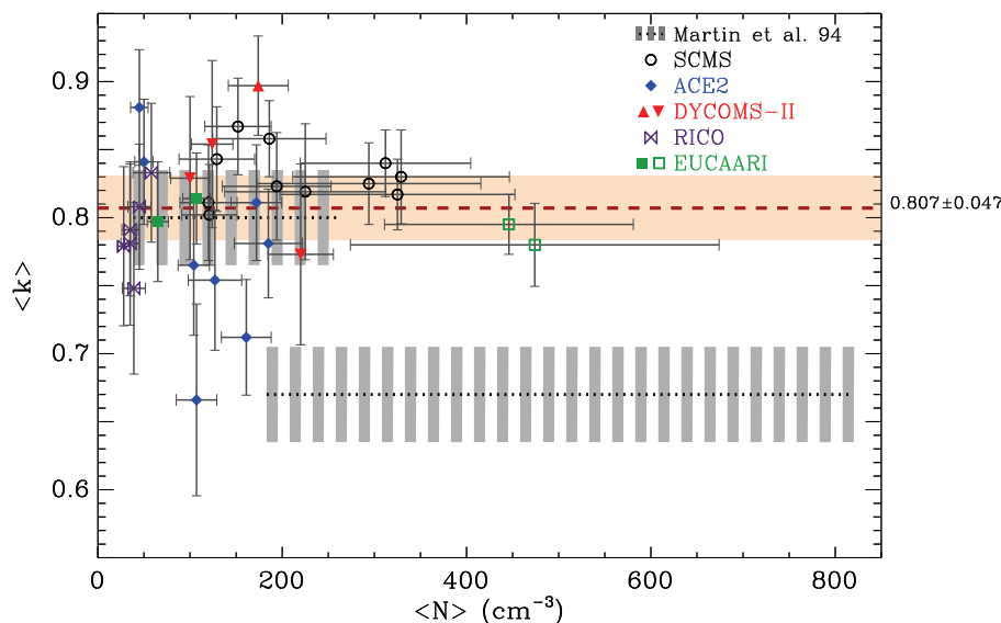
Fig. 6. Flight averaged k factor as function of mean total droplet number concentration for the 33 cases studies listed in Table 4. The error bar corresponds to one standard deviation. Symbols depend on the project as indicated in the legend with open and solid symbols for Cu and Sc clouds, respectively. For DYCOMS-II pointing up triangle is for Fast-FSSP data and pointing down triangles are for SPP-100 data. The average of all the cases is indicated with a dashed line and a light orange bar for the standard deviation. The two dotted lines with bars apart are the values recommended by Martin et al. (1994).
