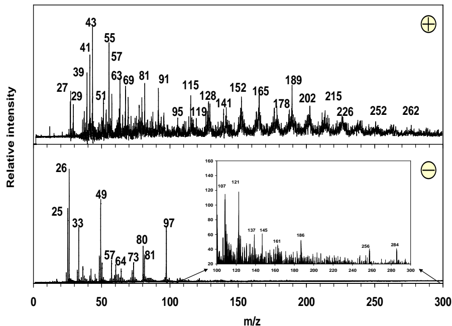
Fig. 2. Single particle positive and negative mass spectra of an individual particle belonging to ART-2a cluster SOA-PAH.
