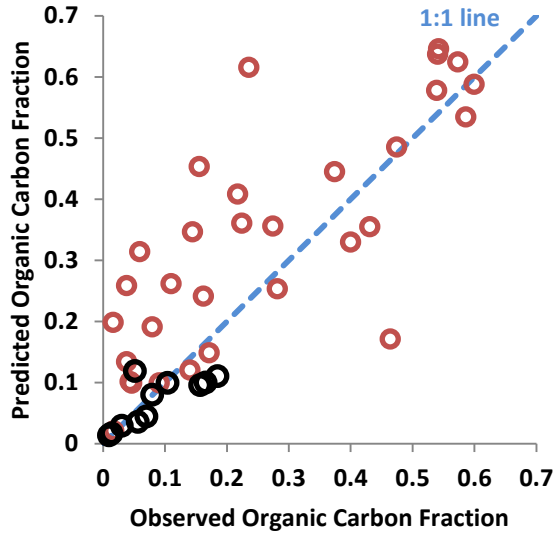
Fig. S1. Scatterplot of predicted vs. observed organic carbon fraction of sea spray for the Mace Head (red) and Point Reyes (black) sites. The blue dashed line shows the 1:1 relationship.
