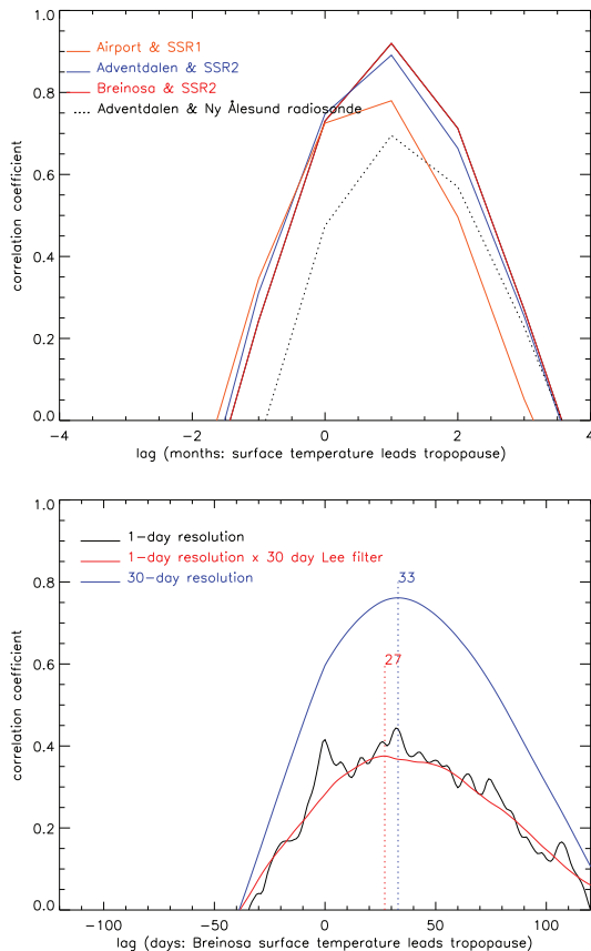
Fig. 4. Upper panel: updated version of results from Hall et al. (2009) showing correlations between tropopause determinations and temperature measurements (see text and Hall et al., 2009 for details). Lower panel: correlations based on daily data (variable line), 30-day smoothed correlation (smooth lower line), and correlation between daily temperature and 30-day smoothed tropopause height (upper smooth line). All temperatures from Breinosa.
