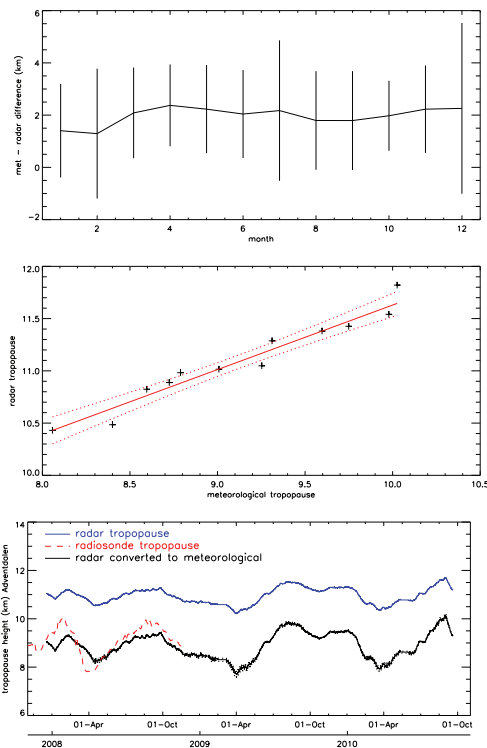
Fig. 3. Upper panel: the height difference between radar and radiosonde tropopause determinations. Although showing a distinct seasonal variation, the peak to peak magnitude is only 1 km. Middle panel: linear regression of radar tropopause on meteorological tropopause heights together with 95% confidence limits. Bottom panel: Tropopause determinations for the period of observation with 30-day Lee filter applied for clarity. Thin upper line: radar determination; lower dashed line: radiosonde determination; solid thick line: estimate the meteorological tropopause (uncertainties based on those of the regression indicated by dotted lines).
