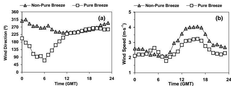
Fig. 9. Daily evolution of mean (a) wind direction and (b) wind speed for pure (51 days) and non-pure (55 days) breezes patterns during data-base used for this analysis.
