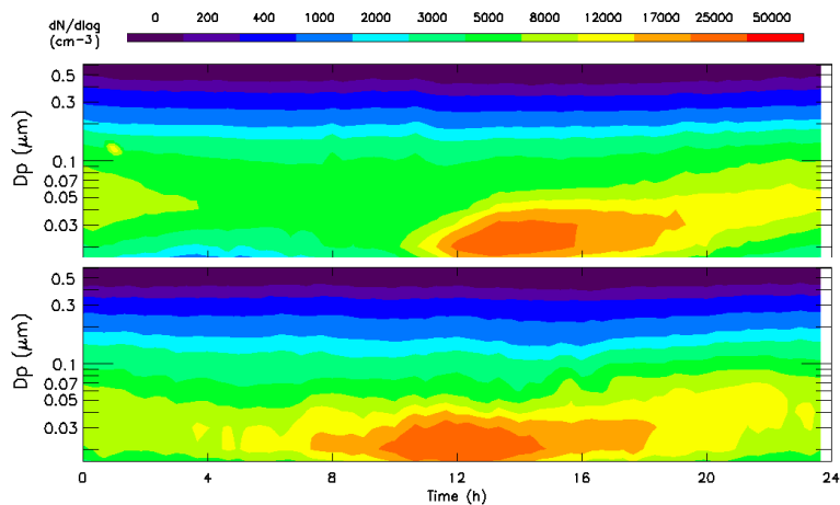
Fig. 11. Mean particle size distribution for new particle formation with (up) wind blowing from NE (Event N_1 , 48 days) and (down) blowing from NW (Event N_2 , 42 days) at El Arenosillo Station.
