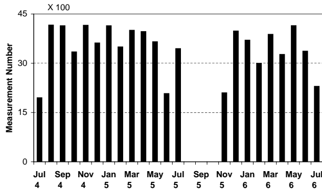
Fig. 3. Number of the particle number size distributions per month at El Arenosillo Station from the 10-min data-base used for the analysis.
