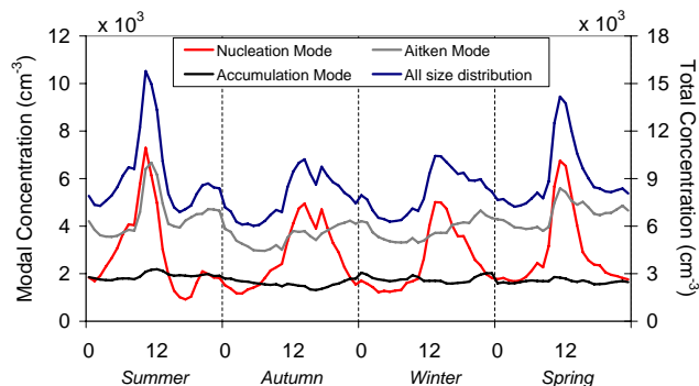
Fig. 7. Daily mean cycles of the total and nucleation, Aitken and accumulation mode concentrations per season, July–September (summer), October–December (autumn), January–March (winter) and April–June (spring).
