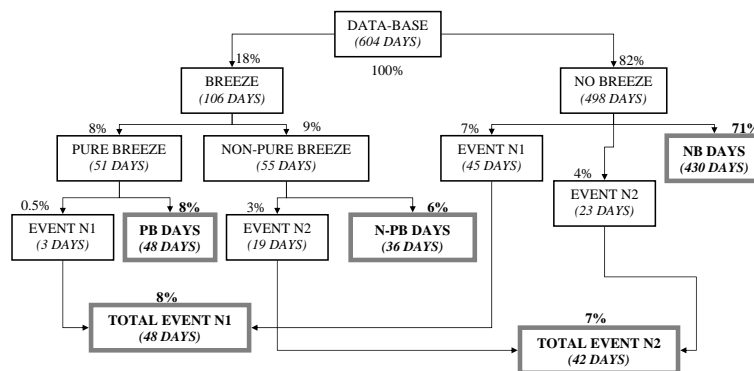
Fig. 8. Representative day's segregation by means of sea-land breezes (pure and non-pure) days and nucleation events ( N_1 and N_2 ).
