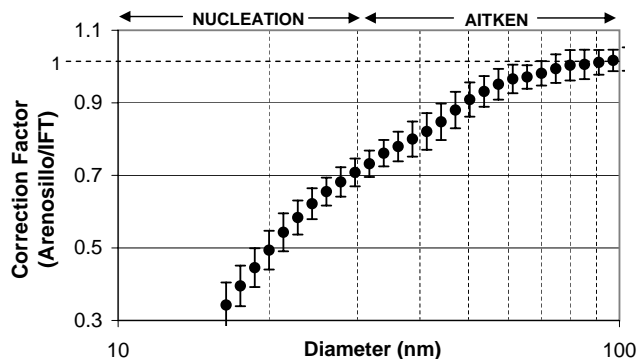
Fig. 2. Ratio of the size distribution measured by the SMPS-EI Arenosillo and the DMPS-IFT. It is defined as the Correction Factor (FC).
