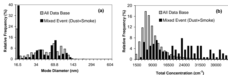
Fig. 4. The relative occurrence frequency of (a) mode diameter and (b) total particle concentration of 1-h data for the entire period of study and during the special mixed event.
