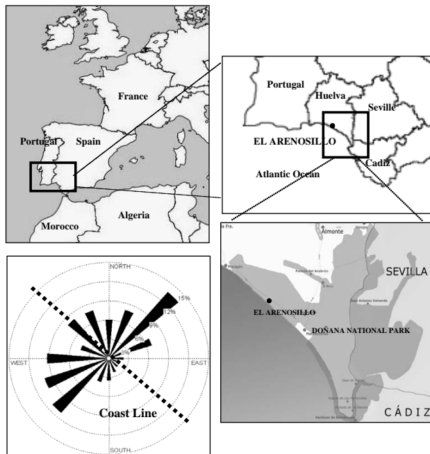
Fig. 1. Map of Iberian Peninsula highlighting the location of El Arenosillo Station, the (15/07/2004–31/07/2006) wind rose and the coastal line.
