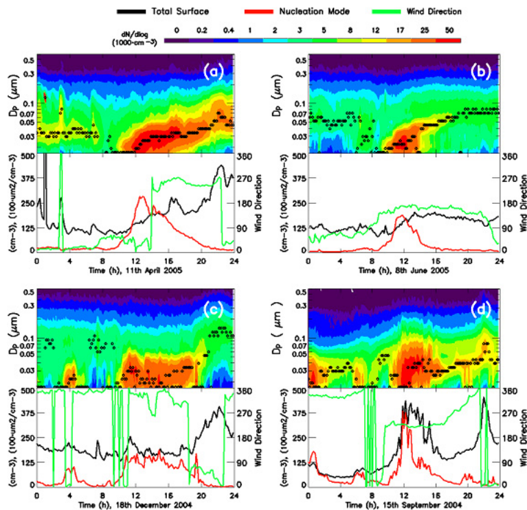
Fig. 10. Daily evolutions of the particle number size distribution at El Arenosillo Station, during (a) 11 April 2005, (b) 8 June 2005, (c) 18 December 2004 and (d) 15 September 2004. Total surface (black line), concentration for nucleation mode (red line), wind direction (green line) and mode diameter (black diamonds) are also represented.
