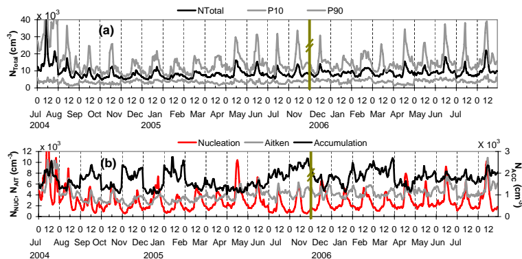
Fig. 6. Daily mean cycles per month of (a) total concentration ( N_T ) (black line) with the 10th and 90th percentiles (grey lines) (b) and concentrations for nucleation ( N_{NUC} ), Aitken ( N_{AIT} ) and accumulation ( N_{ACC} ) modes.
