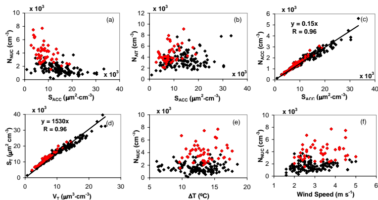
Fig. 12. 24-h averaged of several submicron aerosol physical properties and meteorological parameters at El Arenosillo station.
