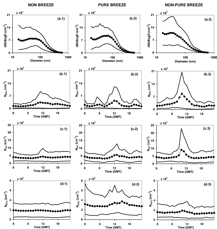
Fig. 14. Mean daily, 10th and 90th percentiles of particle number size distribution and for modal concentration corresponding to 430 NB-days (non breeze), 48 PB-days (Pure) and 36 N-PB-days (Non-Pure) breeze patterns at El Arenosillo.
