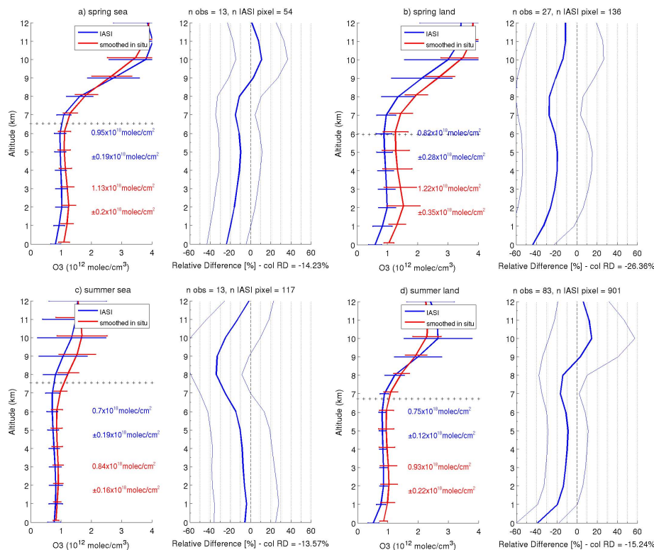
Fig. 9. Left panel: average IASI O 3 profiles (blue lines) and smoothed in situ profiles (red lines) in units of 10 12 molecules cm -3 for spring (top panels) and summer (bottom panels), over sea ( a and c ) and land ( b and d ). The horizontal dashed black line represents the mean position of the maximum altitude reached by each particular aircraft. Errors bars represent the variability of measurements. The coloured numbers indicate the average [0–8 km] columns in 10 17 molecules cm -2 and the standard deviation. Right panel: average relative differences in % (thick blue lines for profiles and numbers below the graphs on the right are the average differences for [0–8 km] columns and \pm 1\sigma (thin blue lines) are also plotted as a function of altitude. The number of in situ observations and IASI co-located pixels are noted at the top right of the panels. The mean ECMWF dynamical tropopause is at 7.8, 8.2, 10.4 and 9.5 km, respectively.
