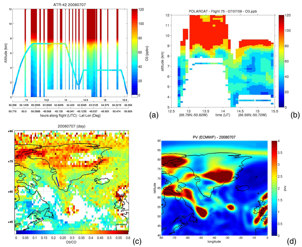
Fig. 12. The color boxes following the flight pattern on 7 July 2008 are cross sections representing the in situ O 3 volume mixing ratios (ppbv) compared to IASI O 3 vertical distributions co-located with the ATR-42 flight using a criteria of [\pm 0.2^\circ; \pm 1\text{ h}] (a) and O 3 lidar vertical measurements (b). In situ (a) and lidar (b) data are plotted as a function of altitude versus time (UTC) along the flight track. The latitude and longitude on x-axis corresponds to the aircraft position (a). Distribution of the ratio between daytime IASI O 3 [0–8 km] partial columns and IASI CO total columns over Greenland on a 1^\circ \times 1^\circ grid with the ATR-42 flight track shown as a blue line (c). White areas indicate no data. Potential vorticity (in PVU) at 8 km over Greenland taken from an ECMWF analysis data at 12:00 UTC on 7 July 2008 (d).
