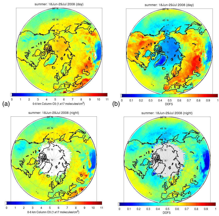
Fig. 5. Same as Fig. 4 for the summer period. White areas indicate no data.
