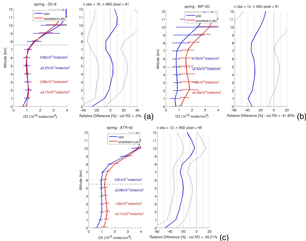
Fig. 6. Left panel: average IASI O 3 profiles (blue lines) and smoothed in situ profiles (red lines) in units of 10 12 molecules cm -3 for each spring aircraft campaign; the horizontal dashed black line represents the mean position of the maximum altitude reached by each particular aircraft. Errors bars represent the variability of measurements. The coloured numbers indicate the average [0–8 km] columns in 10 17 molecules cm -2 together with the standard deviation. Right panel: average relative difference in % (thick blue lines for profiles and numbers below the graphs on the right are the average differences for [0–8 km] columns) and ±1σ (thin blue lines). The number of in situ observations and IASI co-located pixels are noted at the top of the panels on the right. The relative differences are calculated as follows: [(IASI – smoothed in situ)/(smoothed in situ)] · 100. The smoothed in situ profiles are the in situ aircraft measurements completed with the ACE-FTS climatology and convolved with IASI AK (see text for details). Results are shown for the DC-8 (a), the WP-3D (b) and the ATR-42 (c). The mean ECMWF dynamical tropopause is at 8, 8.5 and 7.8 km, respectively.
