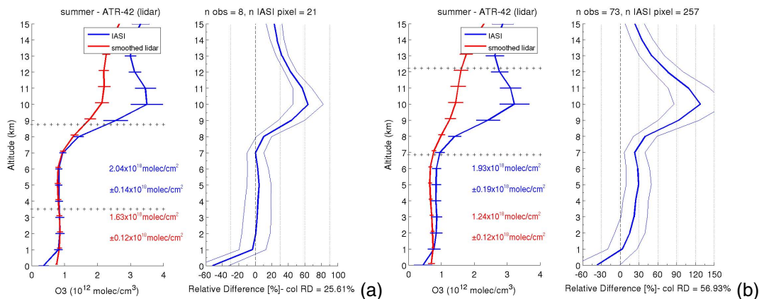
Fig. 8. Left panel: average IASI O 3 profiles (blue lines) and smoothed ATR-42 lidar profiles (red lines) in units of 10^{12} molecules \text{cm}^{-3} . Lidar profiles are separated according to the flight altitude of the ATR-42, below or equal to 4 km (a) and above 4 km (b). The upper horizontal dashed black line represents the mean altitude where the lidar profile ends and the climatology starts. The lower horizontal dashed black line represents the mean altitude where the a priori ends and the lidar profile starts. The coloured numbers indicate the average [0–12 km] column in 10^{17} molecules \text{cm}^{-2} and the standard deviation. Right panel: average relative difference in % (thick blue lines for profiles and numbers below graphs on the right are the average differences for [0–12 km] columns) and \pm 1\sigma (thin blue lines). The number of lidar observations and IASI co-located pixels are noted at the top right of the panels. The relative differences are calculated as follows: [(\text{IASI} - \text{smoothed lidar}) / (\text{smoothed lidar})] \cdot 100 . The smoothed lidar profiles are the measurements completed with the ACE-FTS climatology and the a priori, and convolved with IASI AK (see text for details). The mean ECMWF dynamical tropopause is at 8.4 and 8.8 km, respectively.
