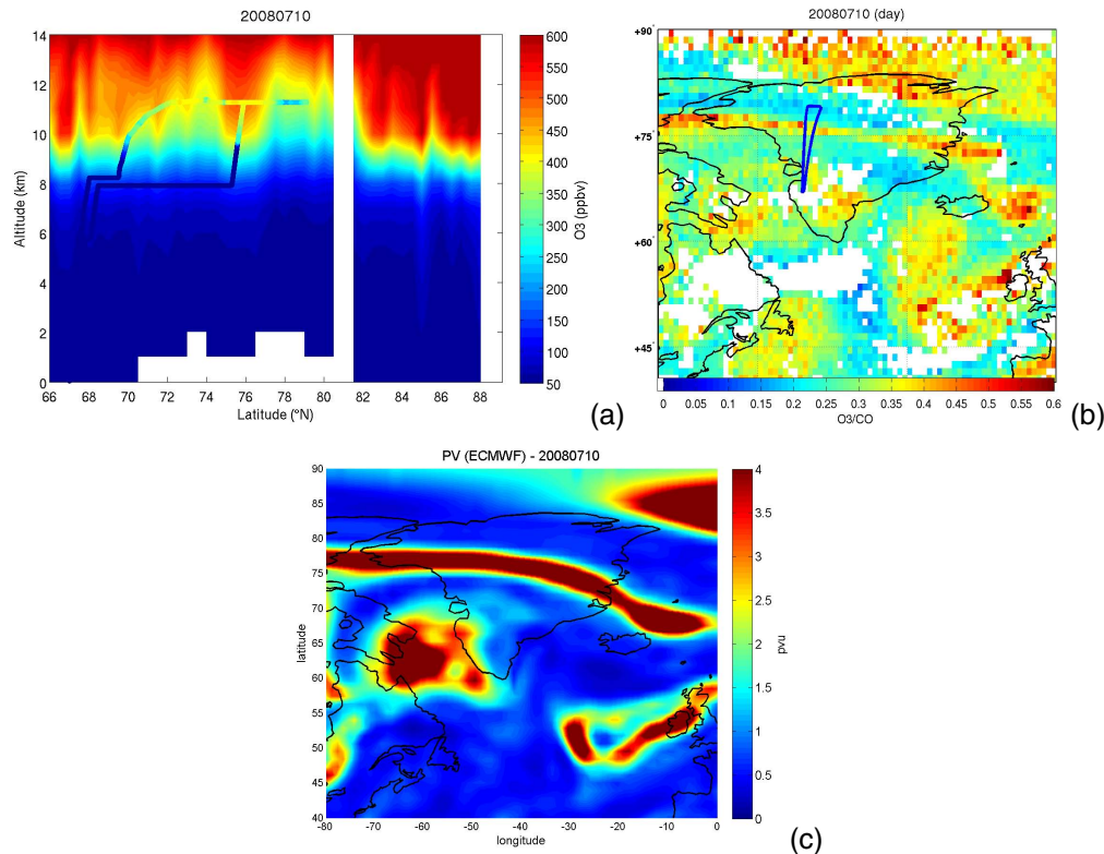
Fig. 11. (a): the color box following the Falcon-20 flight pattern on 10 July 2008 is the cross section representing the in situ O 3 volume mixing ratios (ppbv) compared to IASI O 3 vertical distributions. IASI data are averages data between 49° W and 51° W and sampled every 0.5° between 66° N and 89° N. (b): distributions of the ratio between daytime IASI O 3 [0–8 km] partial columns and IASI CO total columns over Greenland on a 1° × 1° grid. The Falcon-20 flight track is plotted in blue. In (a) and (b), white areas indicate no data. (c): potential vorticity (in PVU) at 8 km over Greenland taken from an ECMWF analysis data at 12:00 UTC on 10 July 2008.
