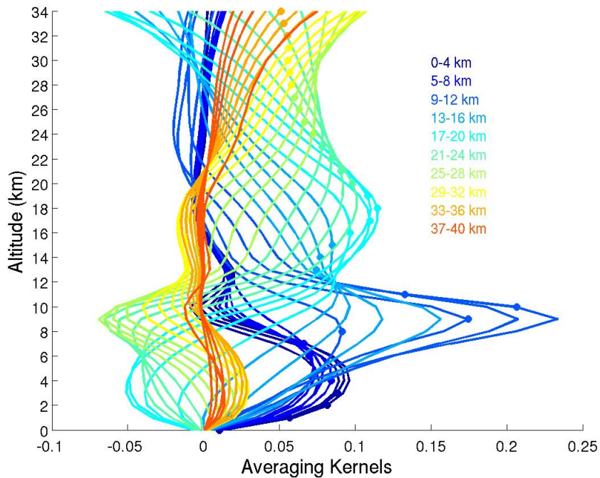
Fig. 3. Averaging kernel functions for different altitudes from FORLI-O 3 retrievals (DOFS = 3.3) at 63.7° N, 20.4° W.
