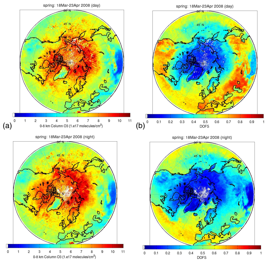
Fig. 4. Maps of IASI [0–8 km] O 3 columns (a) and corresponding DOFS (b) on a 1° × 1° grid for the spring campaign for daytime (top) and night-time (bottom). White areas indicate no data.
