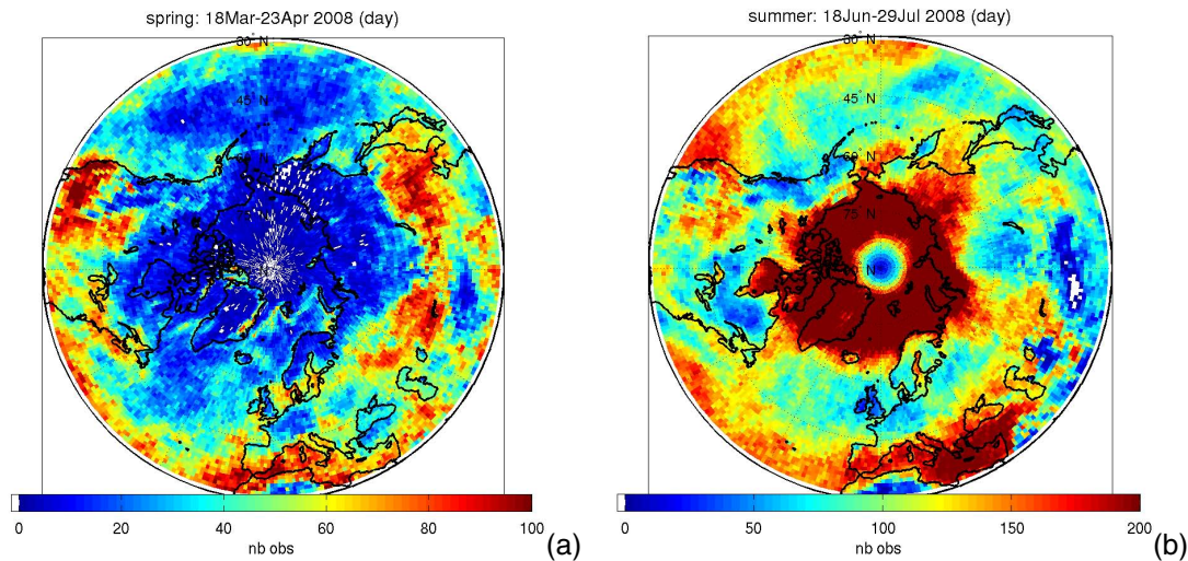
Fig. 2. Distribution of the number of daytime IASI data gridded on 1^\circ \times 1^\circ using the RMS and bias filter for the spring (a) and summer (b) POLARCAT campaigns. White areas indicate no data. Note that the colour scale is multiplied by 2 in summer.
