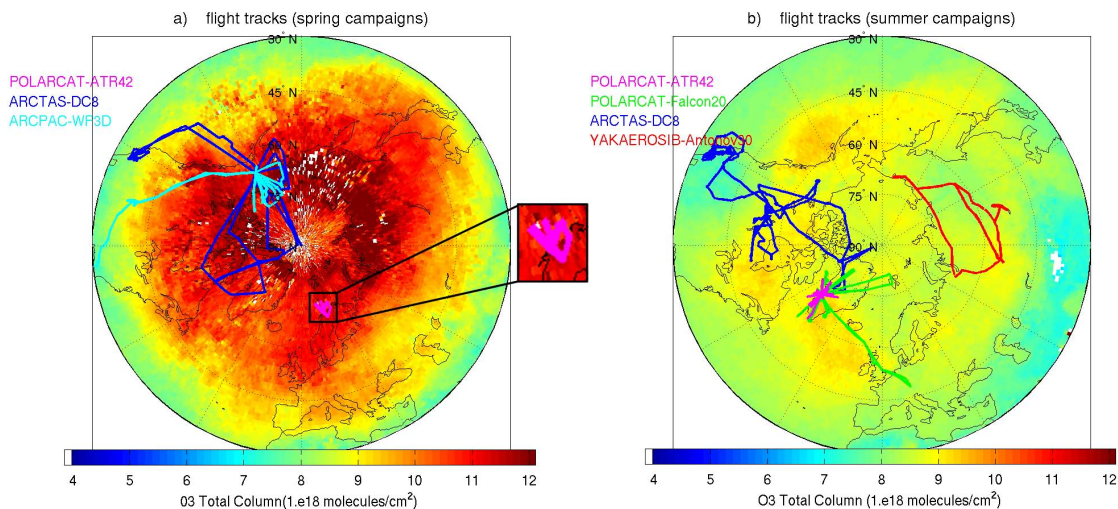
Fig. 1. Global distributions of daytime IASI O 3 total columns averaged for 18 March to 23 April 2008 (period of POLARCAT spring campaigns) with a zoom on ATR-42 flight area (a) and for 18 June to 29 July 2008 (period of POLARCAT summer campaigns) (b) . IASI data are averaged over a 1° × 1° grid. White areas indicate no data. Flight-tracks for all flights of the DC-8 (blue), ATR-42 (magenta), WP-3D (cyan), Falcon-20 (green) and Antonov-30 (red) aircraft are superimposed on the maps.
