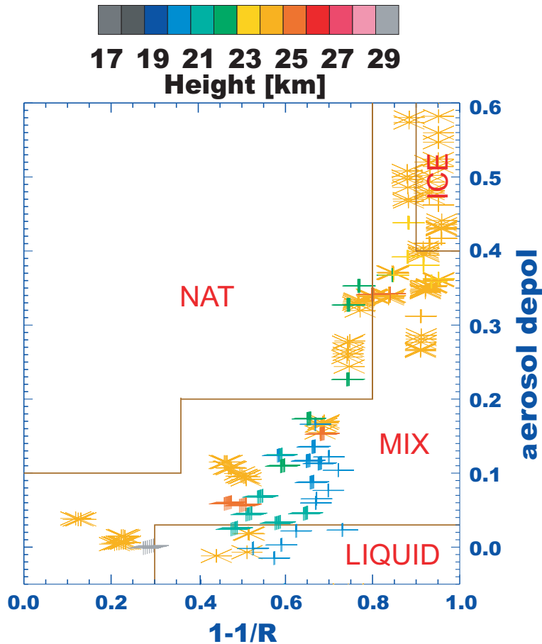
Fig. 2. PSC classification scheme for the inhomogeneous PSC observed on 2 January 2008 (see Fig. 1). The boundaries for NAT, Ice, mixed-particle, and STS PSCs are drawn into the plot as lines. The different colors and symbols represent the height of the PSCs.
