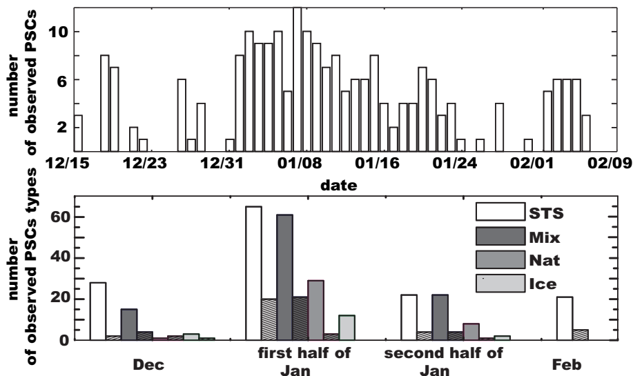
Fig. 3. (a) Daily resolved number of PSCs detected in CALIPSO measurements north of 60° N during winter 2007/2008. PSCs with a large spatial extent might be counted multiple times as they show up subsequent CALIPSO tracks. CALIPSO passes the arctic every 100 min with about 25° longitude shift between. (b) Analysis of the PSC observations in accordance to their type. Unshaded and shaded bars refer to observations over tropospheric clouds or during the absence of tropospheric clouds, respectively. The distribution differs from the display in (a) because individual PSCs might contain areas of different composition.
