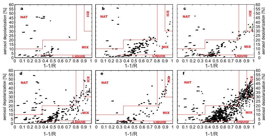
Fig. 4. PSCs detected by CALIPSO classified according to Massoli et al. (2006) with respect to the type of the underlying tropospheric cloud system: cirrus ( a ), mid-tropospheric clouds ( b ), and an absence of tropospheric clouds ( c ). Deep-tropospheric clouds were further distinguished with respect to the overlap between the PSC and the tropospheric cloud layer: PSC had the same ( d ) or a larger spatial extent ( e ) as the underlying deep-tropospheric clouds or the PSC was observed over a mixture of deep-tropospheric clouds and mid-tropospheric clouds ( f ). One dot represents one height bin (60 m vertical resolution, 180 m smoothing length) of a CALIPSO profile obtained with spacial averaging over 1^{\circ} – 10^{\circ} longitude (see Sect. 2).
