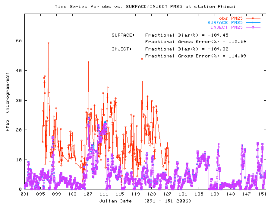
Figure S1. CO, Ozone and PM2.5 Model Performance at Phimai
