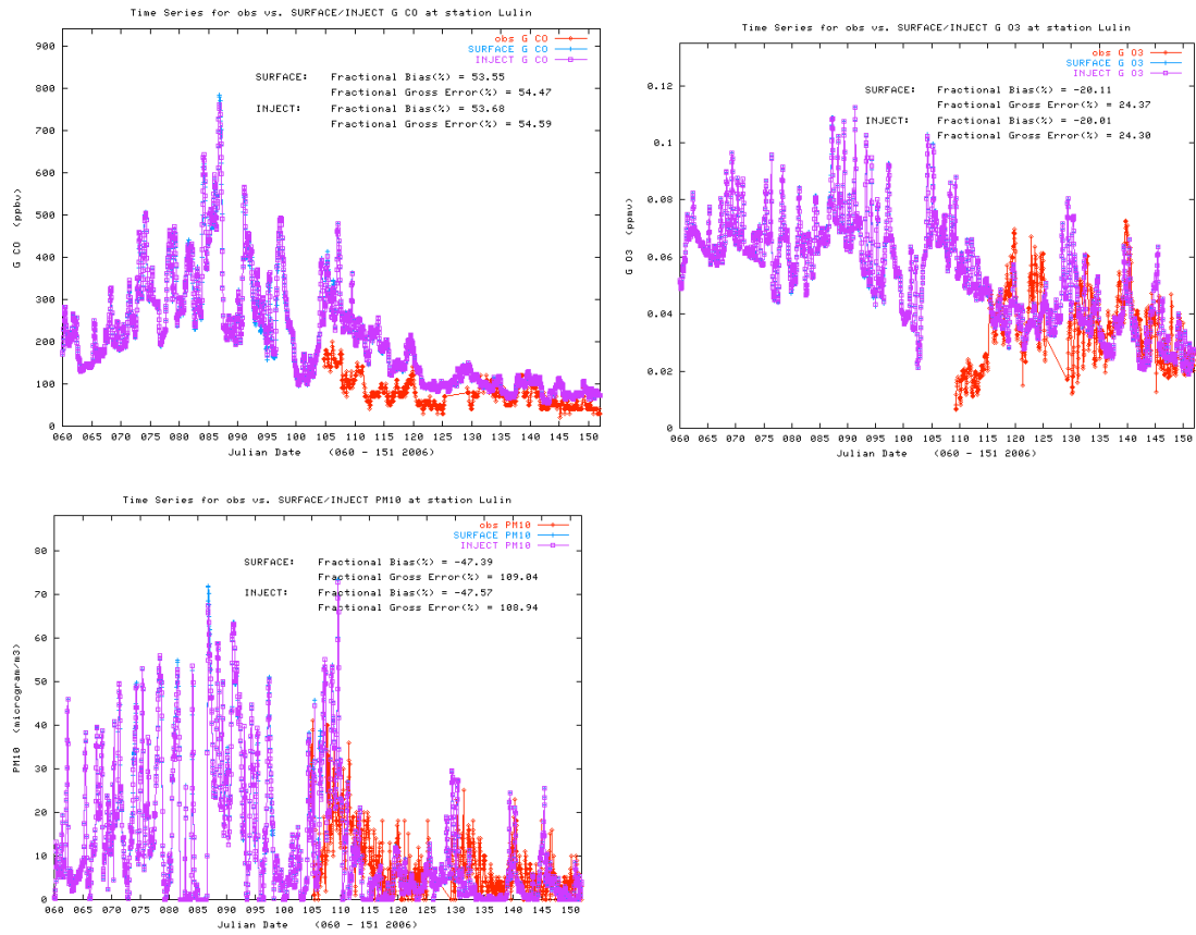
Figure S3. Model Performance of the SUFACE and INJECT Methods at Lulin, Taiwan
