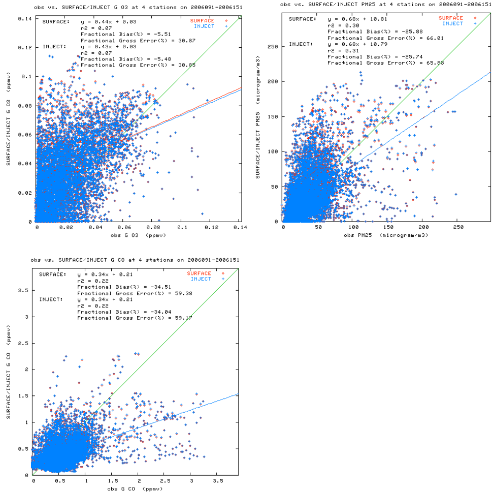
Figure S2. Model Performance of the SURFACE and INJECT Methods at Hong Kong (4 sites)
