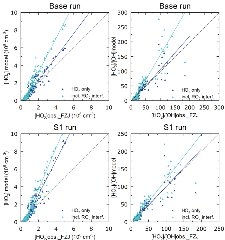
Fig. 8. Scatterplots between HO 2 and HO 2 /OH ratios observed by FZJ instrument and those modeled, without taking RO 2 interference into account (HO 2 only, dark blue), and taking the interference into account (i.e., on the basis of HO 2 (*), light blue). The results are shown for the base run (upper panels) and S1 run (lower panels).
