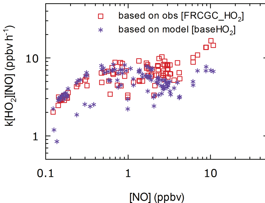
Fig. 11. HO 2 + NO reaction rates derived from HO 2 observed by FRCGC instrument (red squares), and HO 2 modeled by the base run (purple stars) plotted as a function of NO. Only midday (09:00–15:00 UTC) data are used.
