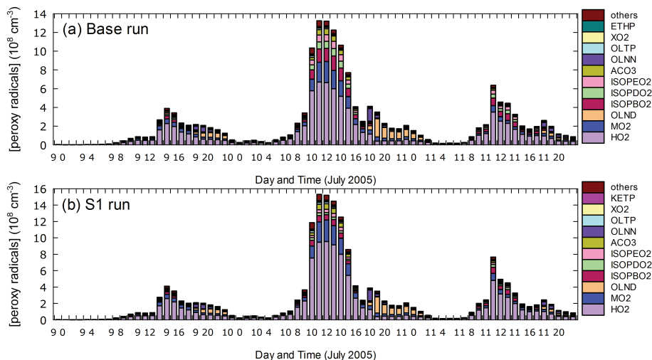
Fig. 5. Breakdown of peroxy radicals (HO 2 and RO 2 ) in the base and S1 runs. MO 2 , OLND, OLNN, ACO 3 , OLTP, ETHP, KETP, and XO 2 , stand for methyl peroxy radical, NO 3 –alkene adduct (reacting via decomposition), NO 3 –alkene adduct (reacting to form HO 2 ), saturated acylperoxy radicals, peroxy radicals from OLT (terminal olefins), peroxy radicals from ethane, peroxy radicals from ketones, and parameterized peroxy radicals accounting for additional NO to NO 2 conversions, respectively.
