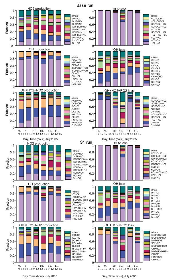
Fig. 4. Breakdown of production and loss processes of OH, HO 2 , and radical group (OH + HO 2 + RO 2 ) in the base and S1 runs.
