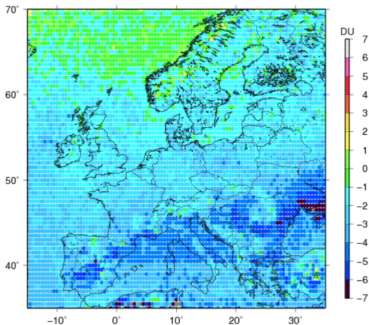
Fig. 6a. Summer 2008 average differences (in DU) between smoothed 0–6 km ozone columns: model median minus IASI.
