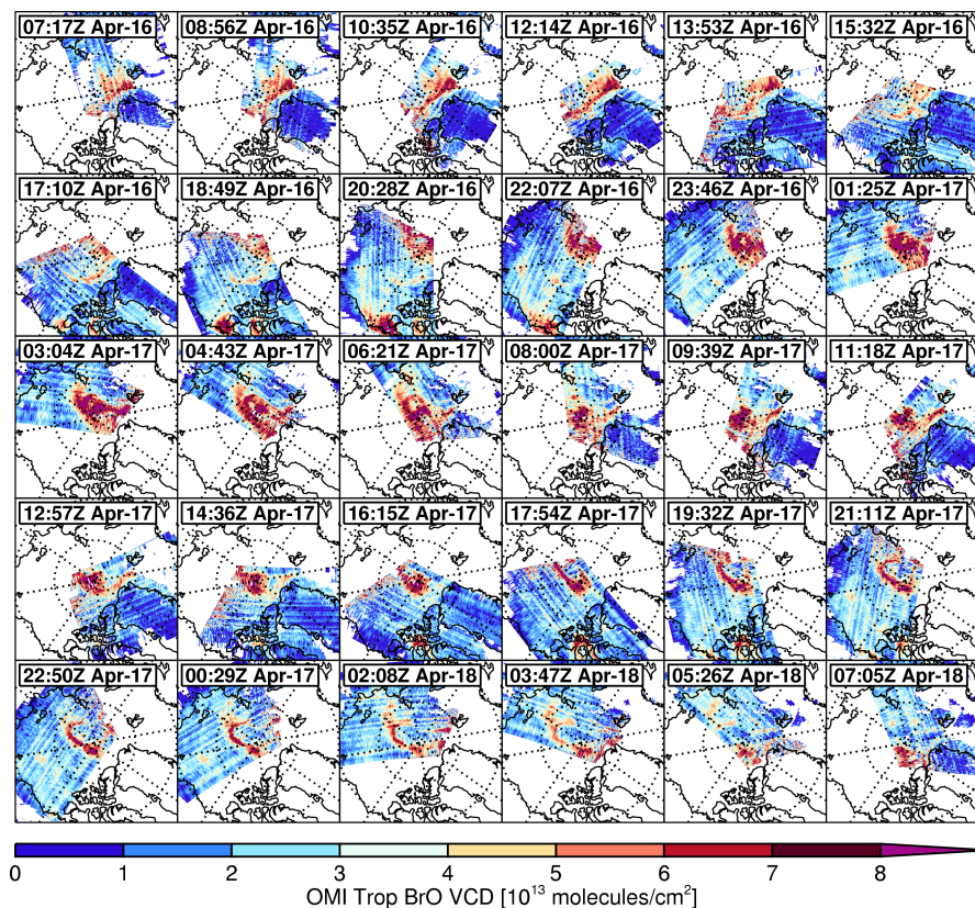
Fig. 11. OMI tropospheric BrO VCD for different orbits (UTC time as indicated) from 16 to 18 April 2008.
