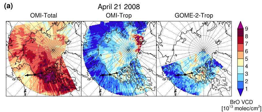
Fig. 10a. Similar to Fig. 6a but for the WP-3D flight of 21 April 2008.
