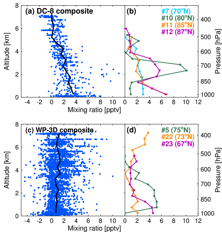
Fig. 2. (a) Collection of DC-8 measurements of BrO (blue dots) and DC-8 composite BrO profile (black line) and (b) DC-8 BrO profiles #7, #10, #11 and #12, (c) similar to (a) but for WP-3D measurements of BrO, (d) WP-3D BrO profiles #5, #22, and #23.
