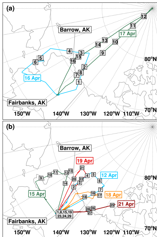
Fig. 1. Flight tracks and the locations of BrO profiles measured by instruments on board the (a) NASA DC-8 aircraft during ARCTAS and (b) NOAA WP-3D aircraft during ARCPAC.
