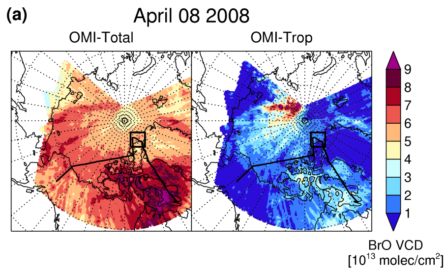
Fig. 8a. Similar to Fig. 6a but for the DC-8 flight on 8 April 2008. GOME-2 data are not available for this flight. The location of severe ozone depletion and high active bromine is marked with a black square.
