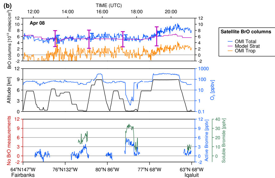
Fig. 8b. Similar to Fig. 7b but for the DC-8 flight on 8 April 2008.
