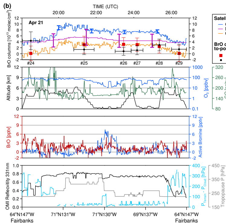
Fig. 10b. Similar to Fig. 9b but for the WP-3D flight on 21 April 2008, with tropopause pressure added.
