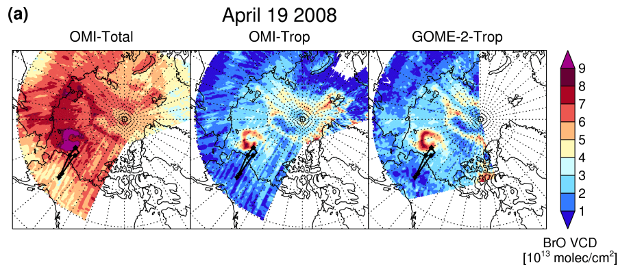
Fig. 9a. Similar to Fig. 6a but for the WP-3D flight of 19 April 2008.
