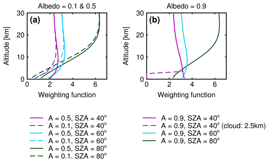
Fig. 3. BrO weighting functions at 344.6 nm for various solar zenith angles (SZA) and surface albedos for (a) clear sky conditions and (b) clear and cloudy sky conditions, where the cloudy case is for an optically thick cloud (cloud extinction coefficient = 300).
