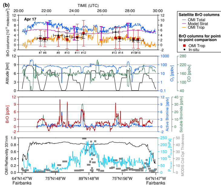
Fig. 6b. Time series plots for NASA ARCTAS DC-8 flight of 17 April 2008 with line colors corresponding to the same color y axis. The top panel shows various estimates of VCD of BrO along the DC-8 flight track, including OMI total column, the modeled stratospheric column, and tropospheric columns based on aircraft in-situ measurements (black dots) as well as our analysis of OMI retrievals (red squares). The error bars of the tropospheric columns are described in the text. The two middle panels show various aircraft in-situ measurements along with the flight altitude. The bottom panel shows OMI reflectivity at 331 nm and cloud retrieved parameters from OMI and MODIS, as described in the text. The measurement accuracy of DC-8 BrO measurements is \pm 40\% . Soluble bromide is not plotted when the mixing ratio is below the detection limit (1–6 pptv).
