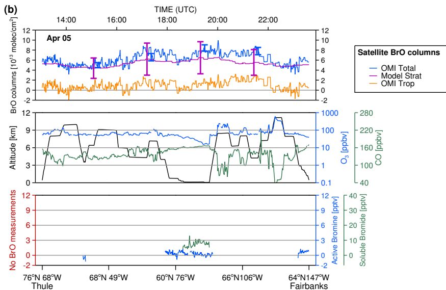
Fig. 7b. Similar to Fig. 6b but for the DC-8 flight on 5 April 2008. Aircraft in situ BrO measurements are not available for this flight.
