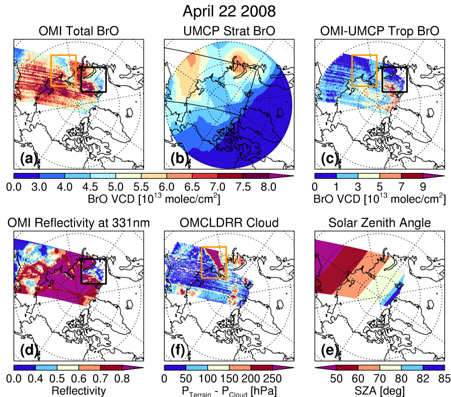
Fig. 5. Various parameters and estimated quantities for OMI orbit 20050 at 03:23 UTC on 22 April 2008 highlighting reduced tropospheric BrO over low albedo surfaces (black box) and reduced BrO in the presence of shielding clouds (orange box). See text for more details and discussion.
