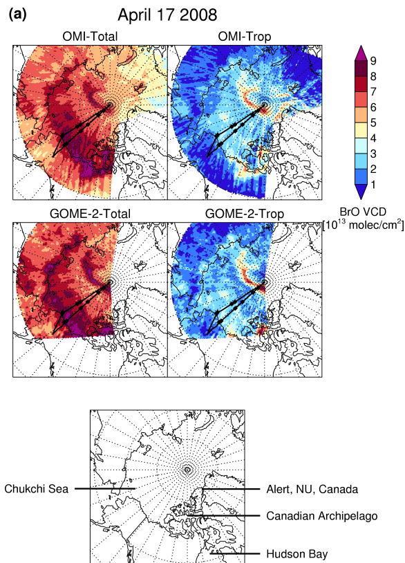
Fig. 6a. Maps on 17 April 2008 of (top left) OMI total vertical column density (VCD) of BrO, (top right) OMI tropospheric VCD of BrO, (middle left) GOME-2 total VCD of BrO, and (middle right) GOME-2 tropospheric VCD of BrO column. Negative values are included as dark blue. The flight track of the DC-8 on 17 April 2008 is indicated by black lines; aircraft profile locations where BrO was measured are marked with black diamonds. (Bottom) Geographic regions of interest described in the paper.
