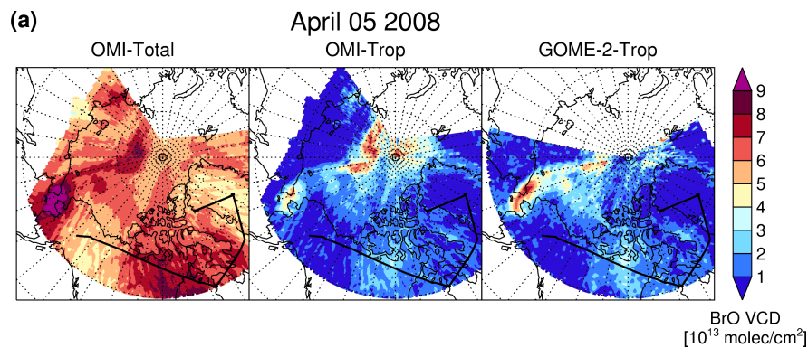
Fig. 7a. Similar to Fig. 6a but for the DC-8 flight on 5 April 2008.
