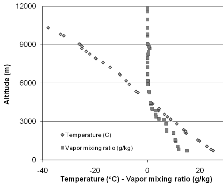
Fig. 1b. Radiosonde of 3 March 2003 at São Paulo airport (12:00 GMT), with temperature ( ^{\circ}\text{C} ) and vapor ratio ( \text{g kg}^{-1} ) vertical profiles.
