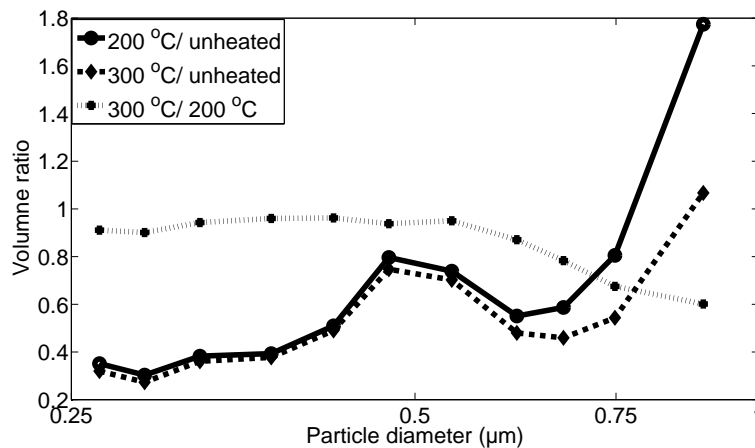
Fig. 5. Volume ratio distribution for different temperature increments.
