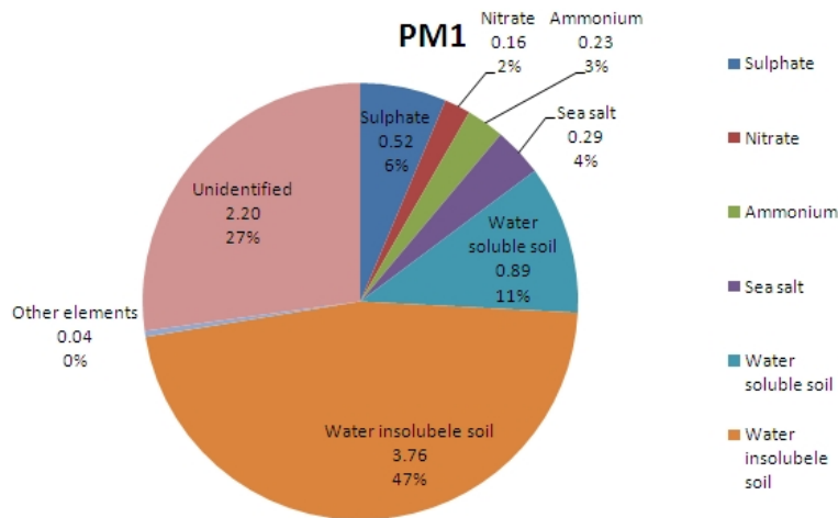
Fig. 6. Chemical composition of PM 1 measured at Hornsgatan.
