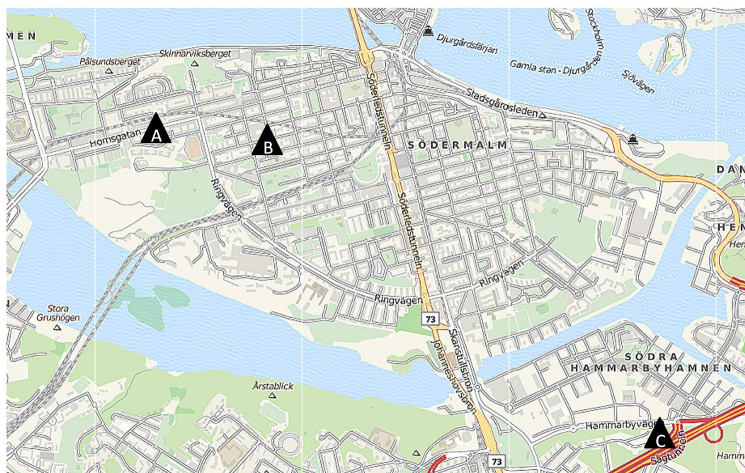
Fig. 1. Location of the monitoring stations in Stockholm: Hornsgatan ( A ), Torkel Knutssongatan ( B ) and Kalmgatan ( C ). Blue indicates water surfaces, green forest/park areas, grey built-up areas and red yellow important roads.
