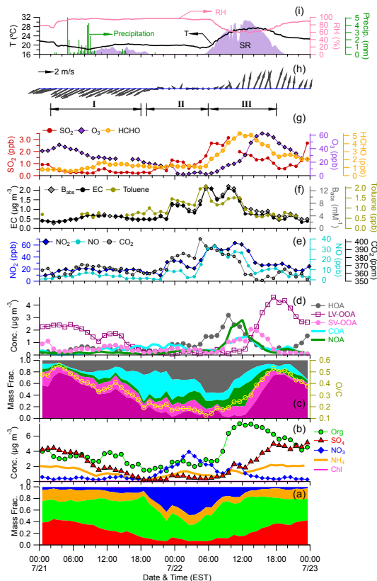
Fig. 1. Time series of meteorology (relative humidity, temperature, precipitation, solar radiation, wind direction, and wind speed), gaseous species, EC and absorption ( B_{\text{abs}} ), hourly average mass concentrations and fractions of NR species (organics, sulfate, ammonium, nitrate, and chloride) and OA components (LV-OOA, SV-OOA, HOA, COA, and NOA), and O/C ratio of OA from 21–22 July. Three stages representing different atmospheric processes are marked as I, II, and III, respectively.
