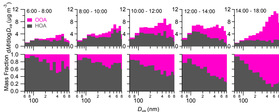
Fig. 7. Average size distributions of HOA and OOA for selected time ranges on 22 July.
