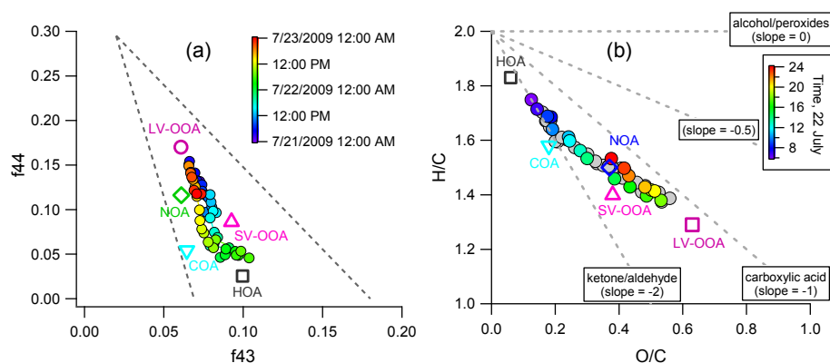
Fig. 5. (a) Relationship between f_{44} (fraction of m/z 44 to total organic signal) and f_{43} (fraction of m/z 43 to total organic signal) from 21–22 July. The f_{44} vs f_{43} for five OA components are also shown. The dash lines represent the triangle region from Ng et al. (2010). (b) Van Krevelen diagram for OA from 21–22 July and OA components identified from PMF analysis.
