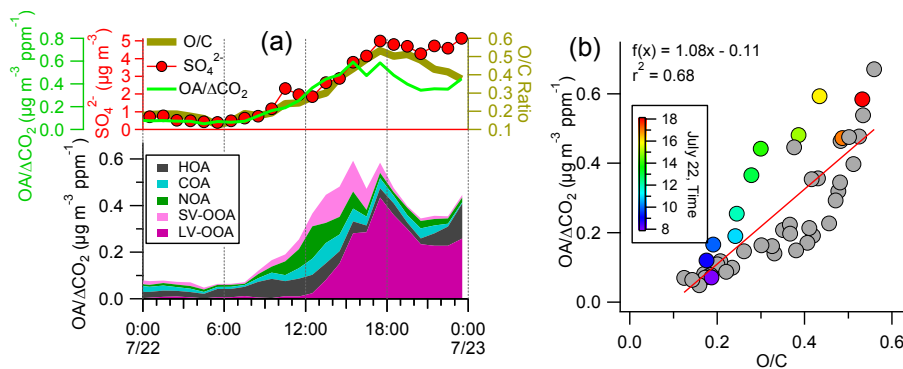
Fig. 6. Evolution of (a) O/C, sulfate, OA/\Delta CO_2 on 22 July, (b) correlations between OA/\Delta CO_2 and O/C ratio for the period of 21–22 July. The data points between 08:00–18:00 on 22 July are colored by the time.
