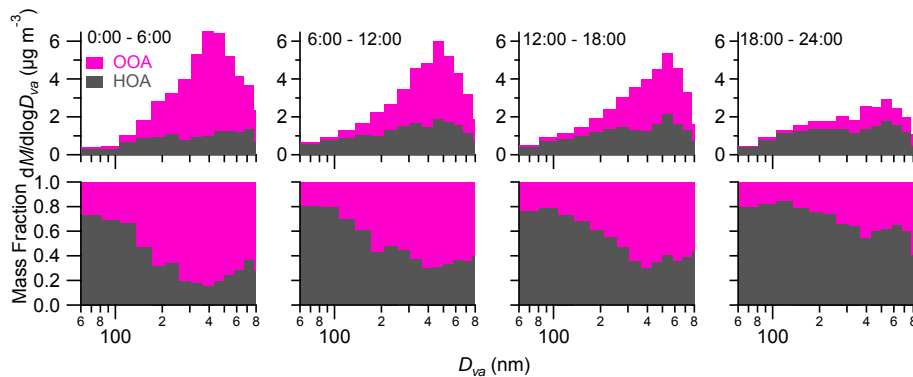
Fig. 3. Average size distributions of HOA and OOA every six hours on 21 July.
