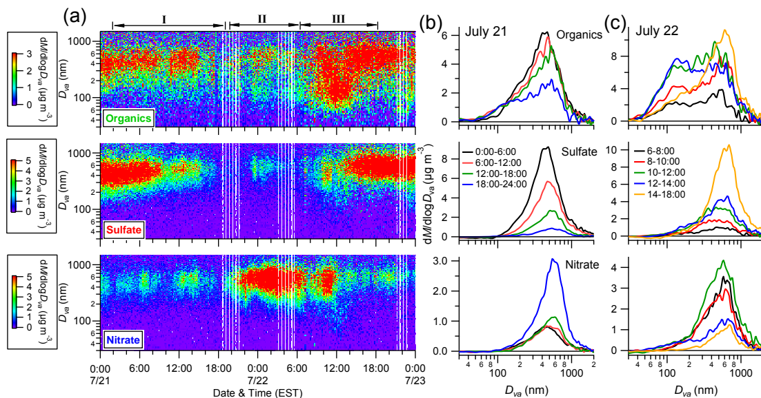
Fig. 2. Evolution of size distributions for the mass concentrations of organics, sulfate, and nitrate. (b), (c) shows the average size distributions of aerosol species for selected time ranges on 21 and 22 July, respectively.
