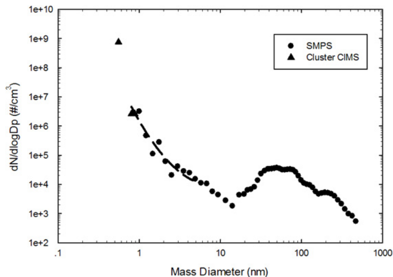
Fig. A4. Particle size distribution observed on 13:00, 7 August 2009. Filled triangles are data obtained by the cluster chemical ionization mass spectrometer (Cluster CIMS) and filled circles are data obtained from two scanning mobility particle spectrometers (SMPS) (Jiang et al., 2011b). The dashed line is obtained by fitting a second order polynomial using the method of least squares to the data over the size range where growth rates are calculated in this work.
