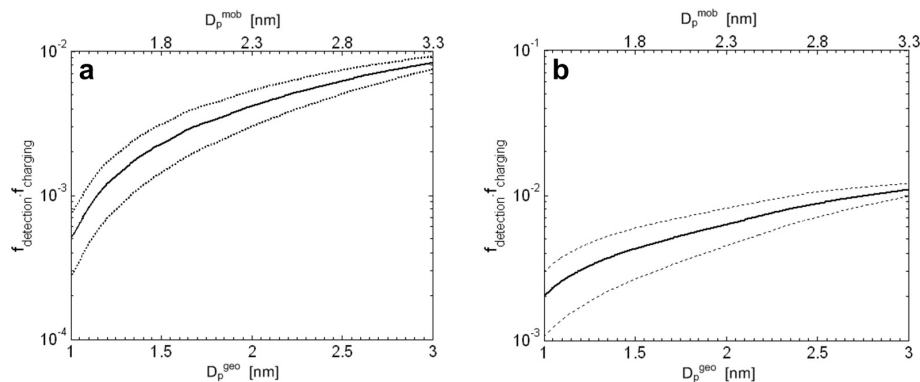
Fig. C2. Upper and lower bound estimates (dotted lines) to the quantity f_{\text{detection}} \cdot f_{\text{charging}} (the product of size-dependent detection and charging efficiencies) as a function of particle mobility diameter D_p^{\text{mob}} (upper abscissa) and particle geometric diameter D_p^{\text{geo}} (lower abscissa) obtained for DEG SMPS operation during (a) NCCN and (b) the NCAR campaign. The differences between the two figures arise from differences in the detection efficiency: the DEG UCPC was operated at higher flow rates and super-saturation ratios during the NCAR study. For both campaigns, the same size-dependent systematic relative uncertainty in f_{\text{detection}} \cdot f_{\text{charging}} was assumed, linearly decreasing from \pm 50\% at 1 nm geometric diameter to \pm 10\% at 3 nm geometric diameter. The solid black line represents the product of the size-dependent detection efficiency of negatively charged NaCl and the bipolar charging efficiency using the parameterization of Wiedensohler (1988). Geometric particle diameters were estimated according to Larriba et al. (2011).
