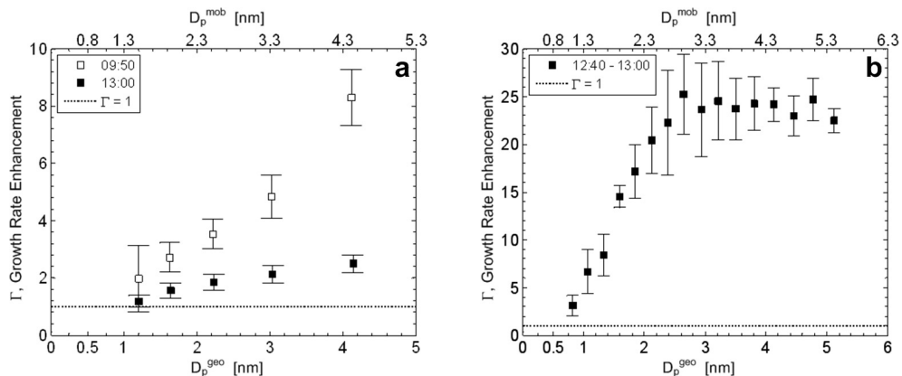
Fig. 2. Values of the growth rate enhancement \Gamma and their corresponding uncertainties are plotted as a function of particle mobility diameter D_p^{mob} (upper abscissa) and particle geometric diameter D_p^{geo} (lower abscissa) for the NPF event observed on (a) 7 August 2009 (NCCN), where uncertainties are presented as one standard deviation, and on (b) 19 September 2010 (NCAR) where uncertainties are presented as one standard error, calculated according to Cantrell (2008). A dotted line indicating \Gamma = 1 is shown for reference. Geometric particle diameters were estimated according to Larriba et al. (2011).
