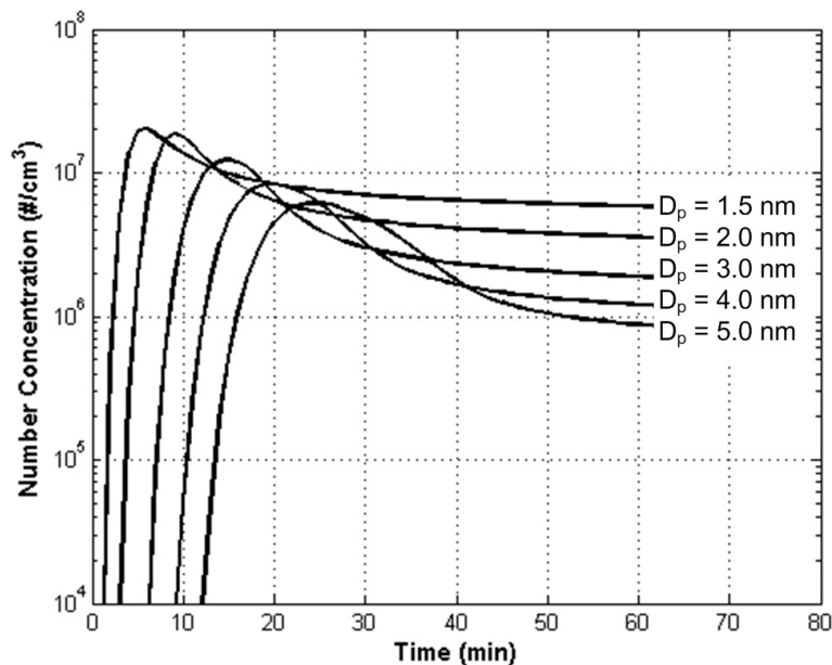
Fig. A3. Time-dependent particle number concentrations at various particle diameters D_p for collision-controlled nucleation in the free-molecular regime for a system that is initially particle-free. For particles smaller than 5 nm, less than an hour is needed to reach a quasi-steady-state. After quasi-steady state is reached, the decrease in number concentration is due to the increase of aerosol surface area (a coagulation sink), and does not depend explicitly on time.
