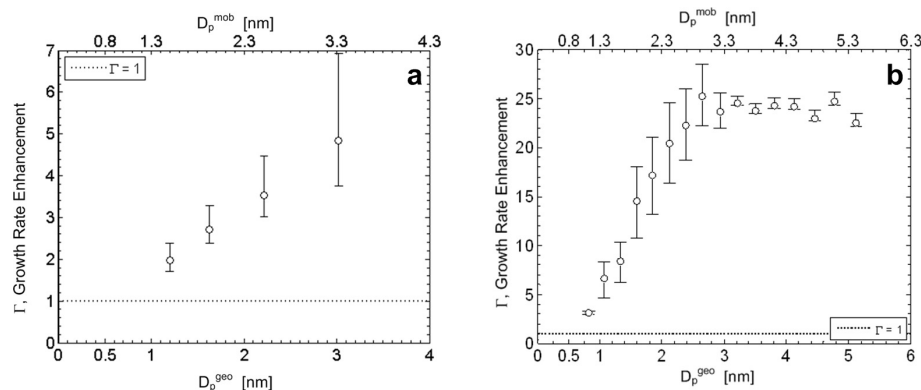
Fig. C3. Effects of systematic uncertainties in particle detection and charging efficiencies on growth rate enhancement \Gamma as a function of particle mobility diameter D_p^{\text{mob}} (upper abscissa) and particle geometric diameter D_p^{\text{geo}} (lower abscissa) for the NPF event observed on (a) 7 August 2009 (09:50, NCCN) and on (b) 19 September 2010 (12:40–13:00, NCAR). Values of \Gamma calculated using the size-dependent detection efficiency of negatively charged NaCl and the bipolar charging efficiency using the parameterization of Wiedensohler (1988) are presented as open circles. Resulting upper and lower limits on \Gamma , based on assumed systematic uncertainties in the product f_{\text{detection}} \cdot f_{\text{charging}} , are shown for each value of \Gamma as horizontal bars. A line indicating \Gamma = 1 is shown for reference. Geometric particle diameters were estimated according to Larriba et al. (2011).
