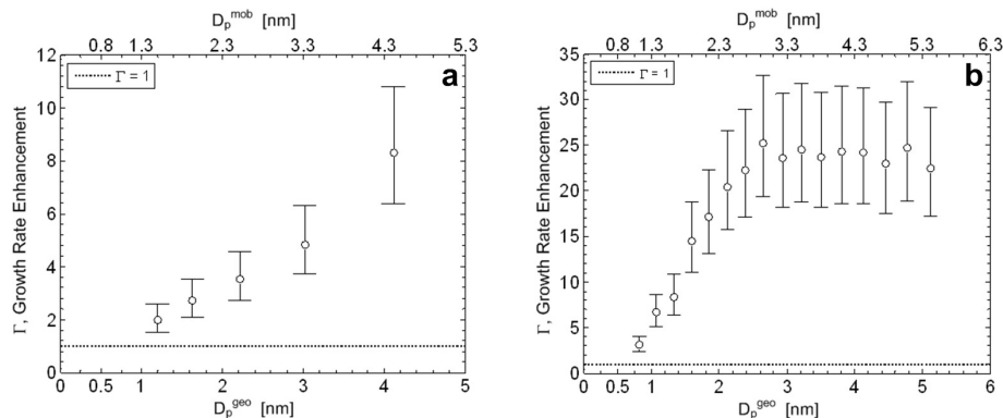
Fig. C1. Effect of systematic uncertainties in [\text{H}_2\text{SO}_4] on growth rate enhancement \Gamma as a function of particle mobility diameter D_p^{\text{mob}} (upper abscissa) and particle geometric diameter D_p^{\text{geo}} (lower abscissa) for the NPF event observed on (a) 7 August 2009 (09:50, NCCN) and on (b) 19 September 2010 (12:40–13:00, NCAR). Values of \Gamma calculated using the median values of [\text{H}_2\text{SO}_4] are presented as open circles. Resulting upper and lower limits on \Gamma , based on lower and upper limits on [\text{H}_2\text{SO}_4] known to within a factor of 1.3, are shown for each value of \Gamma as horizontal bars. A line indicating \Gamma = 1 is shown for reference. Geometric particle diameters were estimated according to Larriba et al. (2011).
