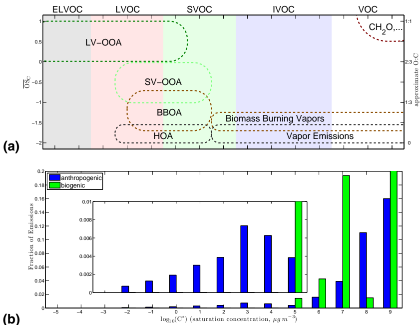
Fig. 1. (a) Volatility ( C^* in \mu\text{g m}^{-3} ) and oxidation state ( \overline{\text{OS}}_C ) for important atmospheric organics. Note the enormous range on the (logarithmic) x-axis. The volatility ranges described in the text are indicated by colored bands: aerosols are located in the ELVOC (gray), LVOC (red) and SVOC (green) range. Factors based on ambient aerosol-mass-spectrometer (AMS) observations are shown to the left, in the condensed-phase region. The \overline{\text{OS}}_C of ambient aerosol is constrained by high-resolution AMS measurements, while the volatility is constrained by thermodenuder measurements. Oxidation chemistry drives organic material monotonically upwards in this space, toward ultimate (volatile) products \text{CO} and \text{CO}_2 ( \overline{\text{OS}}_C = 2, 4 ), shown in the upper right. Ranges for primary emissions are shown as bands along the low \overline{\text{OS}}_C region of the space. (b) Emissions vs. volatility in the continental United States. Fluxes are shown for anthropogenic (pyrogenic) and biogenic emissions, as a fraction of total emissions. Emissions are very heavily weighted toward the volatile end of the range – the primary OA AMS factors (HOA and BBOA) represent the lowest-volatility tails of the pyrogenic flux distributions. The inset magnifies the lower volatility emissions for clarity.
