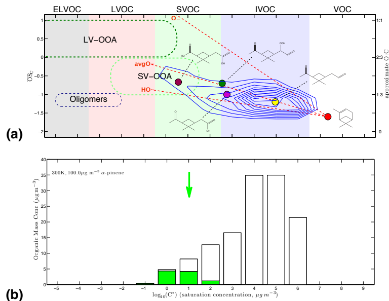
Fig. 3. Products from the ozone + \alpha -pinene reaction in one and two dimensions. (a) The product mass distribution is shown with blue contours. Representative 1st generation products are indicated with colored circles within the contours, along with their molecular structures. \alpha -Pinene is shown with a red circle. The dashed red lines extending from the \alpha -pinene point of origin indicate the trajectories for functionalization in this 2-D space. The middle line is near the value for organic acids and also the average value assumed for 2-D-VBS calculations. (b) A 1-D-VBS product distribution for the same SOA, given by vertical sums over \overline{\text{OS}}_C for each \log_{10}C^* bin. Partitioning is shown for \sim 10 \mu\text{g m}^{-3} of SOA, obtained from oxidation of 100 \mu\text{g m}^{-3} of \alpha -pinene, with condensed-phase OA in green and vapor-phase products in white.
