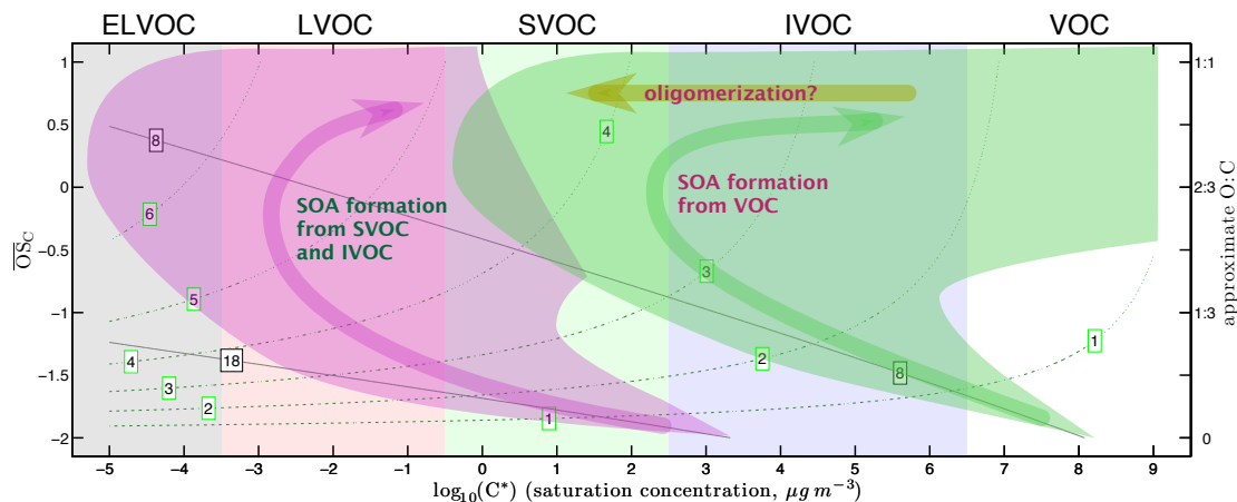
Fig. 7. Two reaction trajectories in 2-D space. SOA formed from VOCs (shown at C_8 ) moves rapidly upward in \overline{OS}_C but reaches a minimum in C^* only barely sufficient to form any SOA in the atmosphere. SOA formed from SVOCs and IVOCs (shown at C_{18} ) moves more slowly upward in \overline{OS}_C but reaches very low C^* values. Both trajectories ultimately result in complete fragmentation (in the limit where the chemistry is allowed to continue to completion), and both consist of a cloud of individual reaction pathways initially centered on the mean carbon isopleth for the parent carbon number. A potential oligomerization trajectory is shown as well.
