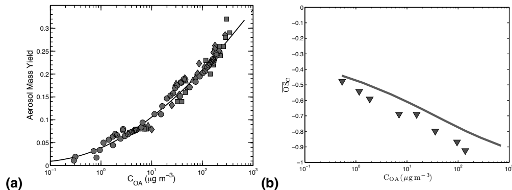
Fig. 2. SOA mass yields (a), (Presto and Donahue, 2006)) and average oxidation state of carbon ( \overline{OS}_C , (b), (Shilling et al., 2009)) from \alpha -pinene + O_3 , both plotted vs. SOA mass ( C_{OA} ). SOA mass yields are used to fit the 1-D-VBS product distribution and \overline{OS}_C the constrains the product oxidation state. Partitioning predictions are shown as curves.
