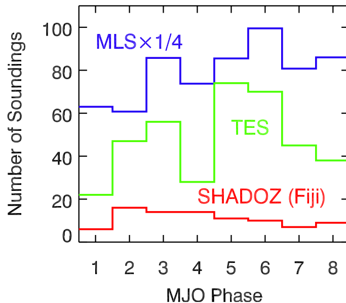
Fig. 8. The number of MLS (blue) and TES (green) swath footprints that fall into the 10^\circ -longitude \times 8^\circ -latitude box centered at Fiji used in this study. The count of MLS has been scaled down by a factor of 4. The number of SHADOZ ozonesonde measurements used in this study is shown in red.
