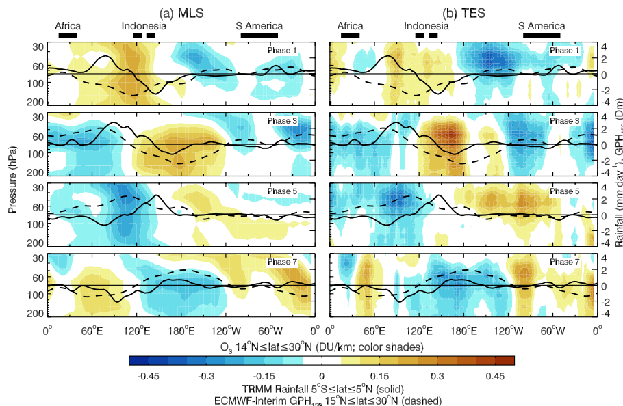
Fig. 6. Pressure-longitude cross sections of the MJO-related O_3 anomalies in the northern subtropics averaged between 14^\circ\text{N} and 30^\circ\text{N} from both MLS (a) and TES (b). A 20^\circ -longitude spatial running average has been applied to remove high-wavenumber fluctuations. Solid lines denote the MJO-related TRMM rainfall anomalies averaged between 5^\circ\text{S} and 5^\circ\text{N} . Dashed lines represent the MJO-related ERA-Interim GPH_{150} anomalies averaged between 15^\circ\text{N} and 30^\circ\text{N} in unit of decameters (1 Dm = 10 m).
