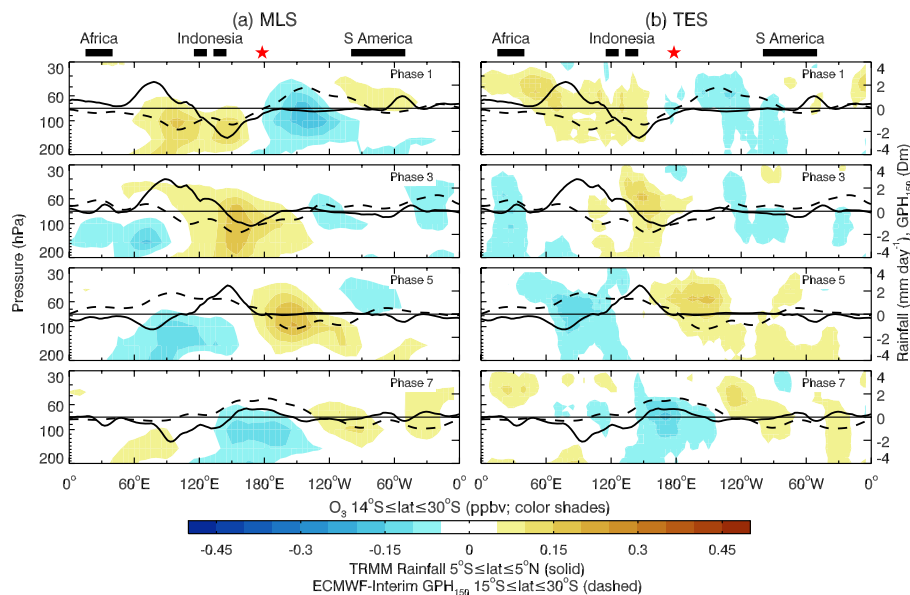
Fig. 7. As in Fig. 6 except for the southern subtropics. The O_3 anomalies (color shades) are averaged between 14^\circ\text{S} and 30^\circ\text{S} ; the GPH_{150} anomalies (dashed) are averaged between 15^\circ\text{S} and 30^\circ\text{S} . The location of Fiji ( 178.4^\circ\text{E} , 18.13^\circ\text{S} ) is denoted by the star (*).
