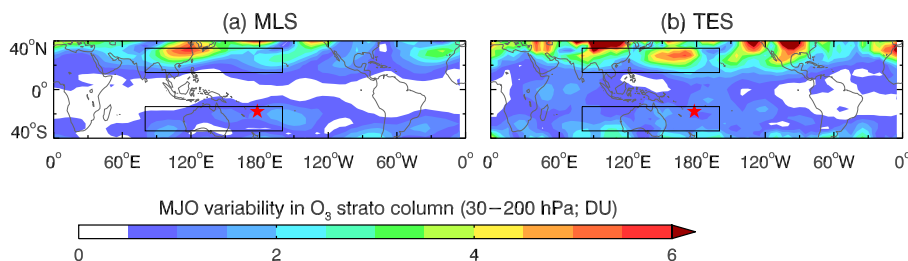
Fig. 4. The MJO variability in O 3 columns derived from MLS and TES observations. The variability is defined as 2 standard deviations of the MJO cycle (see text). The location of Fiji (178.4° E, 18.13° S) is represented by (*). The rectangular boxes enclose representative subtropical regions (80° E–200° E, 14° N/S –34° N/S) where the MJO modulations are largest.
