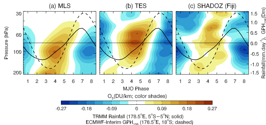
Fig. 9. Vertical structures of the O_3 anomalies over Fiji (178.40° E, 18.13° S) from (a) MLS, (b) TES and (c) SHADOZ as a function of MJO phase for the composite MJO life cycle. The MLS and TES O_3 anomalies are obtained by averaging the swath footprints that fall into the 10°-longitude \times 8°-latitude box centered at Fiji. Solid lines denote MJO-related rainfall anomalies from TRMM averaged between 5° S and 5° N at 178.5° E. Dashed lines represent GPH_{150} anomalies at (178.5° E, 18° S) from ERA-Interim.
