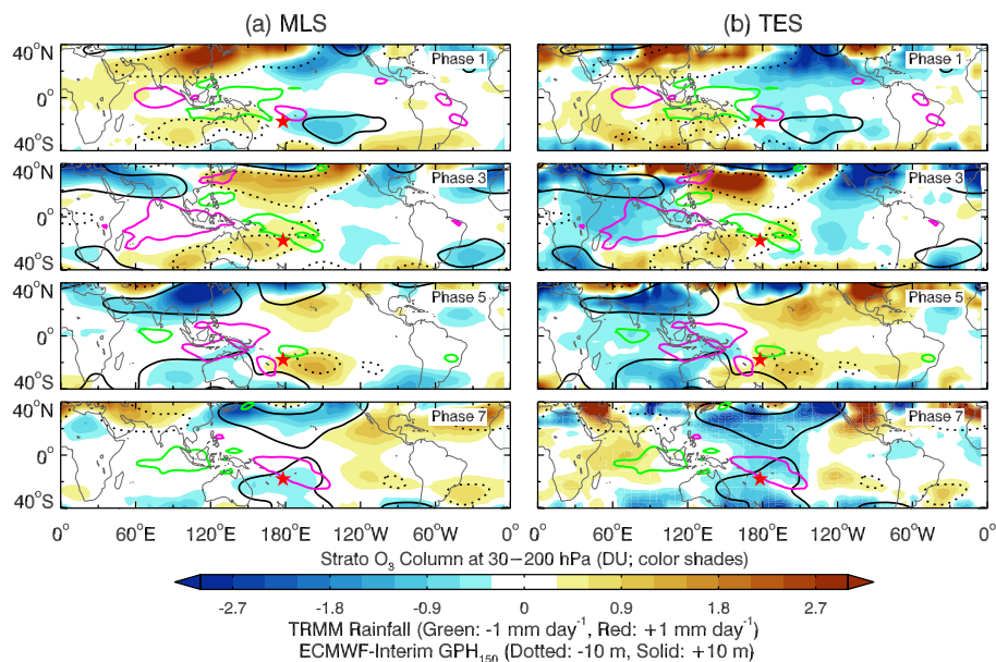
Fig. 3. MJO-related stratospheric \text{O}_3 anomalies integrated between 30–200 hPa in color shades derived from (a) MLS and (b) TES. For simplicity, only MJO phases 1, 3, 5 and 7 are plotted with a 1-2-1 running average applied (see text). Furthermore, a 20^\circ -longitude \times 10^\circ -latitude spatial running average has been applied to remove high wavenumber fluctuations of \text{O}_3 anomalies. The MJO-related rainfall anomalies are overlaid as red ( +1 \text{ mm day}^{-1} ) and green ( -1 \text{ mm day}^{-1} ) solid contours with a 10^\circ -longitude \times 6^\circ -latitude spatial running average applied. The MJO-related 150-hPa geopotential height ( \text{GPH}_{150} ) anomalies are shown as solid ( +10 \text{ m} ) and dotted ( -10 \text{ m} ) black contours with a 9^\circ -longitude \times 6^\circ -latitude spatial running average applied. The location of Fiji ( 178.4^\circ \text{ E} , 18.13^\circ \text{ S} ) is represented by (*).
