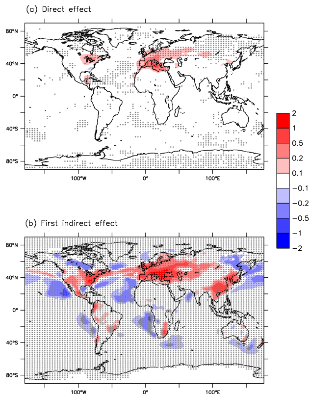
Fig. 16. Difference of radiative forcing between the method using an approximation of the on-line preindustrial concentration and the extended off-line method for the direct effect (a) and between the method using an approximation of the on-line preindustrial concentration and the reference method for the first indirect effect (b) (in \text{W m}^{-2} ). The statistical significance of the difference was tested at the 95 % confidence level using a bootstrap method. Regions where the difference is statistically significant are indicated with dots.
