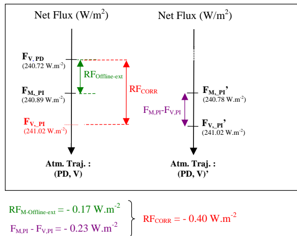
Fig. 13. Schematical representation of the error in the radiative forcing estimation computed from 2 sulphate fields which don't satisfy the criteria of having consistent meteorological fields. Correction with the " F_{M,PI} - F_{V,PI} " term estimated in the Sect. 5.5. The fluxes do not include the impact of direct effect. Only the change due to the first indirect effect is taken into account.
