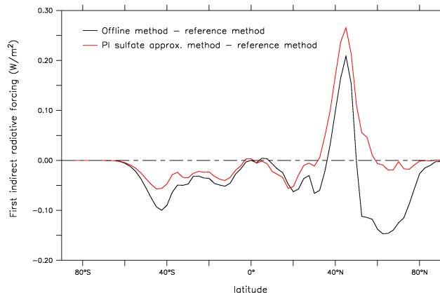
Fig. 17. Zonal mean of the difference of first indirect radiative forcing ( \text{W m}^{-2} ) of the off-line method (black) and the preindustrial sulphate concentration approximation method (red) compared to the reference method.
