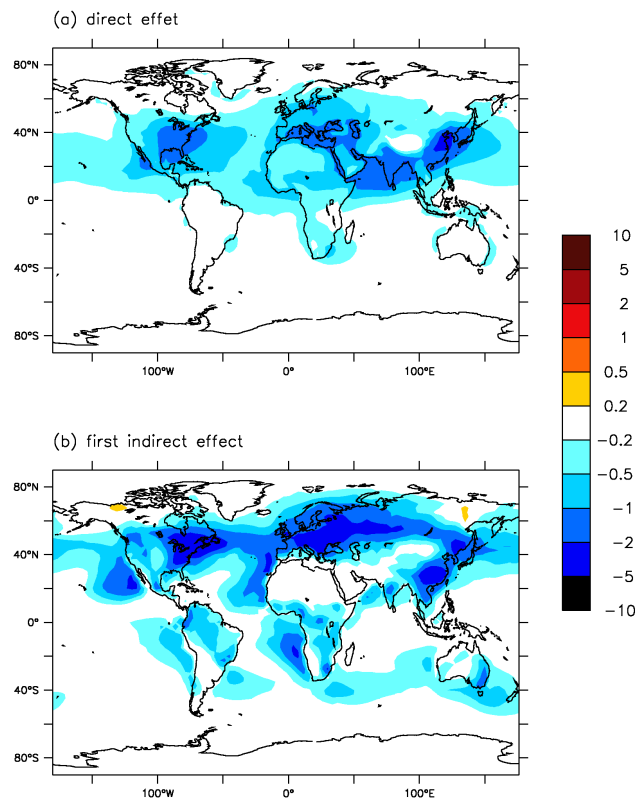
Fig. 4. Radiative forcings ( \text{W m}^{-2} ) estimated with the off-line configuration of the model for present day sulphate emissions: (a) direct effect, (b) 1 indirect effect.
