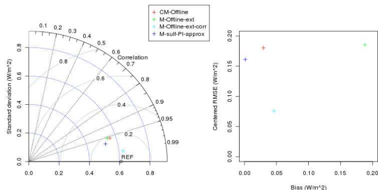
Fig. 18. Comparison of biases on the estimation of the first indirect radiative forcing computed with the four tested methods and relatively to the reference method: off-line method (red), extended off-line method (green); corrected extended off-line method (cyan) preindustrial sulphate concentration approximation method (blue). Taylor diagram (left) presents the performance of methods to represent the spatial pattern of the first indirect effect (including standard deviation, correlation and centered root mean squared error). Right: scatter plot compares the mean bias and the standard deviation of the error for each method.
