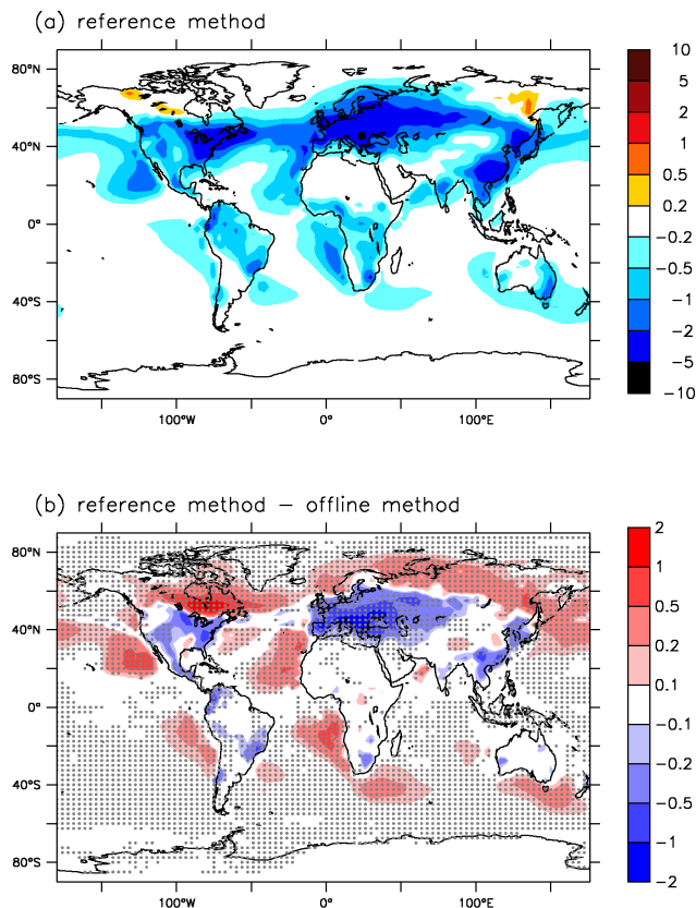
Fig. 11. (a) Reference method ( M_{REF} ) radiative forcing of the first indirect effect ( W m^{-2} ); (b): difference of radiative forcing between the reference method ( M_{REF} ) and the off-line method ( CM_{Offline} ). The statistical significance of the difference was tested at the 95 % confidence level using a bootstrap method. Regions where the difference is statistically significant are indicated with dots.
