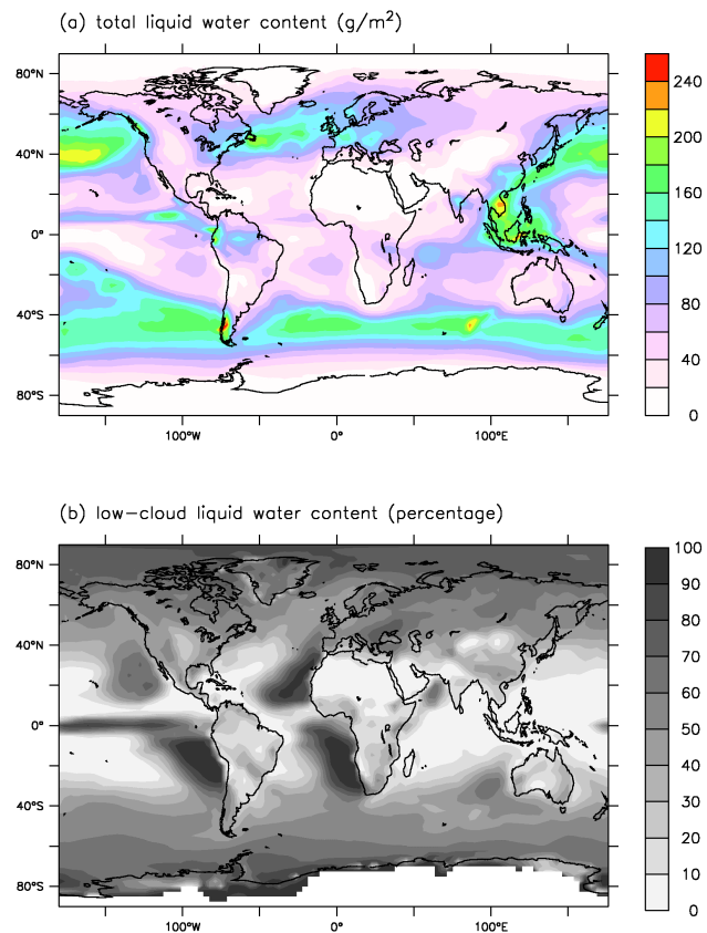
Fig. 7. (a) Cloud liquid water path ( \text{g m}^{-2} ) for all the clouds and (b) percentage of this liquid water path in low level clouds ( P > 850 hPa).
