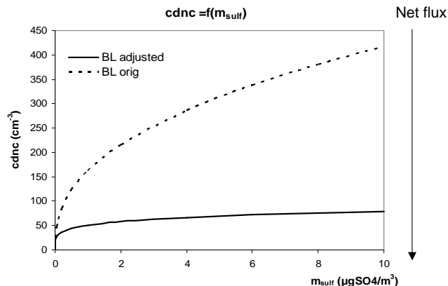
Fig. 1. Relationship between clouds droplet number ( \text{cm}^{-3} ) and the sulphate concentrations ( \mu\text{gSO}_4 \text{m}^{-3} ) from the Boucher and Lohmann 1995 D formula, with the original empirical constant (dashed) and with the adjusted empirical constant of Quaas et al., 2005 (solid line).
