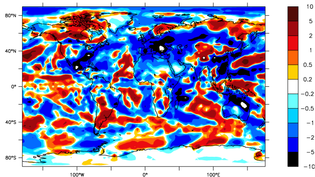
Fig. 3. Difference between the short wave top-of-atmosphere net fluxes (in \text{W m}^{-2} ) computed with present day and with preindustrial sulphate emissions. The on-line configuration of the model is used.
