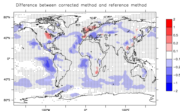
Fig. 14. Difference of the radiative forcing of the first indirect effect calculated from the extended off-line method corrected with the \Delta NF_{PI} term and that one calculated in the reference method (experiment VAR) in W m^{-2} . The statistical significance of the difference was tested at the 95 % confidence level using a bootstrap method. Regions where the difference is statistically significant are indicated with dots. Color bar of the first map varies from -10 and +10 W m^{-2} whereas values of the second map (difference) vary from -2 and +2 W m^{-2} .
