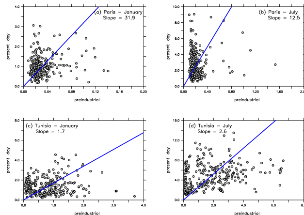
Fig. 15. Correlation between the present-day sulphate concentration and the preindustrial one for 2 grid points (Paris and Tunisia) and 2 months (January and July). The blue line represents the expected values of the actual by preindustrial instantaneous ratio considering it is the same that the ratio of monthly mean concentrations. Slopes indicate the values of the monthly mean ratio.
