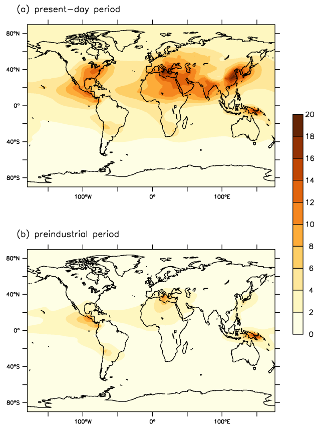
Fig. 8. Annual mean of the sulphate load ( \text{mg}(\text{SO}_4)\text{m}^{-2} ) for present day (a) and preindustrial periods (b) .
