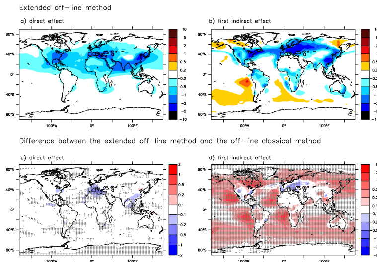
Fig. 10. Radiative forcing calculated from the extended off-line method for: (a) sulphate direct effect ( \text{W m}^{-2} ), (b) sulphate first indirect effect ( \text{W m}^{-2} ). Difference of radiative forcings between the off-line extended method and the off-line method: (c) sulphate direct effect ( \text{W m}^{-2} ), (d) sulphate first indirect effect ( \text{W m}^{-2} ). The statistical significance of the difference was tested at the 95 % confidence level using a bootstrap method. Regions where the difference is statistically significant are indicated with dots. The scales of the top row maps is in the range (-10; +10 \text{ W m}^{-2}) whereas the values for the bottom row maps (that represent differences in radiative forcings) vary between (-2; +2) or (-5; +5) \text{ W m}^{-2} .
