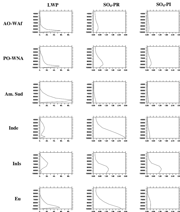
Fig. 9. Annual mean vertical profile of the cloud liquid water content ( \text{mg m}^{-3} ), and of the sulphate content (in \mu\text{g}(\text{SO}_4) \text{m}^{-3} ) for present day ( \text{SO}_4\text{-PR} ) and preindustrial emissions ( \text{SO}_4\text{-PI} ). 6 regions are considered: (1) South Atlantic Ocean along the West Coast of Africa (referred as AO-WAf), (2) North Pacific Ocean along the West Coast of North America (referred as PO-WNA); (3) the southern part of South America (South Am.); (4) India (India); (5) Indonesia Islands (InIs); (6) Europe (Eu).
