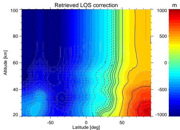
Fig. 1. Average differences between retrieved and engineering tangent altitudes during December–February of 2007–2009.
