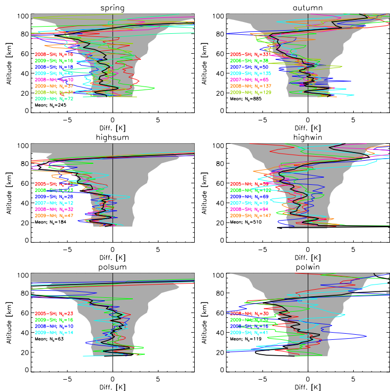
Fig. 10. Average temperature differences of co-located measurements of MIPAS v511 minus ACE-FTS v2.2 measurements for spring and autumn (upper row), high latitudes ( 50^{\circ} – 70^{\circ} ) summer and winter (middle row) and polar ( 70^{\circ} – 90^{\circ} ) summer and winter (bottom row). The differences averaged for the different years and hemispheres (for which the number of co-located measurements are also indicated) are shown in color. Average difference for each period and latitude box is shown in black. The shadowed area is MIPAS and ACE-FTS combined error.
