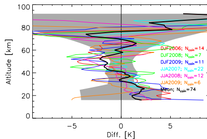
Fig. 16a. Mean temperature differences of solstice MIPAS v511 and Table Mountain Facility lidar ( 34^\circ N, 118^\circ W) co-located measurements (the seasons, years and number of coincidences are indicated in color). The total number of co-locations is 74. Average difference is shown in black. The shadowed area is the combined error.
