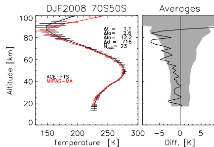
Fig. 9. Average of MIPAS v511 (red) and ACE-FTS v2.2 (black) co-located temperature profiles (left) and their difference (MIPAS–ACE; right) for Southern Hemisphere summer ( 50^{\circ}\text{S} – 70^{\circ}\text{S} ) in 2008. Horizontal bars are their standard deviation. Average differences in time in hours, latitude and longitude in degrees, distance in kilometers, and number of averaged profiles for each instrument are also shown. The shadowed area in the right panel is the combined error.
