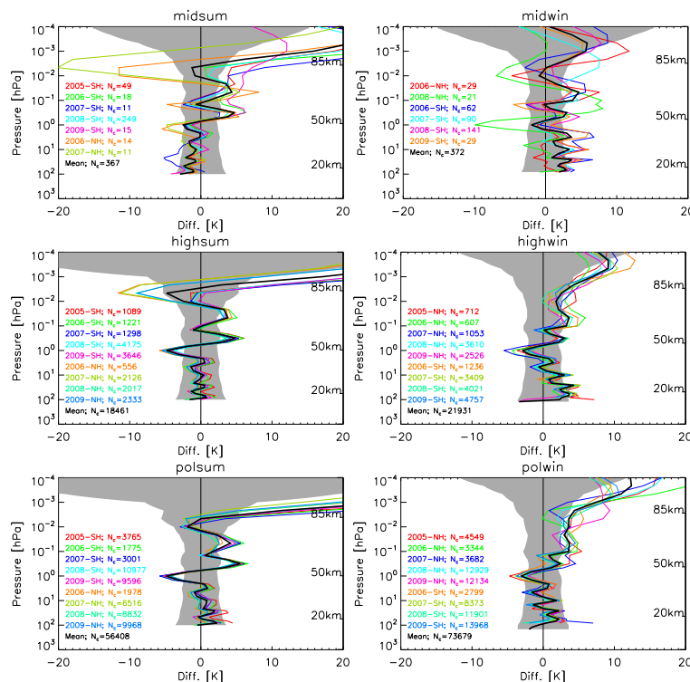
Fig. 12. Average temperature differences of solstice (left: summer; right: solstice) co-located measurements of MIPAS v511 minus MLS v2.2 measurements for mid-latitudes (30°–50°; upper row), high latitudes (50°–70°; middle row) and polar (70°–90°; bottom row). Differences averaged for the different years and hemispheres (for which the number of co-located measurements are indicated) are shown in color and average difference for each period and latitude is shown in black. The shadowed area is the combined error. The corresponding mean MIPAS approximate altitude is shown in the vertical right axis.
