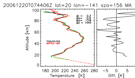
Fig. 13. Example of a comparison on December 2006 of individual nighttime profiles of temperature (left) and their difference (MIPAS–lidar; right) measured by MIPAS v511 (red – dashed line correspond to an extended profile with ECMWF values) and the lidar at the Mauna Loa Observatory (20° N, 156° W) (black: convolved with MIPAS averaging kernels; green: not-convolved). The horizontal bars are the noise errors. Differences between both measurements in time in hours, latitude and longitude in degrees and distance in kilometers are also shown. Note MIPAS ability to reproduce vertical structures shown in the lidar measurements.
