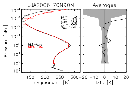
Fig. 11. Average of 1978 temperature profiles of MIPAS v511 (red) and MLS v2.2 (black) co-located measurements (left) and their difference (MIPAS–MLS; right) for Northern Hemisphere polar summer (70° N–90° N) in 2006. MIPAS profiles have been convolved to meet MLS vertical resolution. Horizontal bars are the average profiles standard deviation. Average differences in time of measurements in hours, latitude and longitude in degrees, and distance in kilometers are also shown. The shadowed area in the right panel is the MLS and MIPAS combined systematic error.
