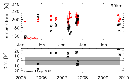
Fig. 18. Nightly mean MIPAS v511 temperature at 95 km (red) and SATI O 2 rotational temperatures (37° N, 3° W) (black) and their standard deviation (vertical bars from 2005 to 2009 (top panel) and their difference (MIPAS–SATI). The shadowed area is MIPAS systematic error. The mean difference and its error are also indicated.
