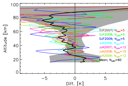
Fig. 14a. Mean temperature differences (MIPAS–lidar) of solstice co-located measurements of MIPAS v511 and Mauna Loa Observatory lidar ( 20^{\circ} N, 156^{\circ} W) (the seasons, years and number of coincidences are indicated in color). Average difference is shown in black. The total number of co-locations is 60. The shadowed area is the combined systematic error.
