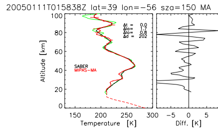
Fig. 4. Left: example of a comparison of an individual MIPAS v511 temperature profile at 39^\circ N and 56^\circ W in January 2005 (solid red) with a co-located SABER v1.07 measurement (green) and its corresponding smoothed profile using MIPAS averaging kernels and a priori profile as in Eq. (5) (black). The differences in time in hours ( \Delta t ), latitude ( \Delta la ) and longitude ( \Delta lo ) in degrees, and distance ( \Delta d ) in kilometers between the two measurements are also shown. Red horizontal bars are the MIPAS noise errors. The dashed red line shows the extension of the MIPAS profile with the corresponding ECMWF profile. Right: difference between MIPAS and SABER convolved temperatures (MIPAS–SABER).
