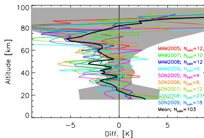
Fig. 14b. As in Fig. 14a but for comparisons over MLO during equinox. The total number of co-locations is 103.
