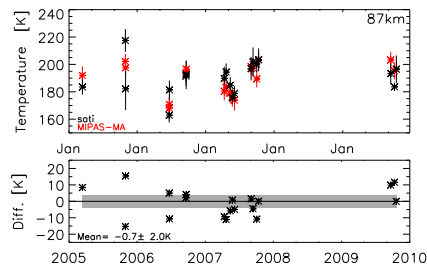
Fig. 17. Nightly mean MIPAS v511 temperature at 87 km (red) and SATI OH rotational temperatures ( 37^\circ N, 3^\circ W) (black) and their standard deviation (vertical bars) from 2005 to 2009 (top panel) and their difference (MIPAS–SATI). The shadowed area is MIPAS systematic error. The mean difference and its error are also indicated.
