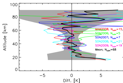
Fig. 16b. As in Fig. 16a but for comparisons over TMF during equinox. The total number of co-locations is 68.
