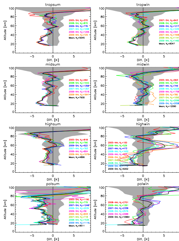
Fig. 6. Mean temperature differences of solstice (left column: summer; right column: winter) co-located measurements of MIPAS v511 minus SABER v1.07 measurements for the tropics (10°–30°; 1st row), mid-latitudes (30°–50°; 2nd row), high latitudes (50°–70°; 3rd row) and the poles (70°–90°; 4th row). The differences averaged for the different years and hemispheres (for which the number of co-located measurements are also indicated) are shown in color. Average difference is shown in black. The shadowed area is the MIPAS and SABER combined systematic error.
