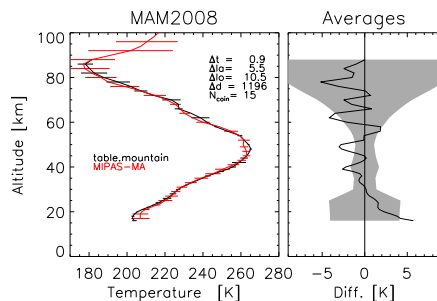
Fig. 15. Mean of co-located profiles of MIPAS v511 and Table Mountain Facility lidar ( 34^{\circ} N, 118^{\circ} W) temperatures (left) and their difference (MIPAS–lidar; right) for the spring in 2008 (March, April and May). The total number of averaged profiles is 15. Horizontal bars are their standard deviation. Average differences in time in hours, latitude and longitude in degrees and distance in kilometers are also shown. The shadowed area in the right panel is the combined systematic error.
