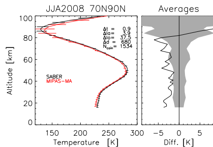
Fig. 7. As in Fig. 5 but for the north pole (70° N–90° N). This figure shows the typical behavior over the polar summer, where MIPAS is slightly colder and shows similar gradients up to 80 km and warmer above. MIPAS stratopause and mesopause is located slightly below SABER's.
