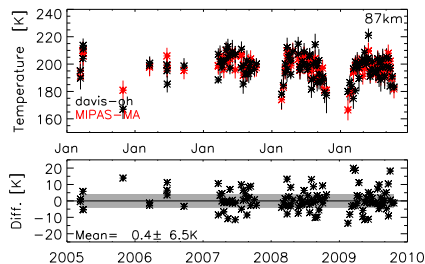
Fig. 19. Nightly mean MIPAS v511 temperature at 87 km (red) and Davis OH rotational temperatures ( 69^\circ S, 78^\circ E) (black) and their standard deviation (vertical bars) from 2005 to 2009 (top panel) and their difference (MIPAS – DS; bottom panel). The shadowed area is the combined error.
