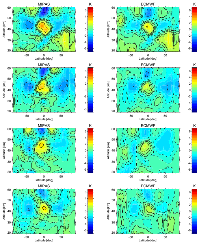
Fig. 3. Seasonal averages of zonal mean temperature differences between descending (10 a.m.) and ascending (10 p.m.) orbit branch observations of MIPAS (left) and ECMWF sampled at the corresponding MIPAS locations. Top to bottom: December–February (DJF), March–May (MAM), June–August (JJA), and September–November (SON).
