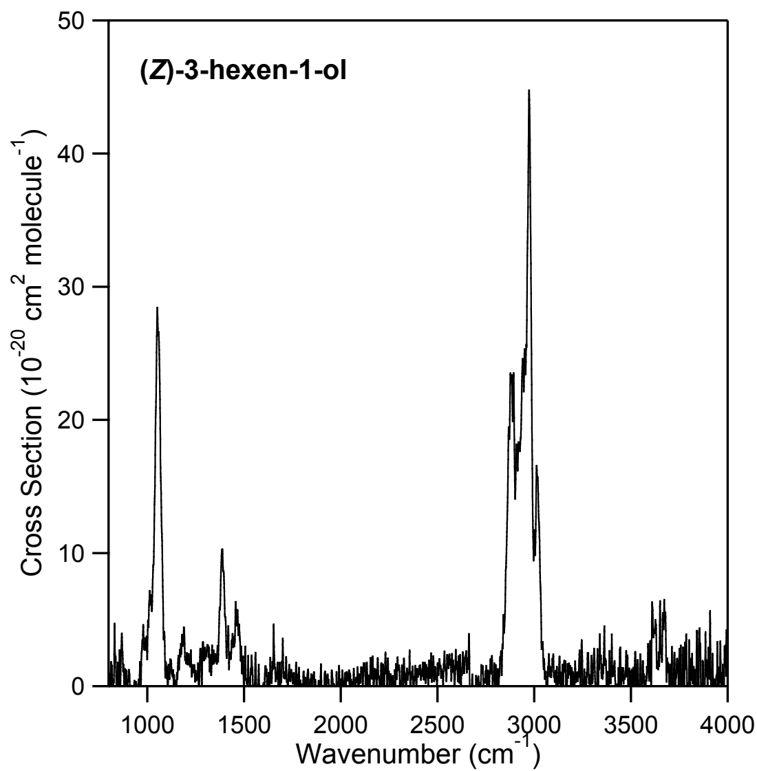
Figure S1. Infrared absorption spectra of C5 and C6 unsaturated alcohols measured in this work.
