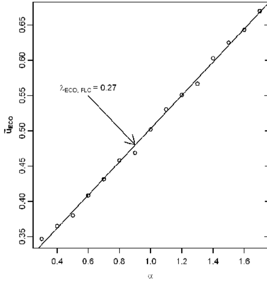
Figure S2. Determination of \bar{u}_{ECO} sensitivity to u_{FLC} for \Delta x = 200 km and \Delta t = 30 day.
