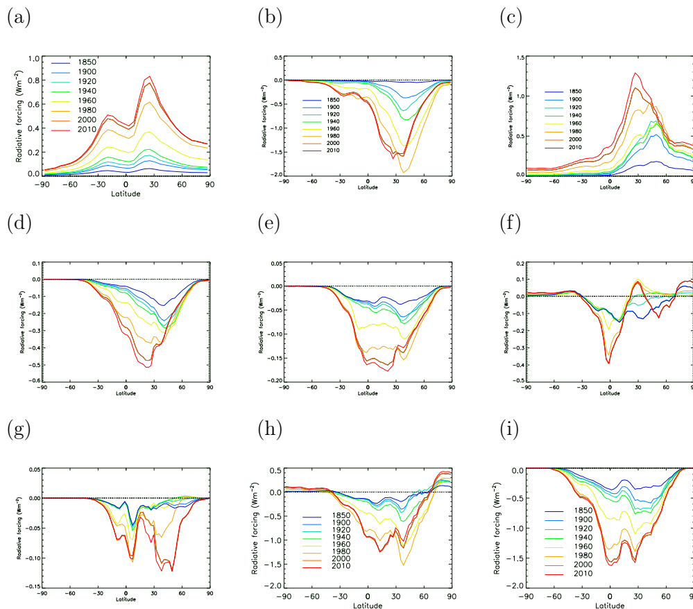
Fig. 3. Zonal mean RF for selected years for tropospheric ozone (a) , direct aerosol effect of sulphate (b) , FFBF BC (c) , FFBF OC (d) , SOA (e) , BB aerosols (f) , nitrate (g) , total direct aerosol effect (h) and the cloud albedo effect (i) .
