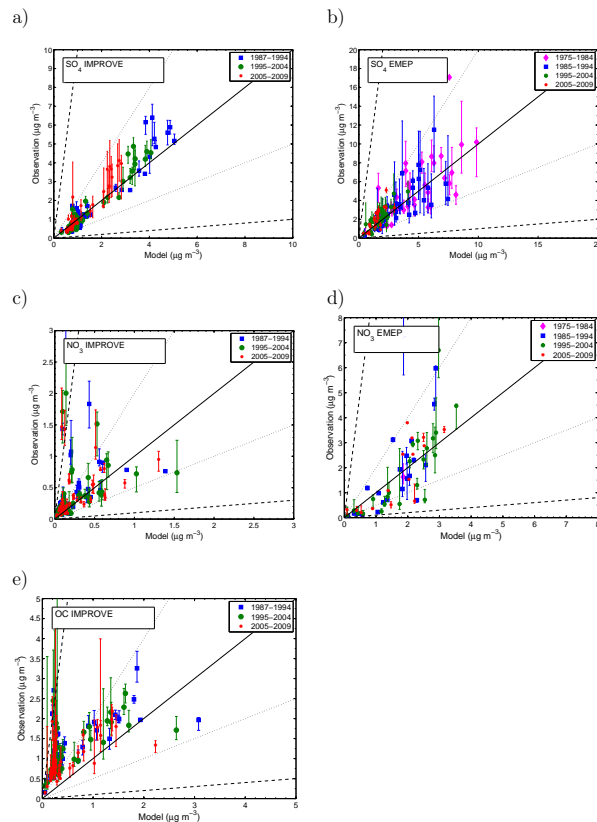
Fig. 10. The median of the observed annual means from the IMPROVE and EMEP networks compared with the corresponding modelled annual means for sulphate ( a , b ), nitrate ( c , d ) and OC ( e ) for each decade. The solid line shows a one-to-one correspondence. The dotted lines show a factor of 2 difference and the dashed lines a factor 10 difference between the observations and model results. The error bars added to the observations denote the maximum and minimum of the annual means in the decade.
