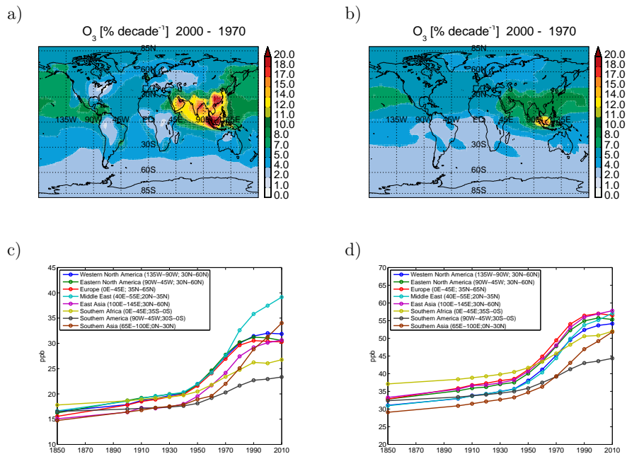
Fig. 6. Relative change (% decade -1 ) in surface O_3 (a) and at approximately 500 hPa (b) between 1970 and 2000. Time evolution of regional mean O_3 at the surface (c) and approximately 500 hPa (d).
