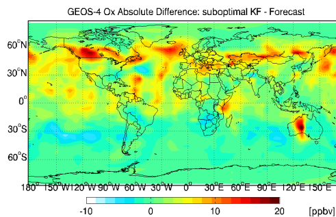
(b) Absolute difference between suboptimal Kalman filter analysis and the free model run
