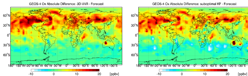
(a) Absolute difference between 3D-Var analysis and the free model run (b) Absolute difference between suboptimal Kalman filter analysis and the free model run
