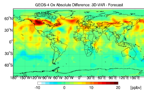
(a) Absolute difference between 3D-Var analysis and the free model run
