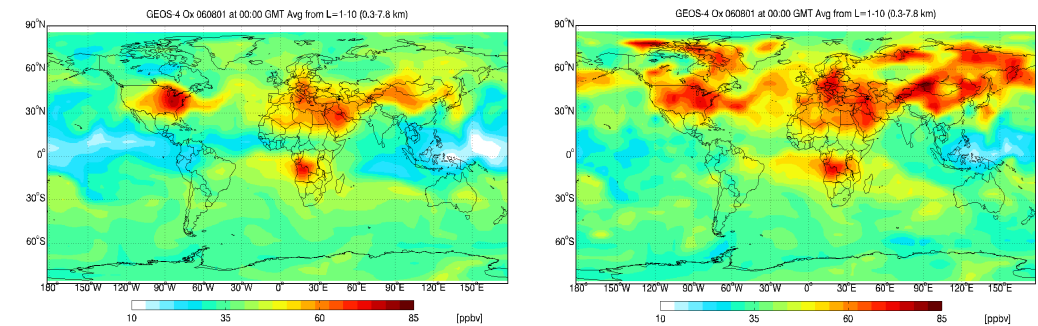
(a) Free model ozone concentration at the beginning of the assimilation window (b) 4D-Var ozone analysis at the beginning of the assimilation window
