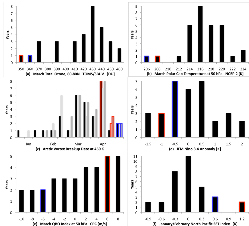
Fig. 1. Histograms of total ozone and dynamical conditions during the 1979–2011 period: (a) March total ozone averaged between 60–80° N [DU]; (b) March Arctic polar cap temperature at 50 hPa [K]; (c) date of the Arctic vortex breakup at 450 K based on the NCEP-2 (black), NCEP-1 (light gray) and CPC (dark gray) reanalyses, binned into 10-day intervals; (d) January–February–March SST anomaly in the Niño 3.4 region [K]; (e) March zonal winds in the equatorial region at 50 hPa [ \text{m s}^{-1} ]; (f) January/February SST anomaly in the 40–50° N, 160–200° E region [K]. Red (blue) outlines indicate the location of 2011 (1997) conditions. Y-axis values indicate the mid-point of each histogram bin.
