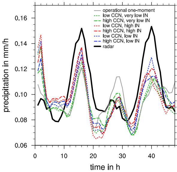
Fig. 5. As Fig. 7 of the main text. Time series of hourly rain rate averaged over the (a) the northern evaluation domain, and (b) the central evaluation domain. Shown are the radar data, the six two-moment microphysics experiments, and the control simulation using the operational one-moment scheme (all simulations initialized at 00 UTC).
