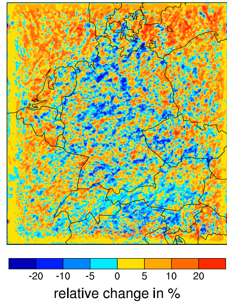
Fig. 2. Relative difference in % of the monthly mean accumulated precipitation of JJA 2008-2010 comparing different experiments. Shown is the full model domain in the original rotated lat-lon coordinates including the nudging zone at the lateral boundaries.
