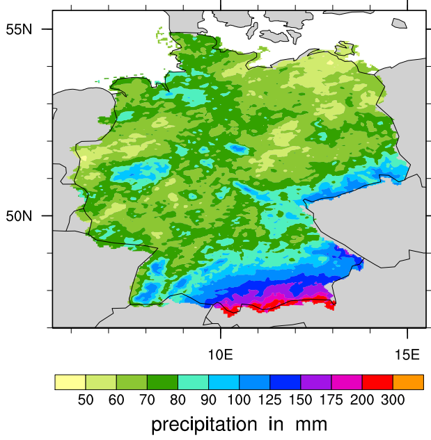
a) Experiment 5: high CCN, very low IN
