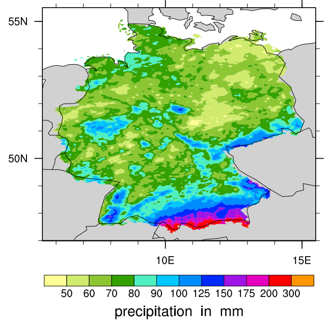
b) Experiment 6: low CCN, very low IN
