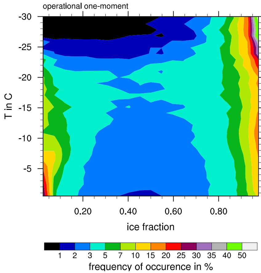
Fig. 7. As Fig. 6 of the main text, but for the operational one-moment microphysics scheme (Exp. 7).
