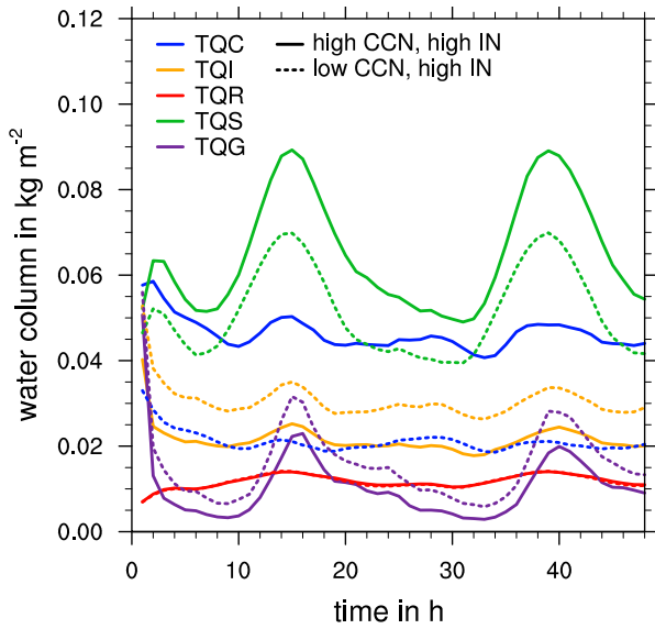
Fig. 4. As Fig. 3 of the main text, but comparing the CCN at high IN (left), and IN perturbation experiments at low CCN (right).
