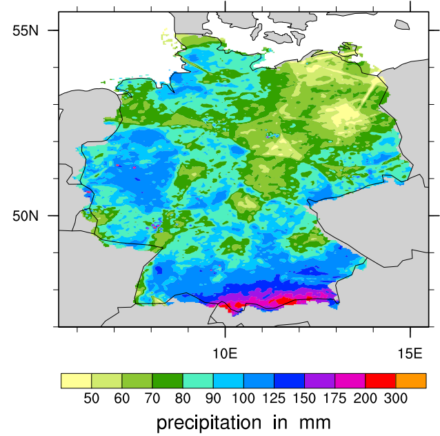
Fig. 1. Monthly mean precipitation amount of JJA 2008, 2009 and 2010. Shown are experiment 5, 6, and 7 as well as the radar product.
