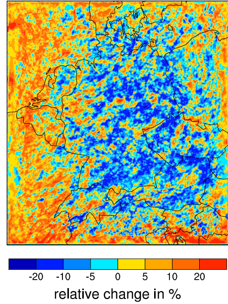
d) Sensitivity to IN (high-low) at low CCN (Exp 4 - Exp 2)
