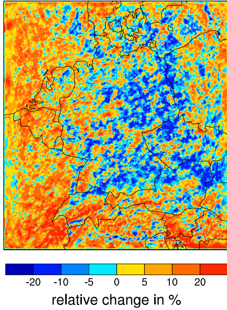
c) Sensitivity to IN (high-low) at high CCN (Exp 3 - Exp 1)
