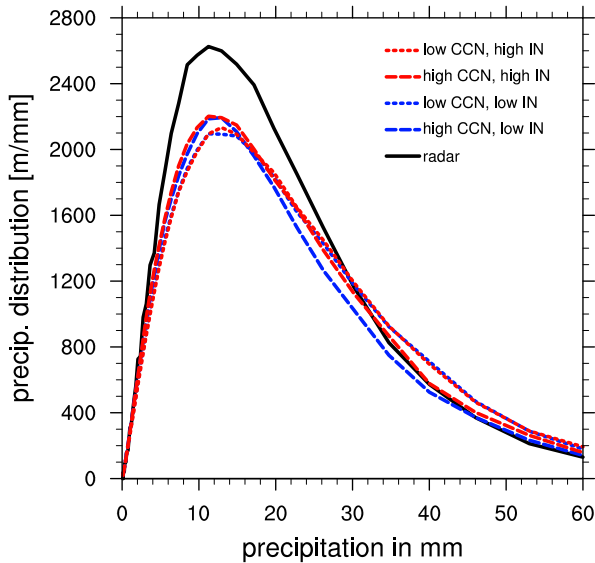
Fig. 3. Precipitation distribution function P(R) = N(R)R p(R) , where R is a 12-h accumulated grid-scale precipitation amount, p(R) is the probability density function of R , and N(R) is the number of events.
