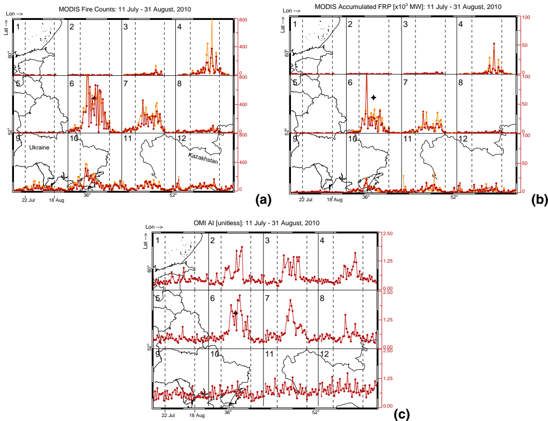
Fig. 4. Time series of fire products, smoke tracers and aerosol properties plotted within 12 geographic domains. The time period shown is from 11 July to 31 August 2010. The latitude and longitude limits of each domain are defined in Table 1. Time series of MODIS fire counts and FRP ( a and b ) are daily sums within each domain. Time series of OMI AI and SSA, MODIS AOT 55 and AIRS CO TC ( c–f ) are area averages. The dashed vertical lines within each domain mark the active fire period between 22 July and 18 August. The solid black star in domain 6 indicates Moscow. In ( a ), ( b ), and ( e ) Aqua-MODIS data are red, and Terra-MODIS in orange.
