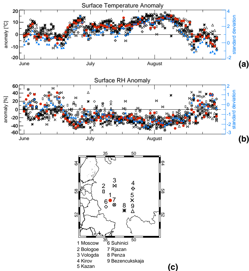
Fig. 1. (a) T_{\text{sfc}} and (b) \text{RH}_{\text{sfc}} anomalies (2010 – (1994–2009 mean)) calculated from radiosonde measurements at nine stations in western Russia. Radiosonde locations, including symbol legend for (a) and (b) are mapped in (c). The red dots highlight data from the Moscow site. Blue triangles show the daily standard deviation of the anomalies using the mean of all station anomalies. The zero line pertains to the anomaly y-axis.
