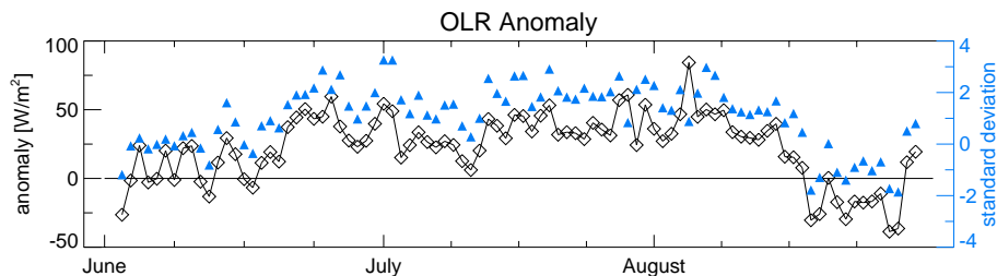
Fig. 2. AIRS OLR daily anomalies ((2010 – (2003–2009 mean)) (black diamonds) and the number of standard deviations (blue triangles) averaged over [33° E–53° E, 52° N–62° N]. The location of the radiosonde stations plotted in Fig. 1c is within this domain.
