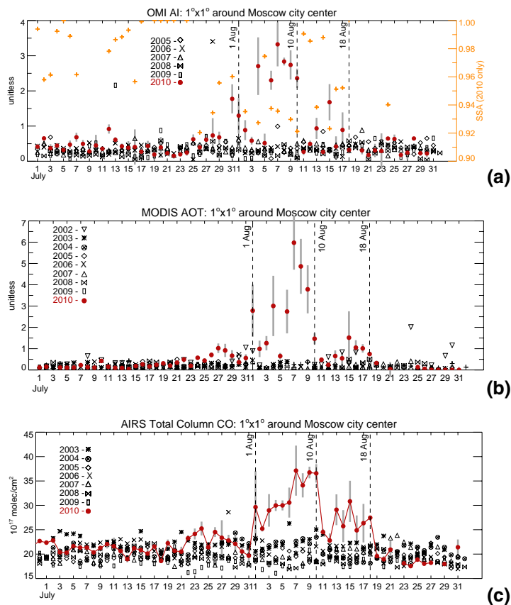
Fig. 7. (a) Daily OMI AI and SSA (2010 only) per year over Moscow between July and August. The 1-sigma standard deviation of SSA is within the uncertainty ( \pm 0.03 ). (b) Daily MODIS AOT 55 and (c) AIRS CO TC plotted similar to (a). AOT 55 are the average of Aqua and Terra MODIS values. The 1- \sigma standard deviations are plotted for 2010 only in grey shading.
