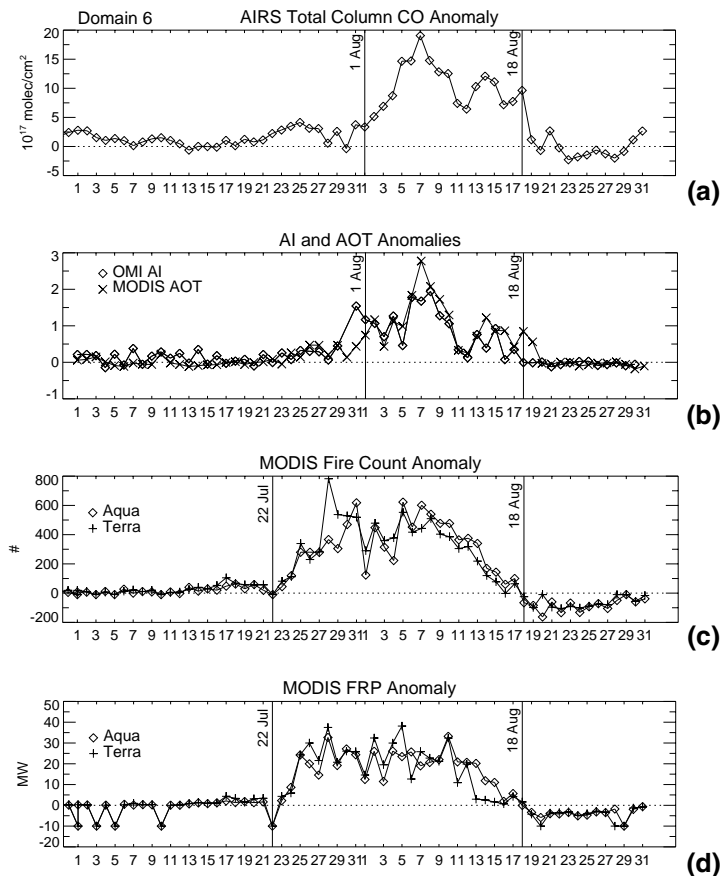
Fig. 5. July and August 2010 anomalies of (a) AIRS \text{CO}_{\text{TC}} , (b) OMI AI and MODIS \text{AOT}_{.55} , (c) MODIS fire counts, and (d) MODIS FRP over domain 6 (52–58° N, 33–43° E). Anomalies for each constituent were calculated by subtracting the 2010 daily values from the daily mean of all previous years. MODIS \text{AOT}_{.55} anomalies in (b) are calculated using the mean of Aqua and Terra.
