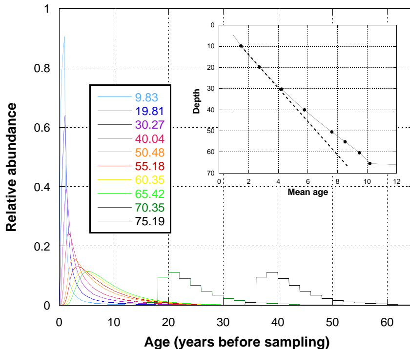
Fig. 8. Normalized age distributions for CO 2 in firn air at selected depths (given in the legend) from the moving-coordinate firn model (see text). The step-like structure within the lockin zone is a result of model discretization and does not reflect any underlying physics. The inset shows the mean age as a function of depth, with points indicating the means for the particular distributions selected for the main plot. The dashed line is included only to highlight the departure from linearity.
