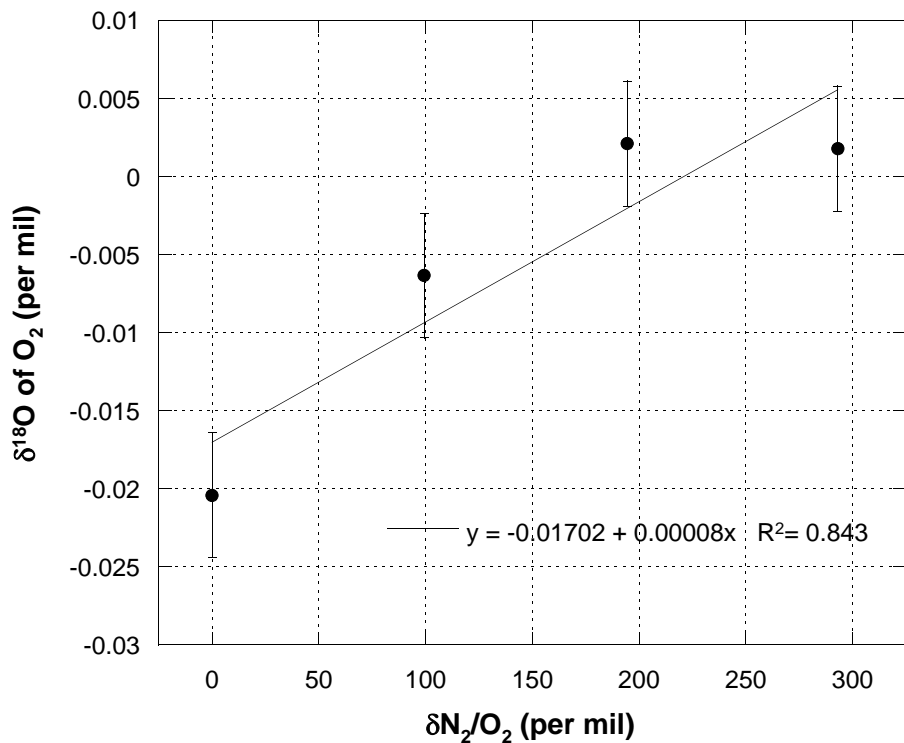
Fig. 9. Results of the “chemical slope” experiment used for correcting oxygen isotope data. Pure commercially-obtained N_2 was added to aliquots of an air standard. Note that N_2 is in the numerator in this plot. The resulting corrections applied to the data were 0.0006 or less.
