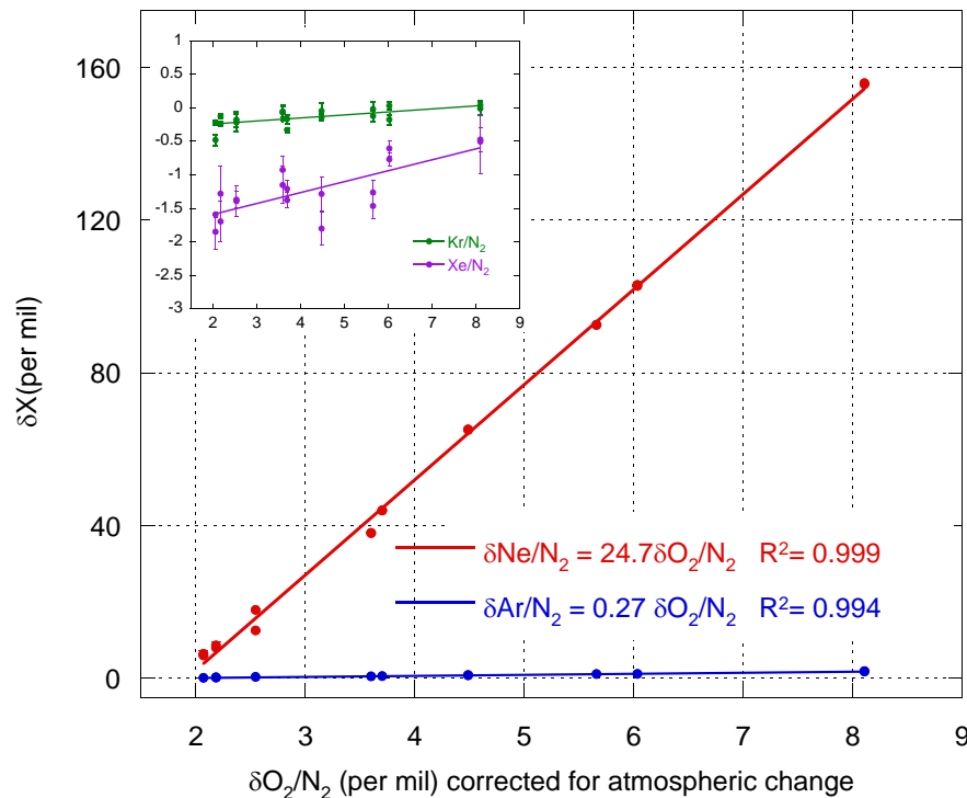
Fig. 4. Ratios of noble gases to N 2 from the lock-in zone. Errors shown are 1 \sigma , derived from the pooled standard deviation of replicate flasks and are generally smaller than the points for Ar/N 2 , Ne/N 2 and O 2 /N 2 . Note however that the model-based correction for atmospheric changes in O 2 introduces additional uncertainty that we have not shown in the plot (see text).
