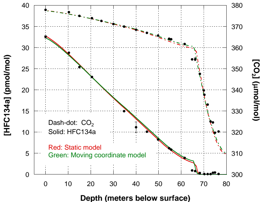
Fig. 3. Output of two different versions of the firn model: the static formulation and the moving-coordinate formulation. Both models were run with the same diffusivity-depth profiles. Two species with very different atmospheric histories (Montzka et al., 1996; Etheridge et al., 1998; Conway et al., 2010) were chosen for illustrative purposes. Also shown are our measurements of the firn air, with error bars. The error bars are based on the pair-wise agreement of replicate flasks collected at each depth, and are usually smaller than the markers on the plot.
