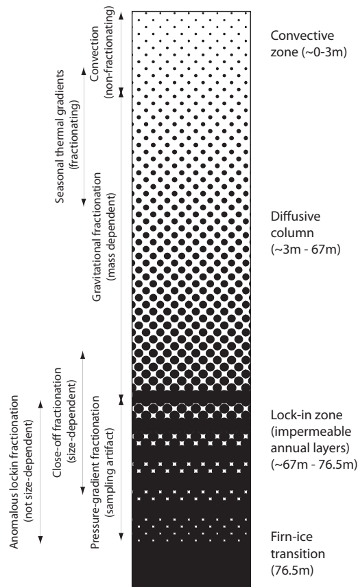
Fig. 1. A schematic diagram of regions in an idealized firn column, showing generic features (on the right) and the transport mechanisms expected to be significant in each region (on the left). Also shown (in parentheses on the right) are the approximate depths of the features at WAIS-D. The figure is not drawn to scale, and not all processes will be present in every naturally occurring firn column.
