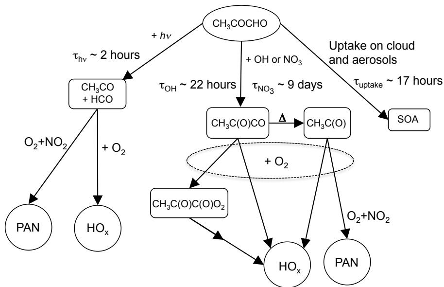
Fig. 1. Simplified atmospheric degradation scheme for methylglyoxal highlighting loss via UV photolysis, OH radical reaction, \text{NO}_3 radical reaction, and cloud and aerosol uptake. Approximate atmospheric lifetimes are included (see text for details).
