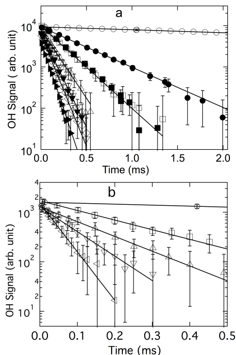
Fig. 2. Representative OH temporal profiles obtained at 295K using \text{H}_2\text{O}_2 photolysis at 248nm (a) and at 211K using tert -butyl hydroperoxide (b) as the OH radical sources. [\text{CH}_3\text{COCHO}] ( 10^{14} molecule \text{cm}^{-3} ); open symbols: [\text{O}_2]=0.0 ; filled symbols: [\text{O}_2]=5.4 \times 10^{16} molecule \text{cm}^{-3} ; (a) : 0.0 ( \circ ), 1.64 ( \bullet ), 3.32 ( \blacksquare , \square ), 5.81 ( \triangle ), 7.91 ( \nabla , \blacktriangledown ), 9.25 ( \diamond ), 11.54 ( \blacktriangleright ); (b) : 0.0 ( \circ ), 1.23 ( \square ), 2.15 ( \triangle ), 3.66 ( \nabla ), 7.78 ( \blacktriangleleft ). Lines in (a) and (b) are fits of the data to Eq. (I). The OH profiles shown in the upper panel have been offset for clarity.
