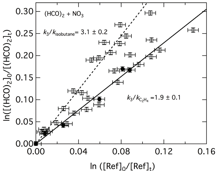
Fig. 6. Relative rate data for the \text{NO}_3 + (\text{HCO})_2 (glyoxal) reaction at 296 K and 650 Torr (Syn. Air) with \text{C}_2\text{H}_4 and iso-butane as the reference compounds. The solid symbols represent the data obtained in the presence of 1.7 \times 10^{16} molecules \text{cm}^{-3} of \text{CF}_3\text{CF}=\text{CHF} . The lines are linear least-squares fits of the data to Eq. (III), where the uncertainty is 2\sigma of the fit precision.
